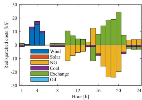
Fig. 7. Hourly total re-dispatching costs per fuel.
