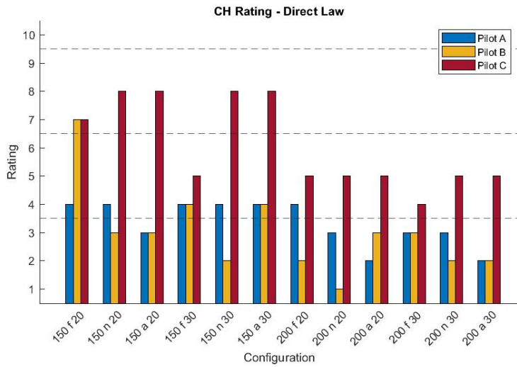
Fig. 15 Handling Qualities Rating – Direct Law.
