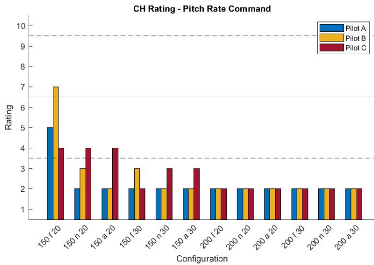
Fig. 16 Handling Qualities Rating – Pitch Rate Command.
