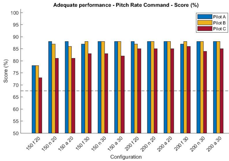
Fig. 12 Adequate performance score – Pitch Rate Command.
