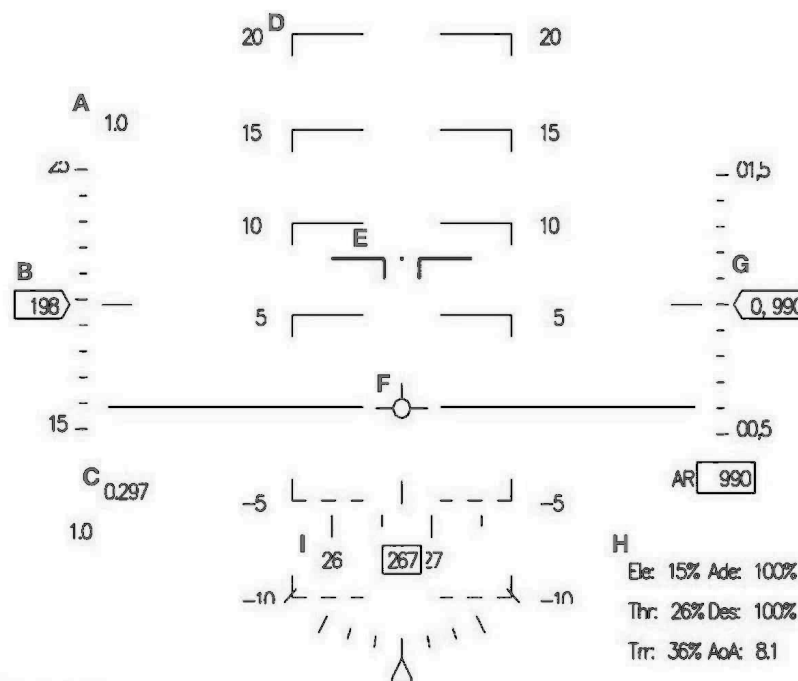
Fig. 7 Arrangement of information in the MIP.
