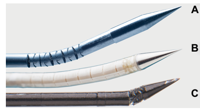
Figure 2 Examples of steerable needle prototypes.
