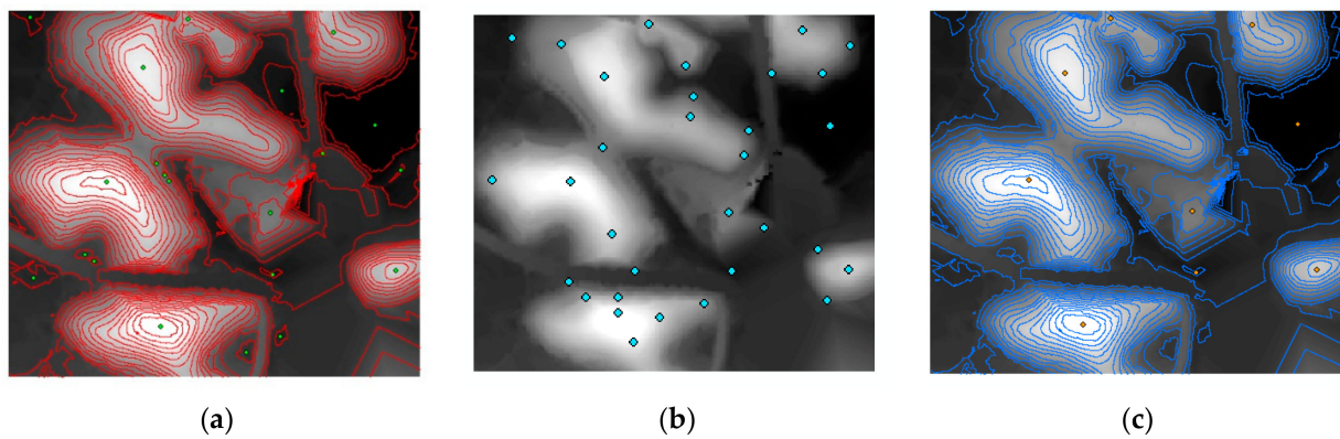
Figure 10. The experimental first dataset distribution map extracted using traditional mountain vertex extraction methods: (a) Contour Line Method; (b) Neighborhood Analysis Method; and (c) Contour line and Neighborhood Analysis Overlay Method.
