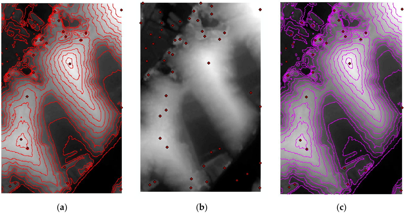
Figure 22. Distribution maps extracted by the traditional Mountain Vertices Extraction Methods using the fourth dataset. (a) Contour Line Method. (b) Neighborhood Analysis Method. (c) Contour line and Neighborhood Analysis Overlay Method.
