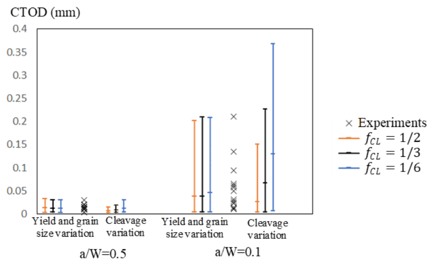
Fig 4. 18 Cleavage prediction of various f_{CL} = \frac{V_{CL}}{V_{CL} + V_{OutCL}}
