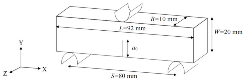
Fig 3. 12 Geometry information of the SENB specimen (Z direction coincides to ND of the plate)
