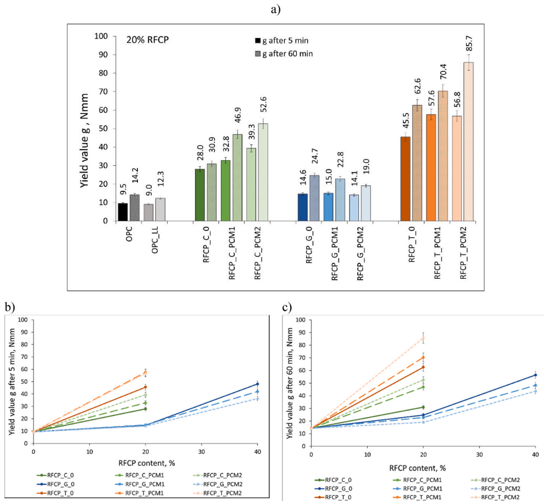
Fig. 11. Influence of type (a) and content of RFPC on yield stress (g) of fresh mortars with w/b = 0.65 after 5 min (b) and 60 min (c).
