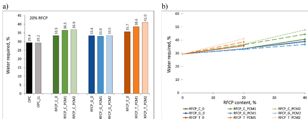
Fig. 5. Influence of type (a) and content of RFPC (b) on water required for standard consistency of cement pastes.
