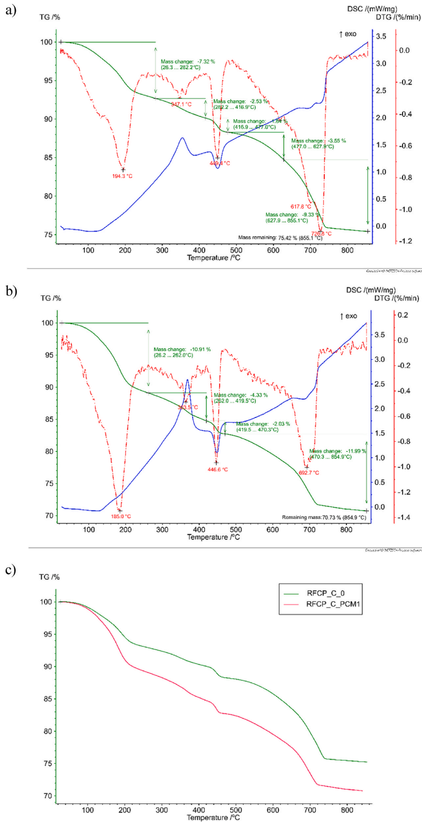
Fig. 3. Thermal analysis of the RFCP: a) RFCP_C_0 (without MPCM), b) RFCP_C_PCM1 (with MPCM Nextek 24D), c) TGA curve comparison of RFCP_C_0 and RFCP_C_PCM1.
