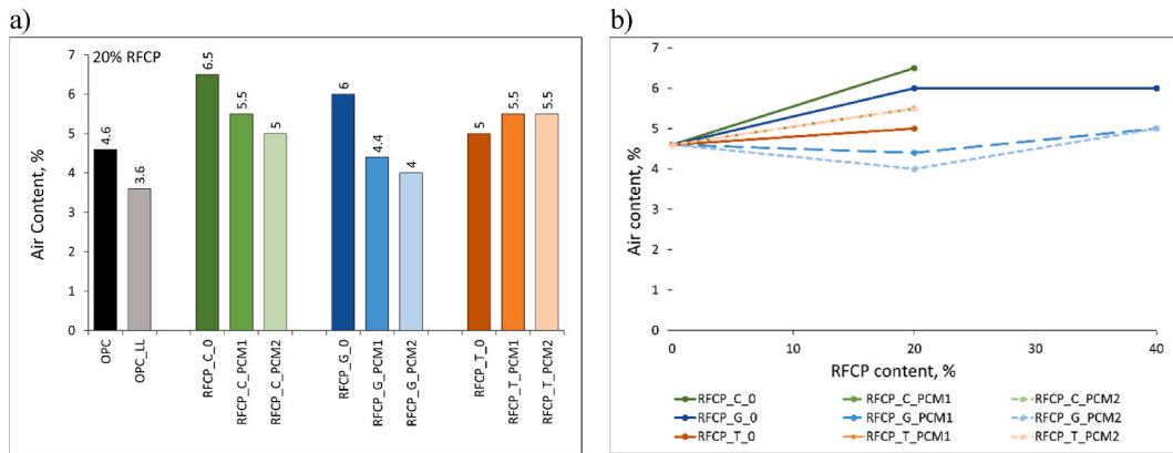
Fig. 15. Influence of type (a) and content (b) of RFCP on air content in fresh mortars with w/b = 0.50 .
