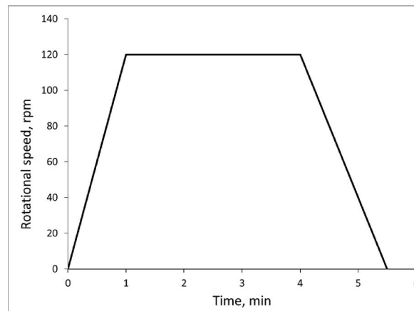
Fig. 4. The measurement procedure used in the rotational rheometer.
