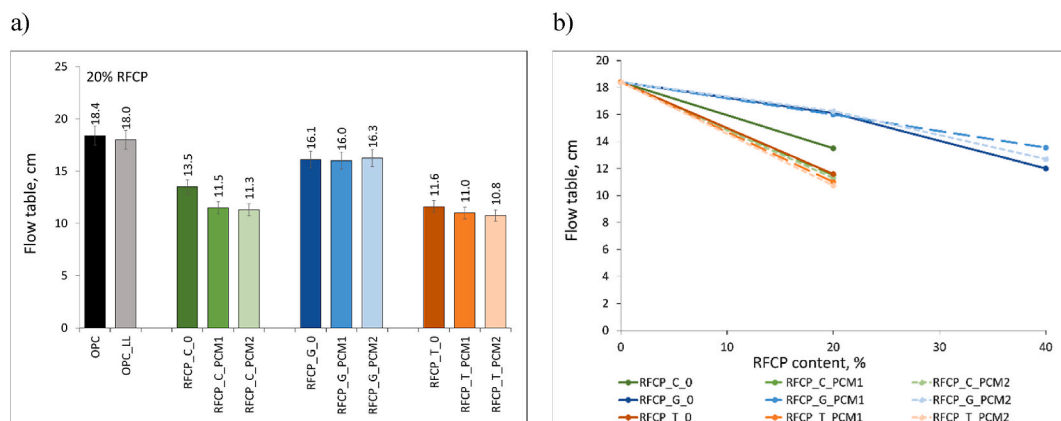
Fig. 9. Influence of type (a) and content (b) of RFCP on the consistency of fresh mortars with w/b = 0.50.
