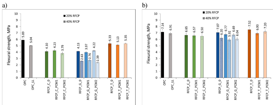
Fig. 17. Influence of RFCP type and content on flexural strength of mortars: a) after 2 days, b) after 28 days.
