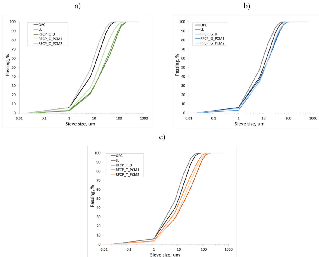
Fig. 1. Grain size distribution of OPC, LL and RFCP: a) RFCP_C; b) RFCP_G and c) RFCP_T.
