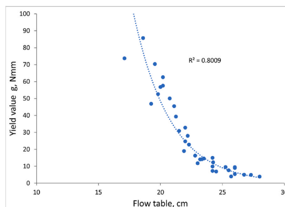
Fig. 13. Relationship between flow table diameter and yield stress ( g ) of fresh mortars with RFPC addition.
