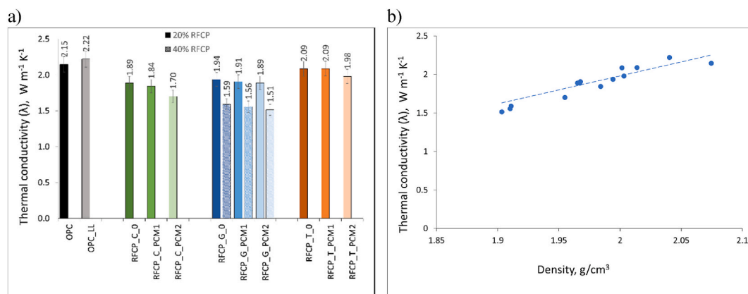
Fig. 24. a) The influence of type and content of RFCP on the thermal conductivity of mortars, b) the relationship between thermal conductivity and density of mortars.
