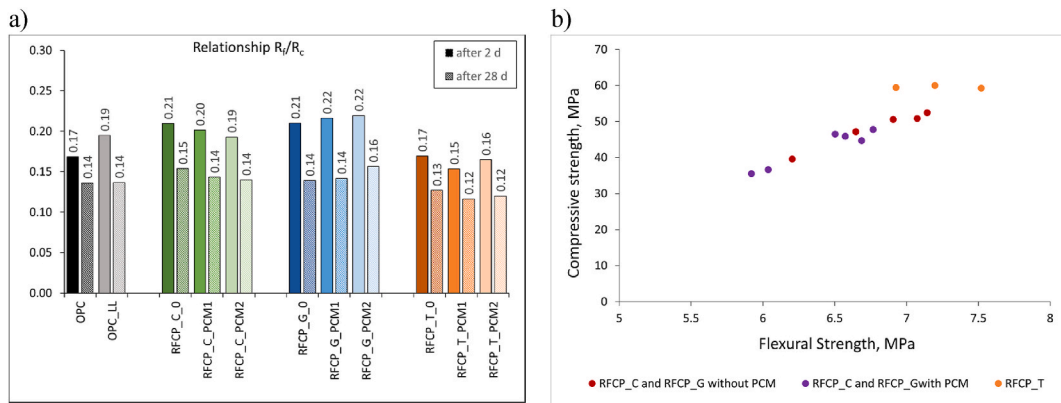
Fig. 20. Influence of RFCP on the relationship between flexural and compressive strength ( R_f/R_c ): a) all tested mortars, b) the impact of the RFCP type.
