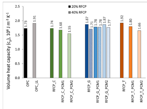
Fig. 25. The influence of type and content of RFCP on volume heat capacity of mortars.
