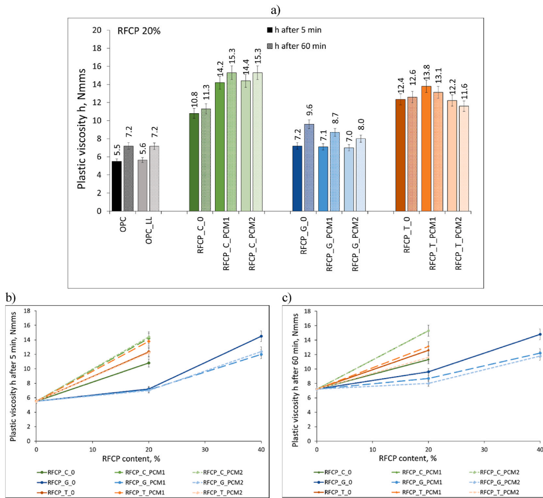
Fig. 12. Influence of type (a) and content of RFPC on plastic viscosity ( h ) of fresh mortars with w/b = 0.65 after 5 min (b) and 60 min (c).
