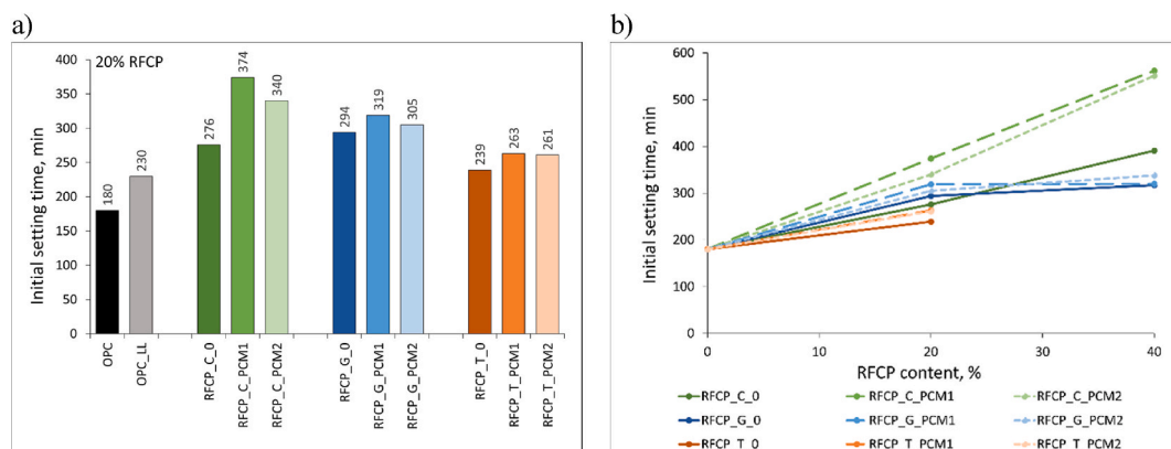
Fig. 6. Influence of type (a) and content of RFCP (b) on the initial setting time of pastes with standard consistency.
