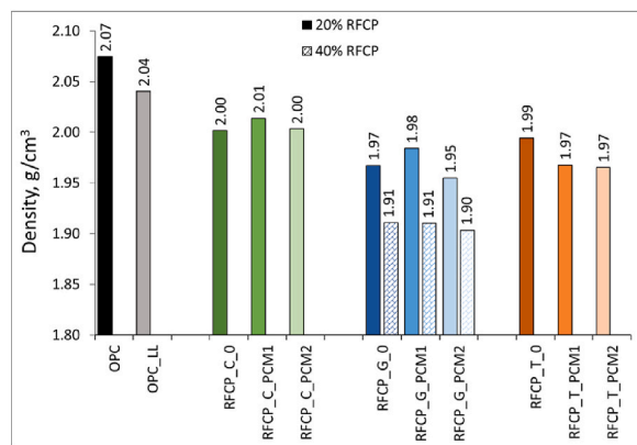
Fig. 16. Influence of RFCP type and content on the density of hardened mortars.
