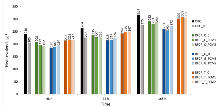
Fig. 8. The heat evolved in the presence of 20 % RFCP as cement replacement.
