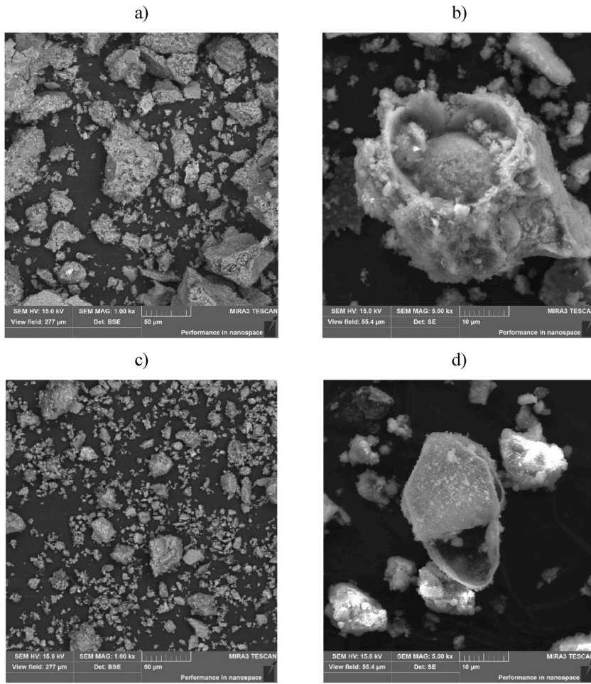
Fig. 2. SEM images: a, b) RFCP_C_PCM1 of grain size <0.125 mm (SSA 5917 cm 2 /g); c, d) RFCP_G_PCM1 of grain size <0.063 mm (SSA 6636 cm 2 /g).
