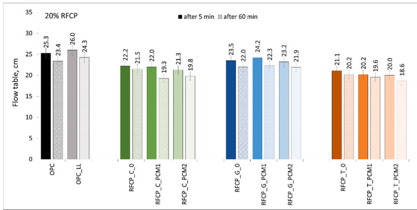
Fig. 10. Influence of type and content of RFPC on the consistency of fresh mortars with w/b = 0.65 after 5 and 60 min.
