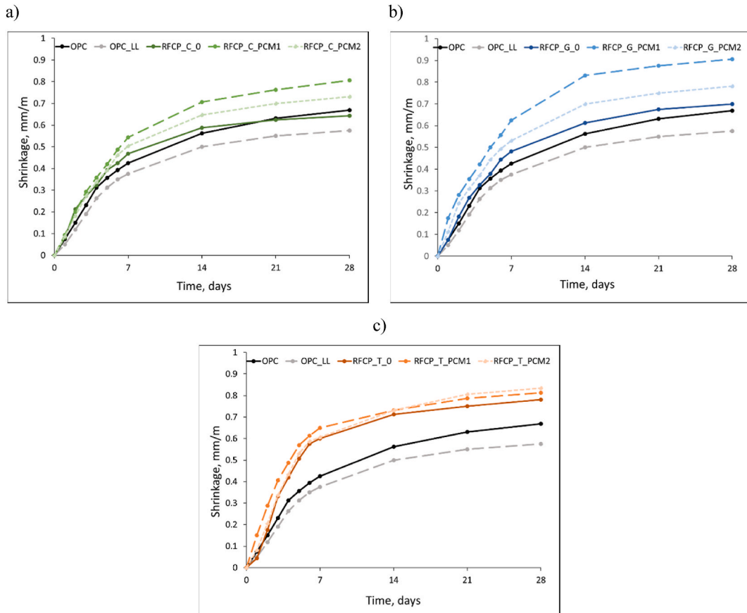
Fig. 21. Effect of 20 % RFCP on mortar shrinkage: a) RFCP_C, b) RFCP_G, c) RFCP_T.
