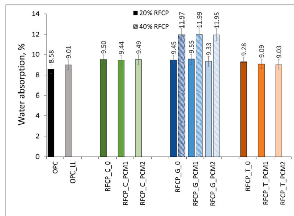
Fig. 23. Influence of RFCP type and content on water absorption of hardened mortars.
