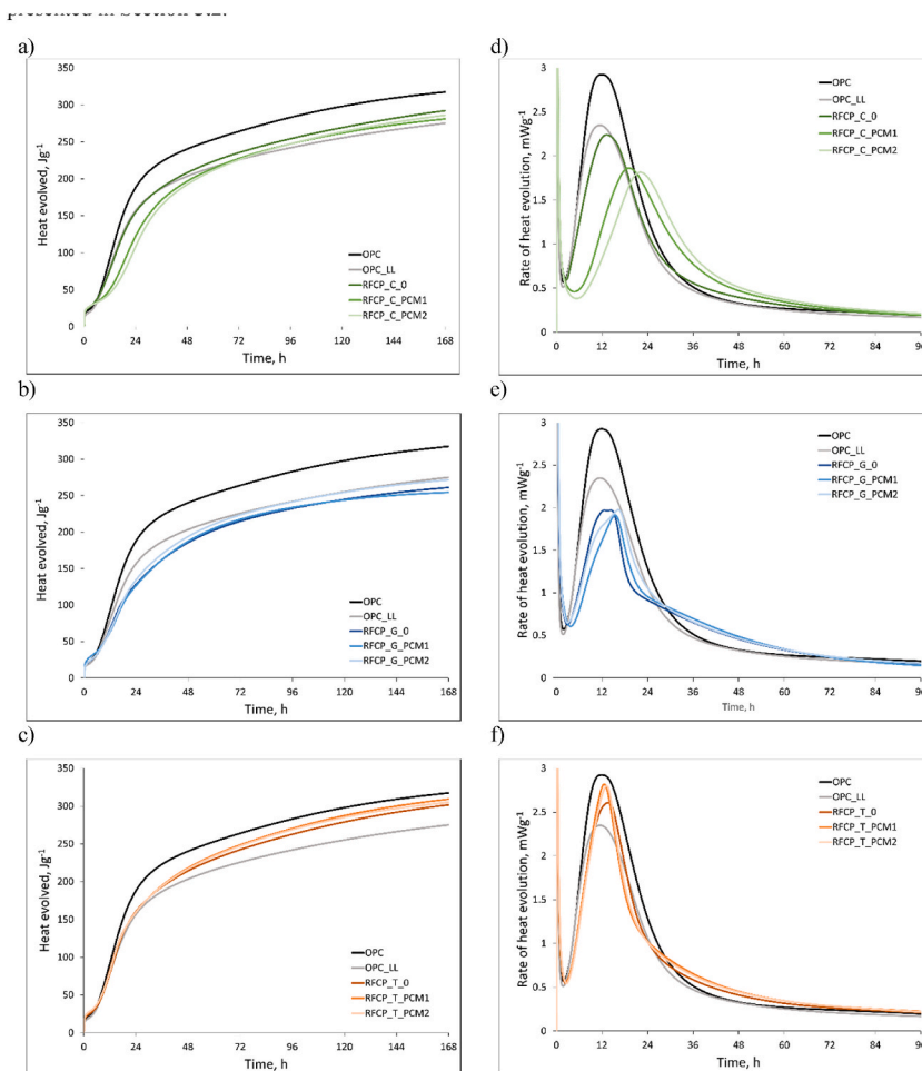
Fig. 7. The heat evolved in the presence of 20 % RFCP as cement replacement: a) RFCP_C, b) RFCP_G, c) RFCP_T and the rate of the heat of evolution of pastes with 20 % RFCP: d) RFCP_C, e) RFCP_G, f) RFCP_T.
