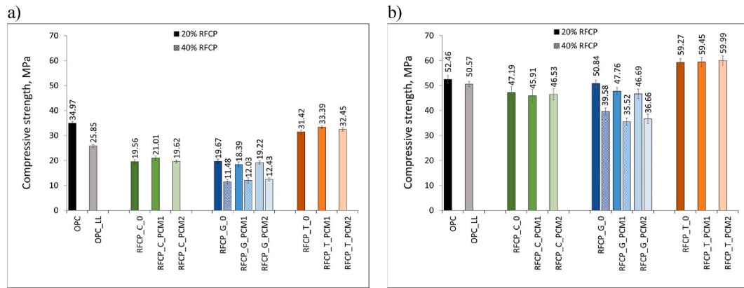
Fig. 18. Influence of RFCP type and content on compressive strength of mortars: a) after 2 days, b) after 28 days.
