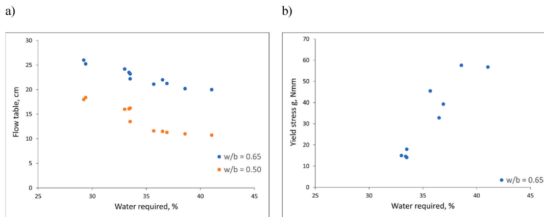
Fig. 14. Relationship between water required for standard consistency of paste and: a) flow of mortars of different w/b ratios, b) yield stress ( g ) of mortars.
