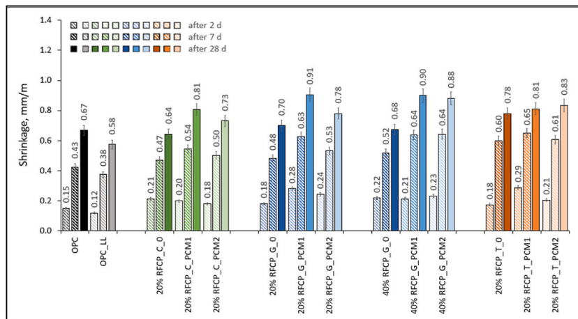
Fig. 22. Effect of RFCP type on mortar shrinkage after 2, 7 and 28 days of measurement.
