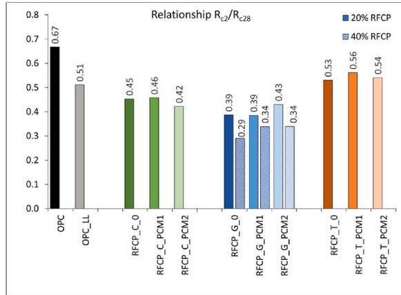
Fig. 19. Effect of RFCP on the ratio of early compressive strength development ( R_{c2}/R_{c28} ) in mortars.
