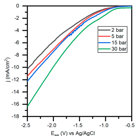
Fig. 5 LSV polarization curves at 10 \text{ mV s}^{-1} on a Au foil electrode in a 0.1 M KHCO_3 electrolyte under applied CO_2 pressures of 2, 5, 15, and 30 bar. The current density increases as expected with pressure
