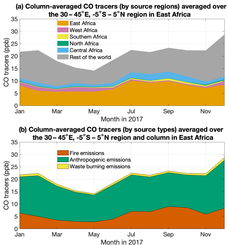
Figure 15. Monthly time series of column-averaged CO tracers in the 5° S–5° N, 30–45° E region in East Africa. (a) CO tracers of emissions from North Africa (green), West Africa (pink), East Africa (orange), Central Africa (blue), Southern Africa (yellow), and the rest of the world (grey). (b) CO tracers of fire emissions (red), anthropogenic emissions (green), and waste burning emissions (yellow).
