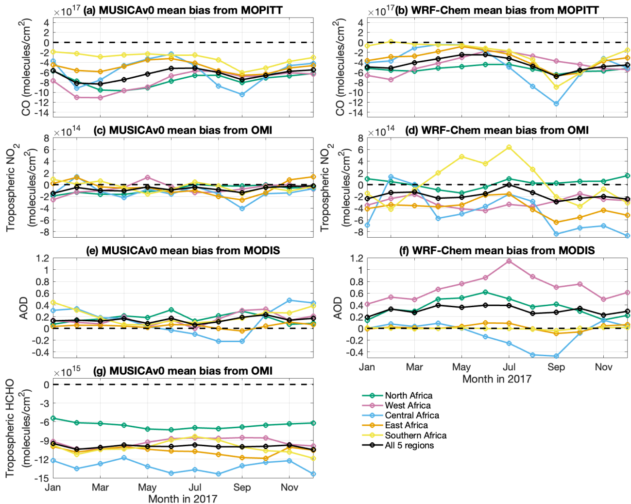
Figure 3. Mean bias of MUSICA v0 and WRF-Chem simulations from satellite data. Monthly time series of mean bias of (a) MUSICA v0 and (b) WRF-Chem against MOPITT CO column (molec. cm -2 ) in 2017 over Africa (black), North Africa (green), West Africa (pink), East Africa (orange), Central Africa (blue), and Southern Africa (yellow). Panels (c, d) are the same as (a, b) but for mean bias against the OMI tropospheric NO 2 column (molec. cm -2 ). Panels (e, f) are the same as (a, b) but for mean bias against MODIS (Terra) aerosol optical depth (AOD). Panel (g) is the same as (a) but for mean bias against the OMI tropospheric HCHO column (molec. cm -2 ).
