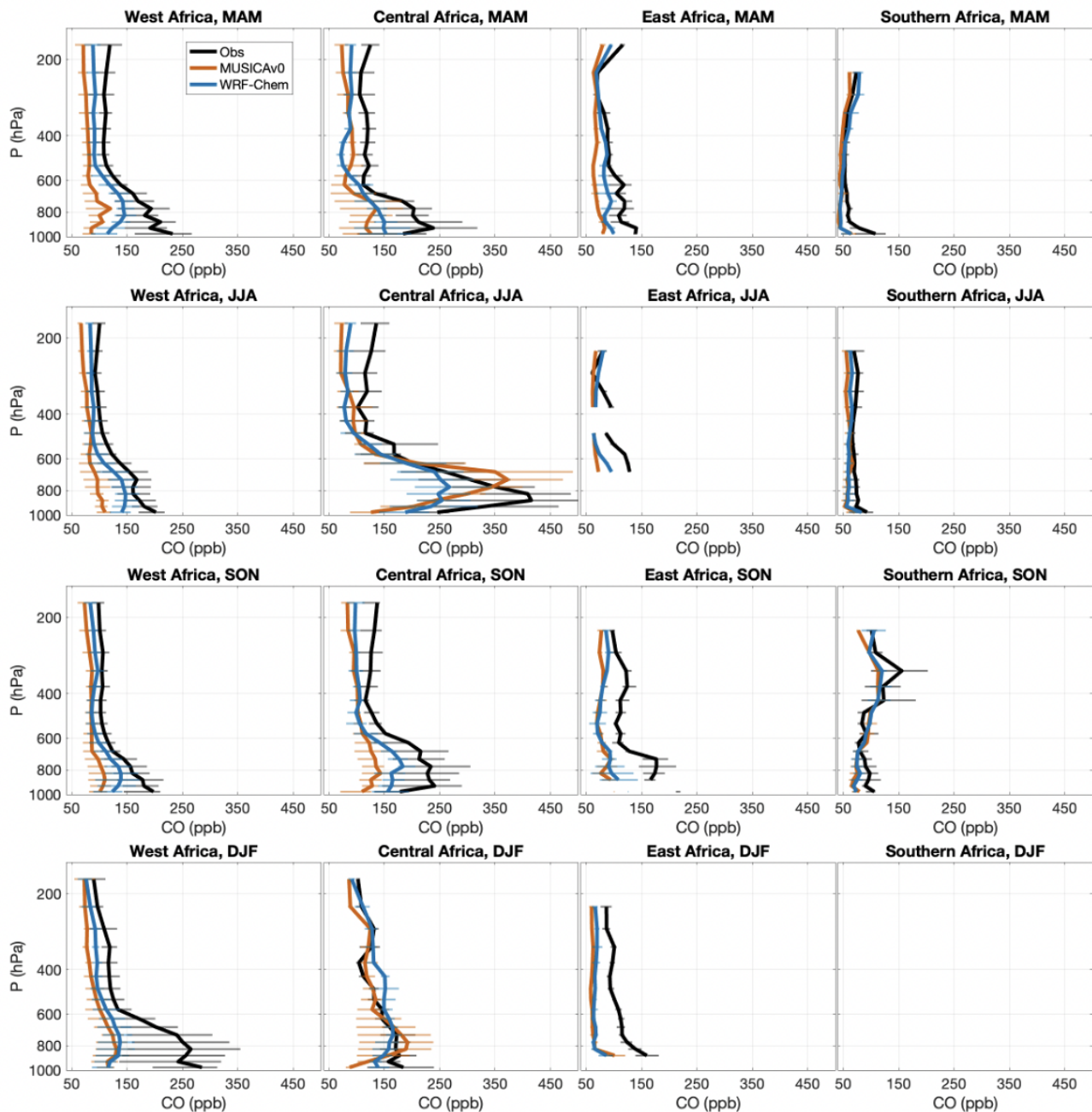
Figure 7. Vertical profiles of CO (ppb) from the In-service Aircraft for a Global Observing System (IAGOS) measurements (black) and corresponding model output from MUSICAv0 (red) and WRF-Chem (blue) during different seasons in 2017 over West Africa, Central Africa, East Africa, and Southern Africa. North Africa is not shown due to data availability. Seasonal mean profiles with the variation in the data in the pressure layer (25 % quantile to 75 % quantile) in MAM (March, April, and May), JJA (June, July, and August), SON (September, October, and November), and DJF (December, January, and February) are shown.
