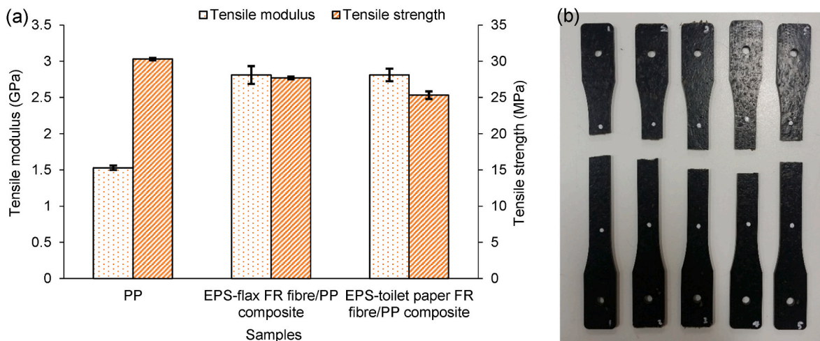
Fig. 10. (a) Tensile properties of PP, EPS-flax FR fibre/PP and EPS-toilet paper FR fibre/PP composites and (b) fractured specimens after tensile testing.
