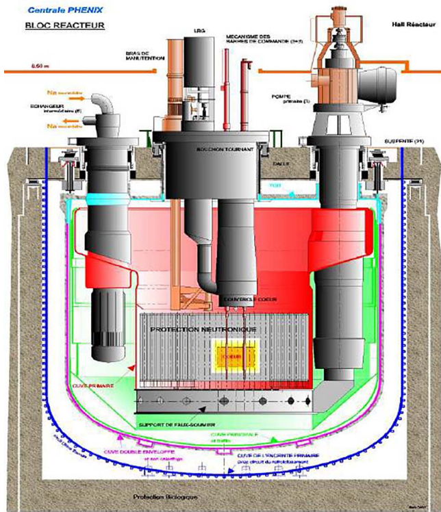
Fig. 1. Schematic of Phenix reactor block (International Atomic Energy Agency, 2013).
