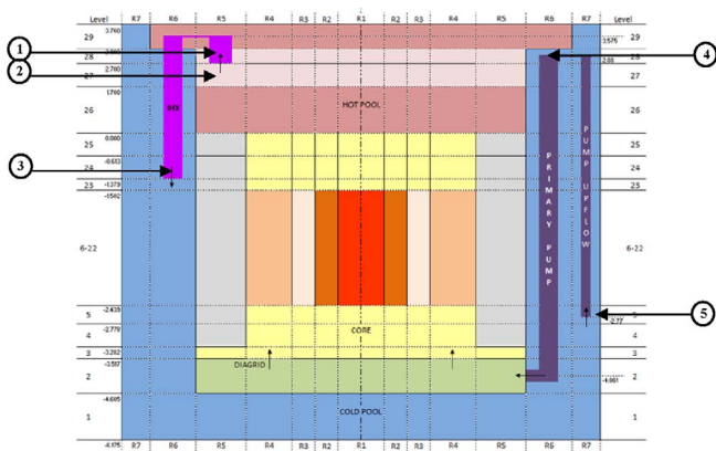
Fig. 4. TRACE VESSEL component axial discretization.
