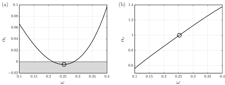
Figure 4: The leading or most unstable wavenumber as function of the temporal frequency \omega at Re = 7000 . (a) The imaginary part \alpha_i . Negative values of \alpha_i characterise unstable modes (gray region). (b) The real part \alpha_r . The point marked by 'o' corresponds to the most amplified frequency for the investigated conditions.
