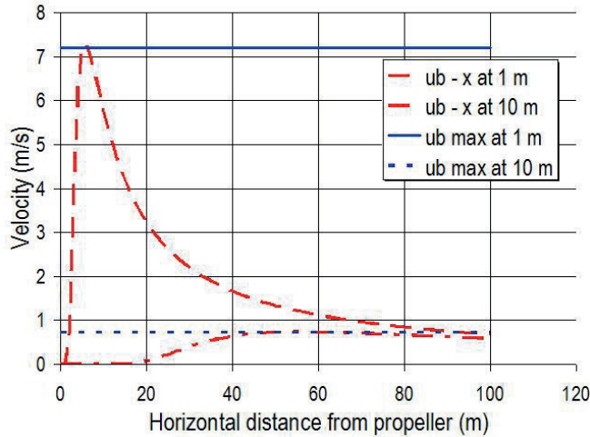
Figure 9-15 Velocities behind propeller for various cases
