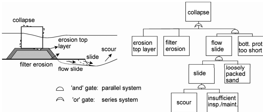
Figure 10-17 Series and parallel systems in fault tree
