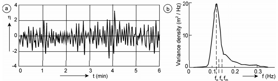
Figure 7-25 Wave registration and wave spectrum North Sea
