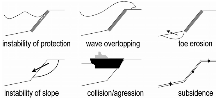
Figure 1-15 Failure mechanisms
