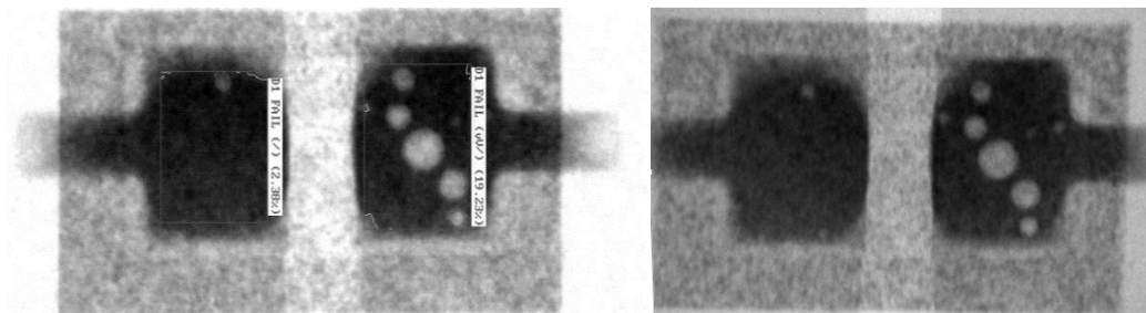
26 Figure 4. X-ray morphology of solder joint of one CSP LED at the aging time of 0 hour (left) and 27 300 hours (right) under 85°C & 85%RH environment
