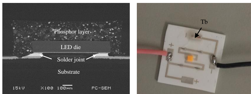
Figure 3. SEM image (left) and physical picture (right) of CSP LED mounted on a ceramic substrate
