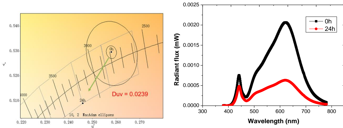
Figure 8. Color shift (left) and spectral change (right) of CSP LEDs under early period aging test
