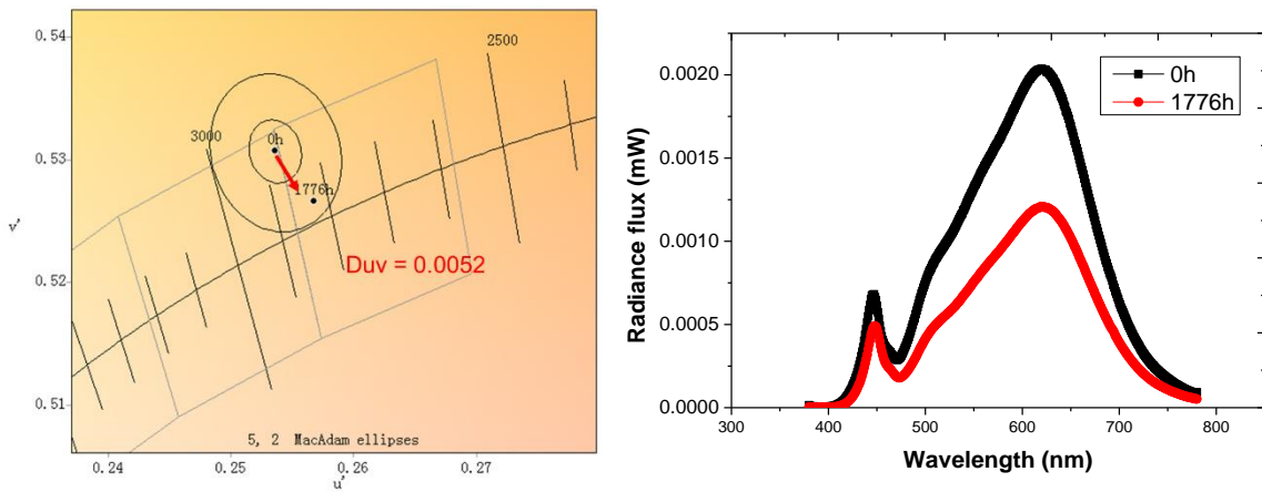
13 Figure 9. Color shift (left) and spectral change (right) of CSP LEDs under long-term aging test
