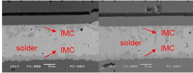
Figure 5. SEM images of solder layer of one CSP LED at the aging time of 0 hour (left) and 1000 hours (right) under 85°C & 85%RH
