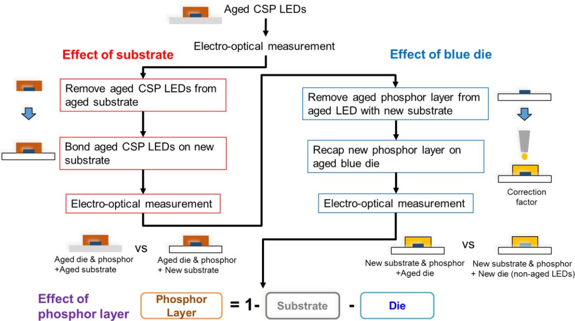
23 Figure 2. A series of experiments designed to investigate the impact of various components on the 24 reliability of CSP LED after aging test. 25
