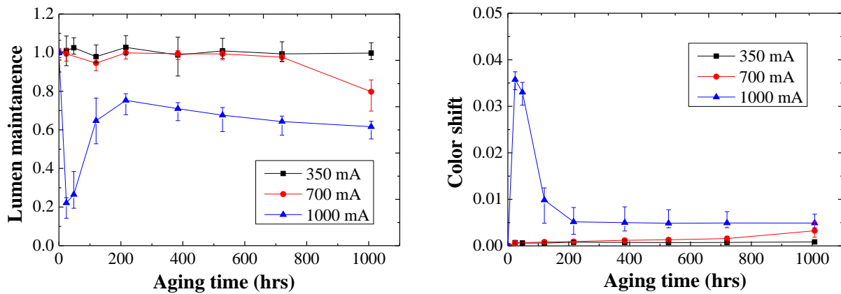
Figure 7. Lumen maintenance and color shift of CSP LEDs under RT aging as a function of time
