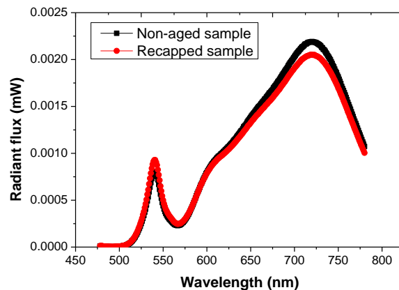
Figure 6. Spectral change between the non-aged and recapped CSP LEDs
