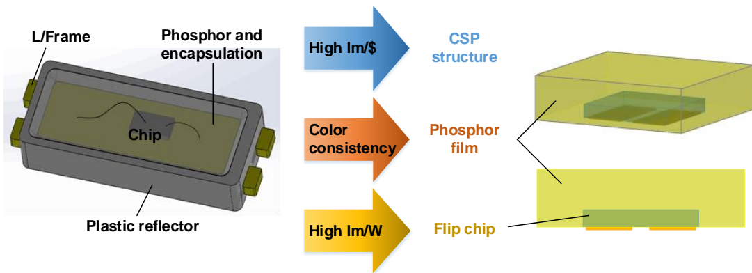
22 Figure 1. A SMD white LED package (left) compared to CSP LED (right)
