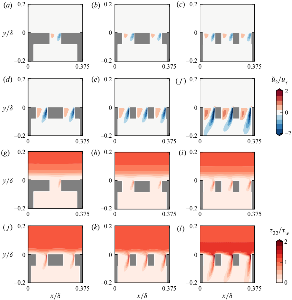
Figure 7. Mean wall-normal velocity \tilde{u}_2 (a–f) and wall-normal Reynolds stress \tau_{22} (g–l) over a liner cavity for flow cases L-L 3 (a,g), L-L 14 (b,h), L-L 32 (c,i), L-M 14 (d,j), L-M 32 (e,k) and L-H 32 (f,l).
