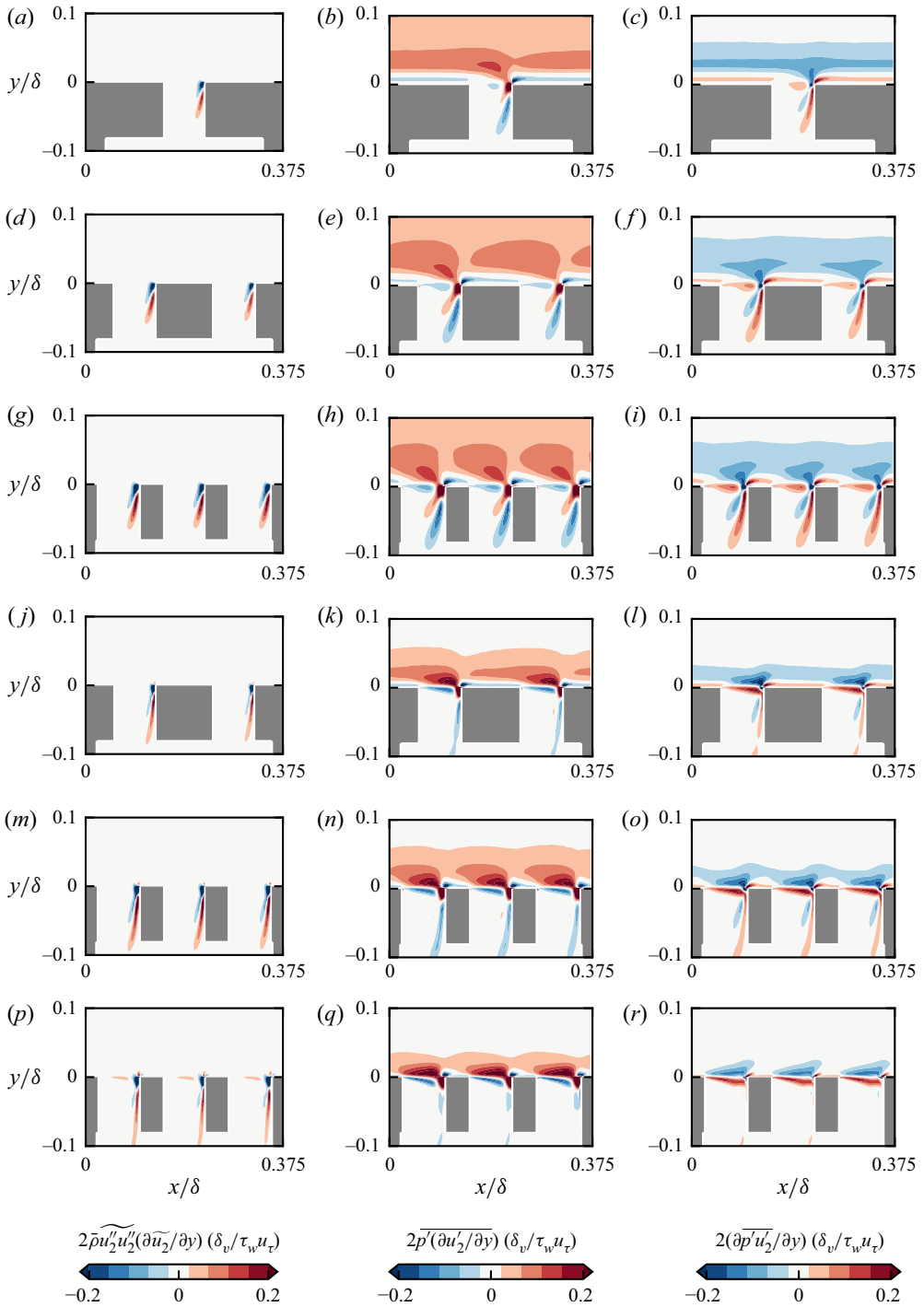
Figure 18. Contours of 2\bar{\rho}u_2''\widetilde{u_2''}\partial\bar{u_2}/\partial y (a,d,g,j,m,p), 2\bar{p}'\partial u_2'/\partial y (b,e,h,k,n,q) and 2\partial(\bar{p}'u_2')/\partial y (c,f,i,l,o,r) normalized by (\tau_w u_\tau)/\delta_v for cases L-L_3 (a-c), L-L_{14} (d-f), L-L_{32} (g-i), L-M_{14} (j-l), L-M_{32} (m-o) and L-H_{32} (p-r).
