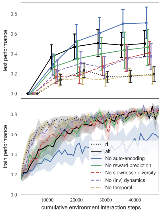
Fig. 5. The effect on the performance of the alt algorithm of turning off individual SRL losses. The no temporal experiment excludes both the (inv) dynamics and the slowness/diversity losses. The performance with all SRL losses ( alt ) and with no SRL losses ( r1 ) are shown for comparison. The mean \pm half a standard deviation of the performance criterion from Section IV are shown.
