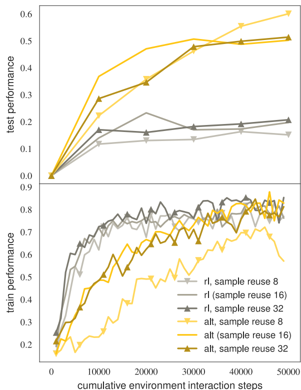
Fig. 4. The influence of the sample-reuse hyper-parameter on the train and test performance of the r1 and alt methods. The means of the performance criterion from Section IV are shown.
