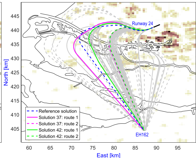
Fig. 7. Optimal ground tracks obtained in the second problem.
