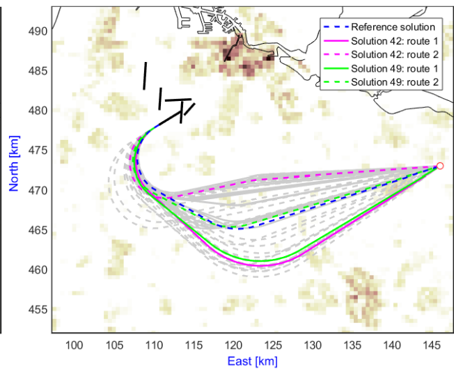
Fig. 14. Optimal ground tracks obtained in the second problem.
