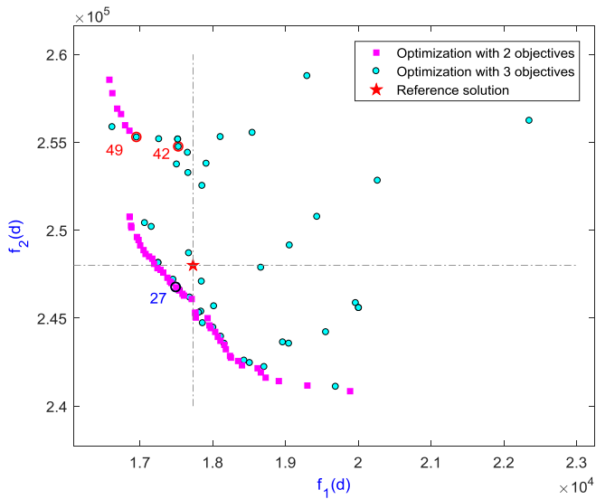
Fig. 11. Comparison of Pareto fronts obtained by the first and second problems and the reference case.
