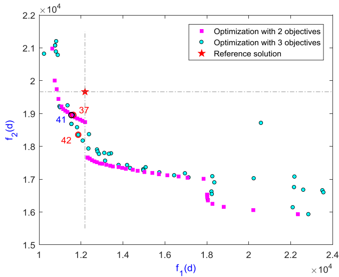
Fig. 4. Comparison of Pareto fronts obtained by the first and second problems and the reference case.
