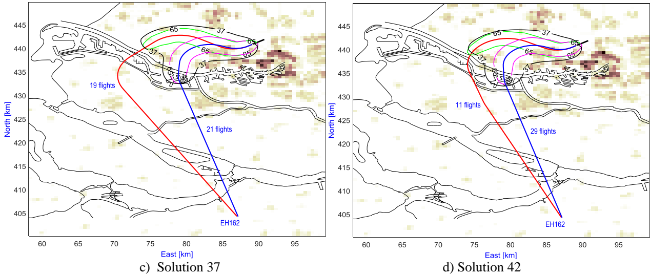
Fig. 8. Illustration of L_{den} and N65 contours of the representative routes and the reference case.
