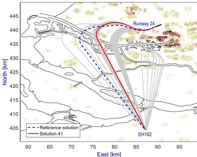
Fig. 6. Optimal ground tracks obtained in the first problem.
