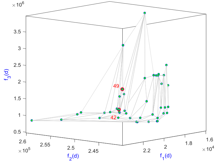
Fig. 12. Pareto fronts obtained by the second problem.
