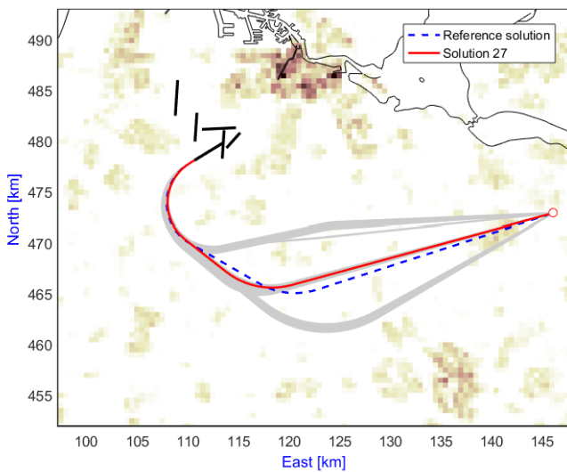
Fig. 13. Optimal ground tracks obtained by the first problem.
