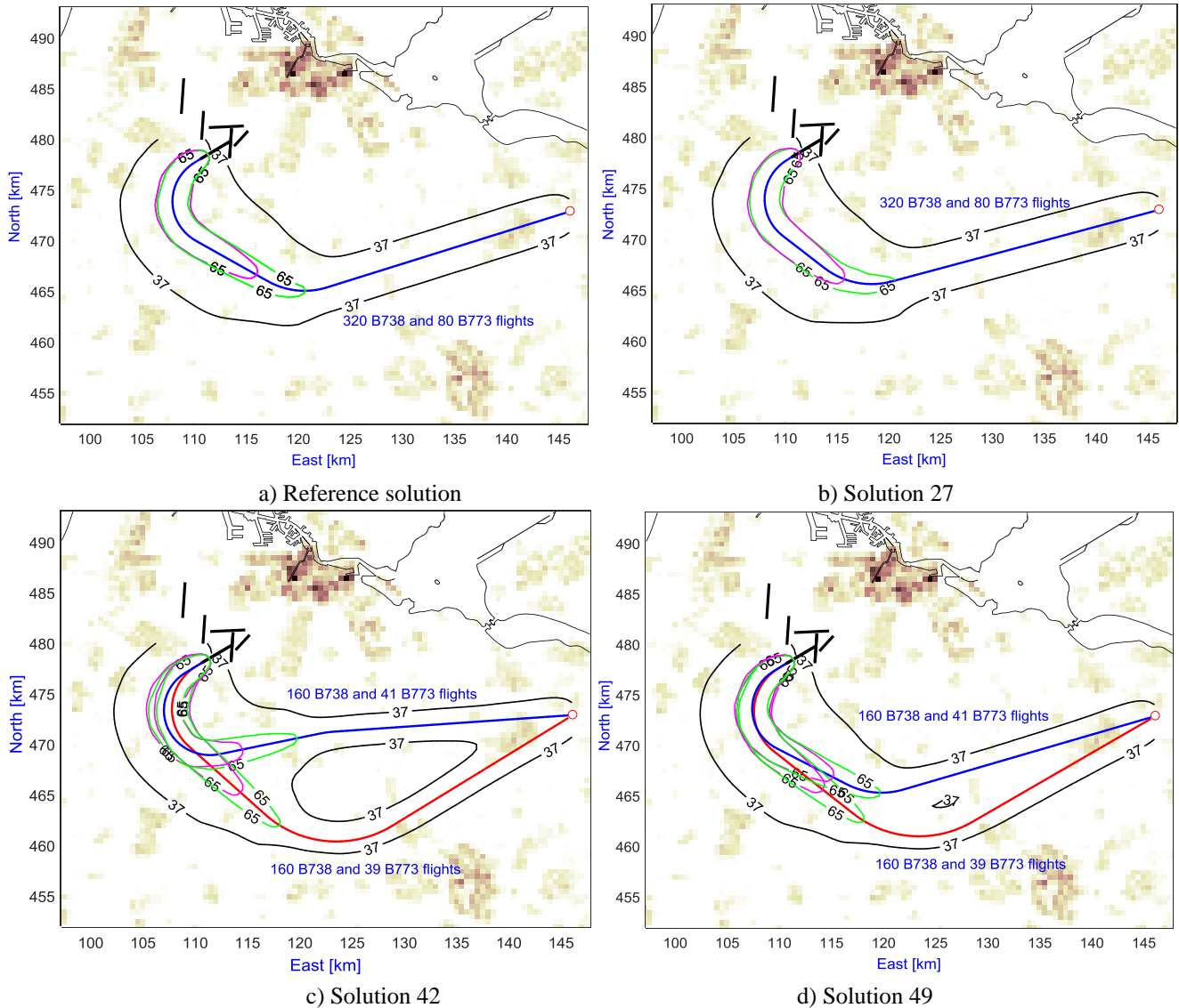
Fig. 15. Illustration of L_{den} and N65 contours of the representative routes and the reference case.
