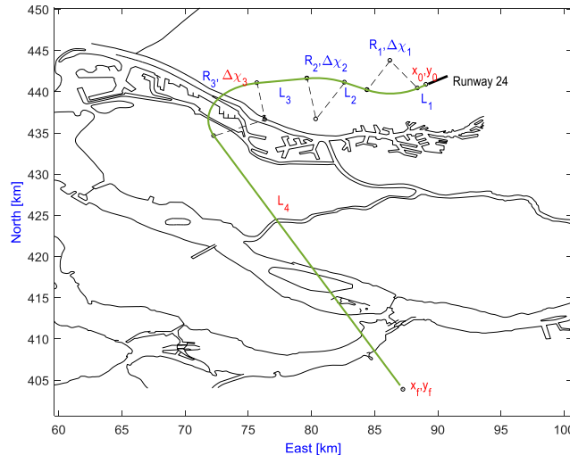
Fig. 1. Illustration of ground track parameterization.
