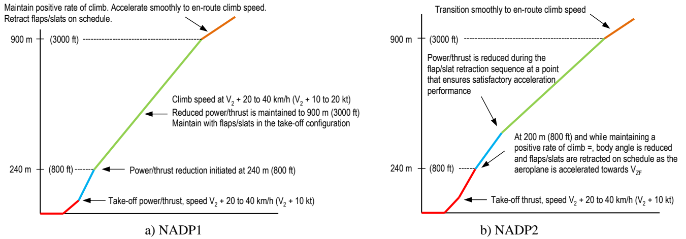
Fig. 2. Noise abatement departure procedure 1 and 2 (ICAO, 2006).
