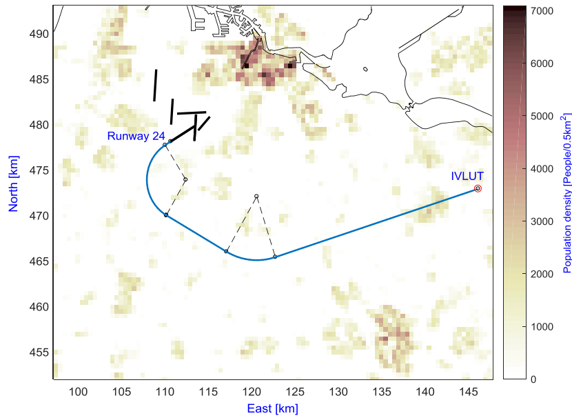
Fig. 10. Departure route LUNIX.
