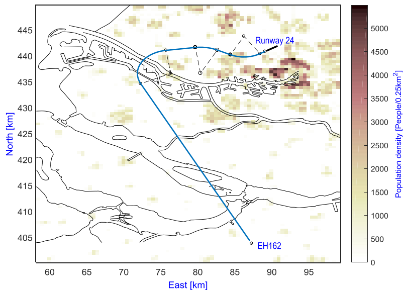
Fig. 3. Departure route WOODY.
