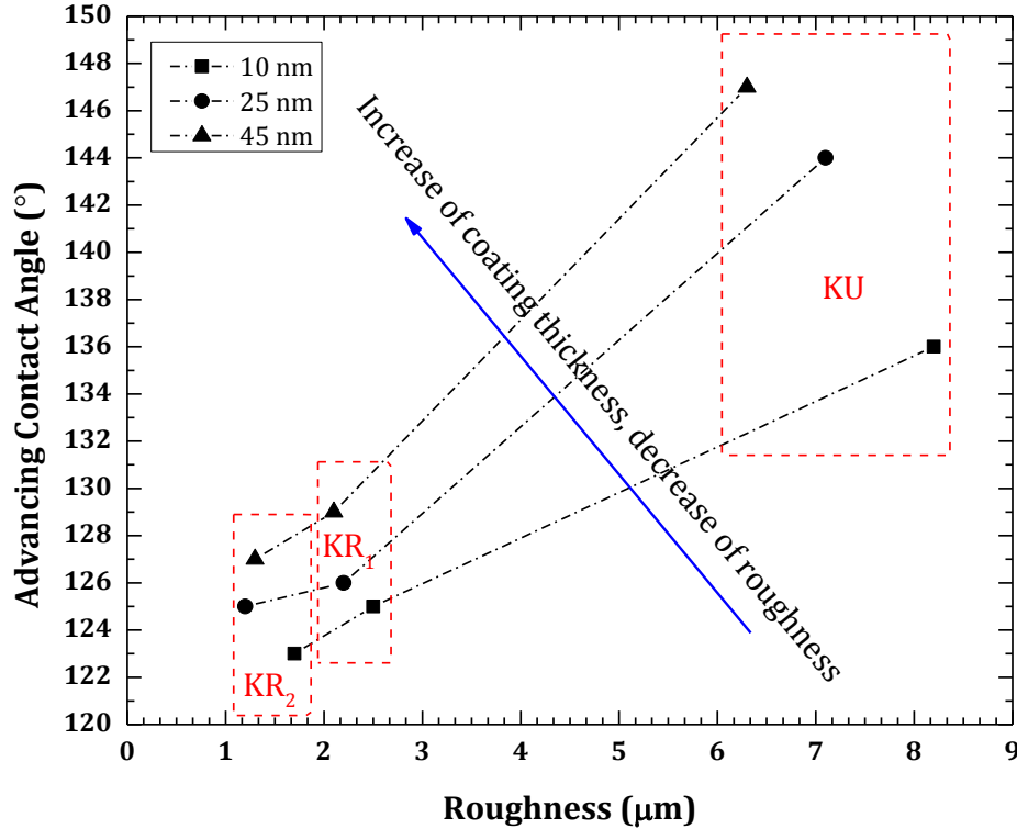
Figure 8. Effect of handsheet's roughness on advancing contact angles ( \theta_{Adv.} ) for handsheets prepared by Kraft pulp.
