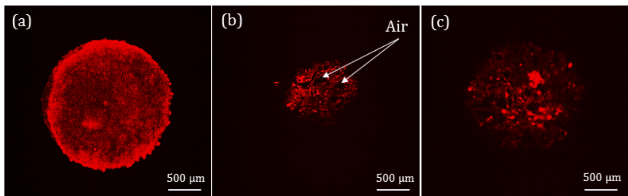
Figure 5. Stain of water droplet on (a) KR 2 handsheet with 25 nm Al 2 O 3 (b) KU handsheet with 25 nm Al 2 O 3 and (c) KU handsheet with 10 nm Al 2 O 3 .
