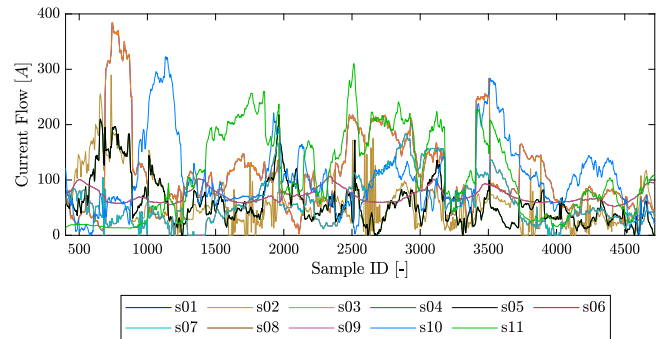
Fig. 4. Current flow for each line monitored by the corresponding self-organizing sensor weather station.
