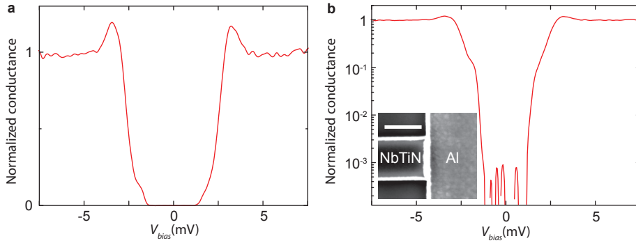
Figure 6.9: dI/dV characteristics of a single NbTiN/AlO x /Al tunnel junction with a normal state resistance of R_N = 2.4 \text{ M}\Omega on the linear (a) and on the logarithmic scale (b), respectively. The measurement was performed at T = 300 \text{ mK} . The inset in (b) shows the scanning electron microscope image of the device. The scale bar denotes 500 nm.
