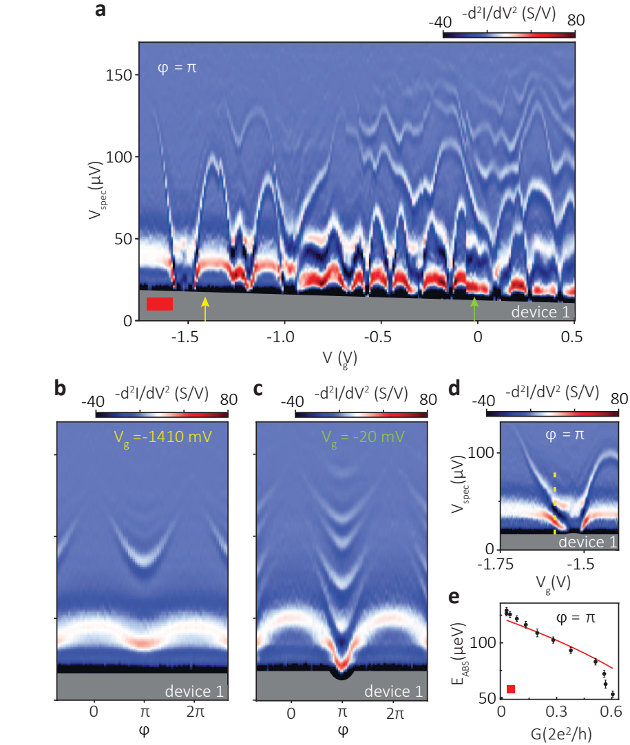
Figure 9.2: Gate dependence of Andreev bound states. (a) -d^2I/dV^2 of the spectrometer junction as a function of V_g at \phi = \pi , where E_{\text{ABS},i} = \Delta\sqrt{1 - T_i} in the short junction limit. Panels (b) and (c): -d^2I/dV^2 of the spectrometer junction as a function of \phi = 2\pi\Phi/\Phi_0 for one channel (b) and several channels (c). The qualitative agreement of the line shapes with Eq. 9.1 confirms the short junction behaviour. Arrows in panel (a) indicate V_g for these measurements. Weakly visible vertically shifted replicas of the ABS lines indicate higher order transitions, see text. (d) Strong hybridization between the ABS excitation and the plasma mode with a level repulsion of \varepsilon = 22 \mu\text{eV} at the yellow dash line. (e) E_{\text{ABS}}(\phi = \pi) as a function of the DC linear conductance G of the nanowire weak link in the gate span denoted by the red bar in panel (a). The solid red line shows the prediction of the single channel model with \Delta = 122 \mu\text{eV} \pm 3 \mu\text{eV} , see text. All data was taken on device 1. Grey regions denote lack of data due to bias instability of the circuit.
