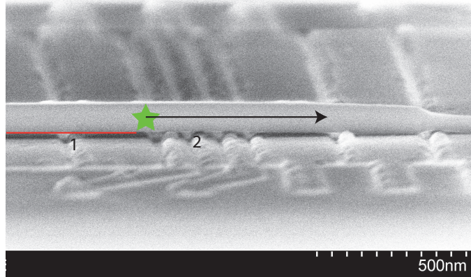
Figure 10.2: SEM image of a nanowire on local fine gates. Air voids are present between the nanowire and the dielectric, which leads to non-uniform gating[139]. This SEM image is an extreme case since the gold lift-off for the gates left small bumps, lifting the nanowire from the flat parts of the gates. The red line depicts the topological region, with the MZM at the end (green star). The question is: can the topological region be extended over the regions with air voids?
