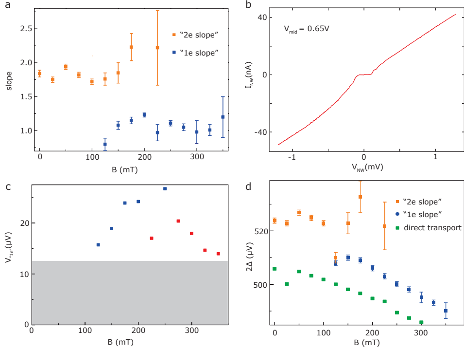
Figure E2: Similar data as shown in fig. 8.4 but with V_{\text{sidegate}} = 1.25\text{V} and V_{\text{mid}} = 0.65\text{V} . a Extracted slopes at different applied magnetic fields along the nanowire. In a range of (125-225mT) magnetic field two different slopes of radiation in the detector is measured. b The measured current versus the measured voltage of the nanowire. The normal state resistance on the negative voltage bias is R_{N,-} = 30.9\text{k}\Omega . c The length of the \sim 1 slope. The end of the slope is determine by the start of the \sim 2 slope (blue datapoints) or by lost of the signal (red datapoints). d The extracted values for 2\Delta are determined by extrapolating to slopes to V_{\text{NW}} = 0\text{V} .
