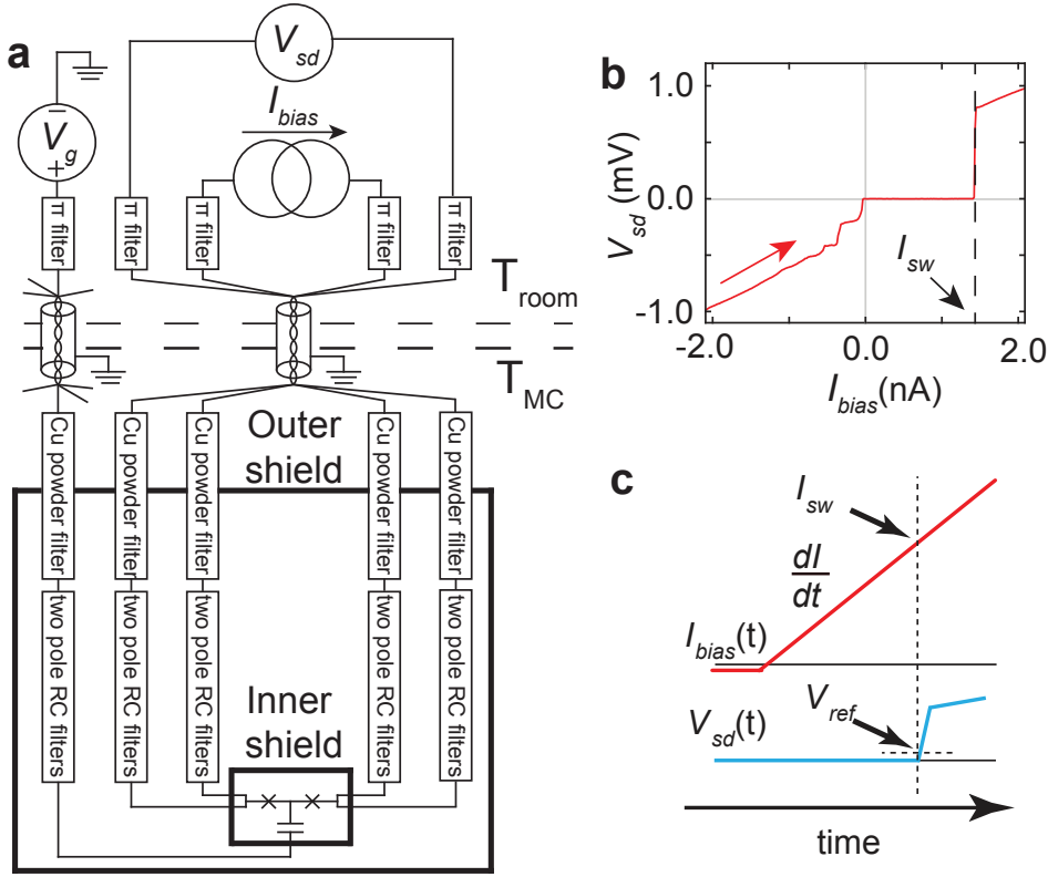
Figure 6.7: Measurement electronic setup and typical waveforms. (a) Schematics of the measurement. (b) Typical experimental V - I trace exhibiting a well-defined switching current, I_{sw} . We observe a retrapping current I_r \ll I_{sw} characteristic to unshunted Josephson junctions in the low temperature limit [177]. The additional features in the resistive state are consistent with Fiske steps [178]. (c) Current ramp (red) with a slope of dI/dt probing I_{sw} which is recorded when the measured V_{sd} (blue) reaches V_{ref} \sim 10 \mu V .
