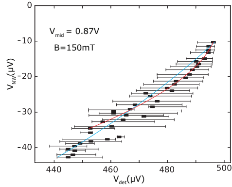
Figure E3: Different possible fits for the 150mT used in figure 8.4(c). The fit in cyan assumes a single slope ( 1.52 \pm 0.05 ) but leave many datapoint below the fit, especially around V_{\text{NW}} \sim 20\mu\text{eV} . The red line is a quadratic fit, which is only a good fit up to V_{\text{NW}} \sim 30\mu\text{eV} but after this point all the datapoints are missed.
