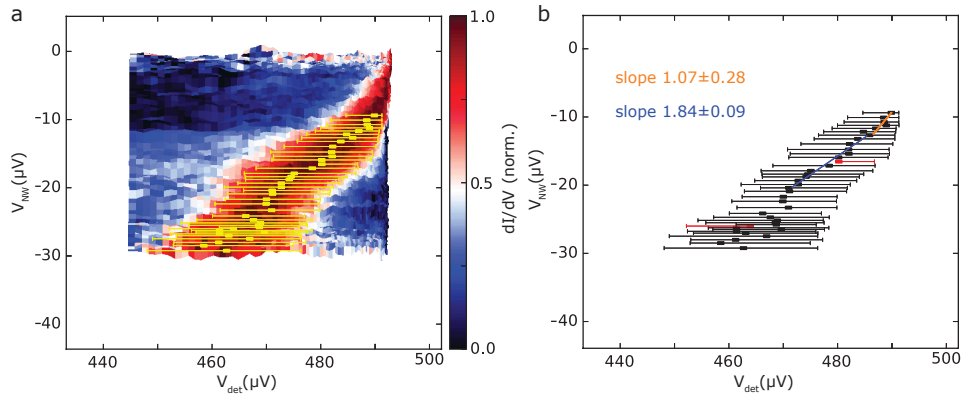
Figure E4: An example of the raw normalized data measured in the detector when the nanowire normal state resistance is R_{N,-} = 8.9\text{k}\Omega which is below the resistance quantum, this indicated multiple channels. a Raw normalized data overlayed with the extracted maximum and the FWHM. The (raw) data is showing a single radiation peak with the accessible linewidth. b The extracted data points fitted with a two slopes up to V_{\text{NW}} \sim 20\mu\text{eV} . After V_{\text{NW}} \sim 20\mu\text{eV} the slope seems to become steeper (more towards 1 again), without understanding the possible origin. The red data points are not taking into account since the peakfinder algorithm could not find a FWHM on one side.
