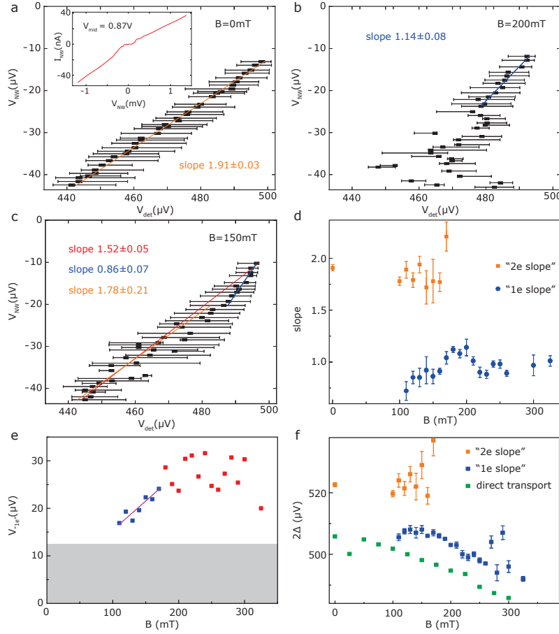
Figure 8.4: Analysis of the radiation emitted from the nanowire Josephson junction with the magnetic field applied along the nanowire ( < 5^\circ ) and with V_{\text{mid}} = 0.87\text{V} and V_{\text{sidegates}} = 1.75\text{V} . A similar data set is shown in Figure E2 for a different gate configuration. a Same plot as 8.3f. Inset: the IV trace of the nanowire Josephson junction, used to determine the normal state resistance, R_{N,\pm} . b Extracted peak positions of the detected lock-in signal when a magnetic field of 200mT is applied along the nanowire. At V_{\text{NW}} \sim 22\mu\text{V} , the algorithm cannot find the peak reliably. In Figure E1b, the extracted peak positions are overlaid with the normalized raw data. The data up to V_{\text{NW}} \sim 22\mu\text{V} shows a slope of 1.14 \pm 0.08 between nanowire and detector voltage. c Extracted peak position of the lock-in signal in the detector at a magnetic field of 150mT. When all the data points are used for a linear fit (red), a slope of 1.52 \pm 0.05 is obtained. Many data points, especially for low nanowire voltages, are below the fitted line. We believe the data is better described by two separate slopes, as shown by the blue and orange lines. In Figure E3, we show another possible fit which we believe is less appropriate. d The extracted slopes, before and after the 'kink'. In the range \sim 100 – 300\text{mT} , a \sim 1 slope is fitted. e The end of the \sim 1 slope. For the blue data points, the \sim 1 slope ended due to a second slope (effectively the position of the 'kink'), while for the red data points it ended due to the lack of a visible signal in the data. f The extracted 2\Delta for the different slopes, assuming that the slopes are linear up to zero nanowire voltage. The green points show the gap extracted from direct measurements. Due to quasiparticle heating, the exact value of 2\Delta could not be extracted accurately from the IV trace, but this data shows the trend with magnetic field.
