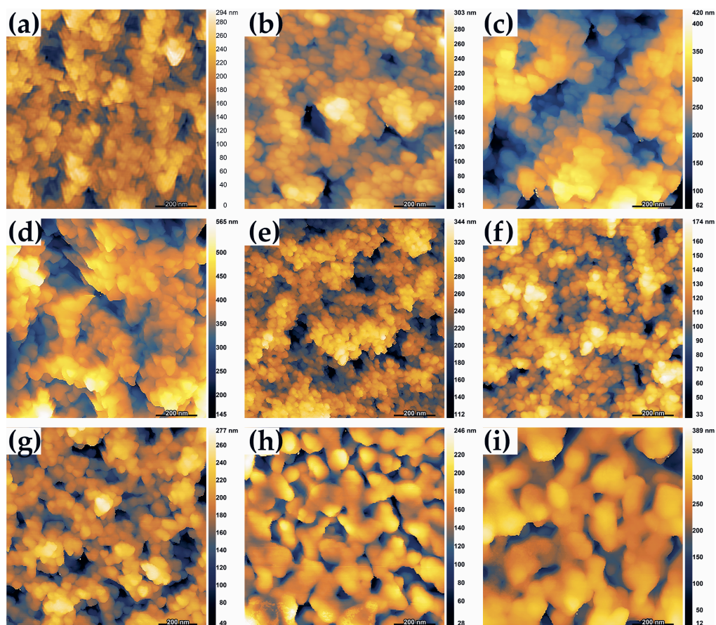
Figure 5.3: AFM morphology of 1.0 \times 1.0 ( \mu\text{m}^2 ) areas of a) non-heat treated samples (b) 15 minutes at 100 °C, (c) 30 minutes at 100 °C, (d) 120 minutes at 100 °C, (e) 15 minutes at 120 °C, (f) 30 minutes at 120 °C, (g) 5 minutes at 150 °C, (h) 15 minutes at 150 °C, (i) 5 minutes at 200 °C.
