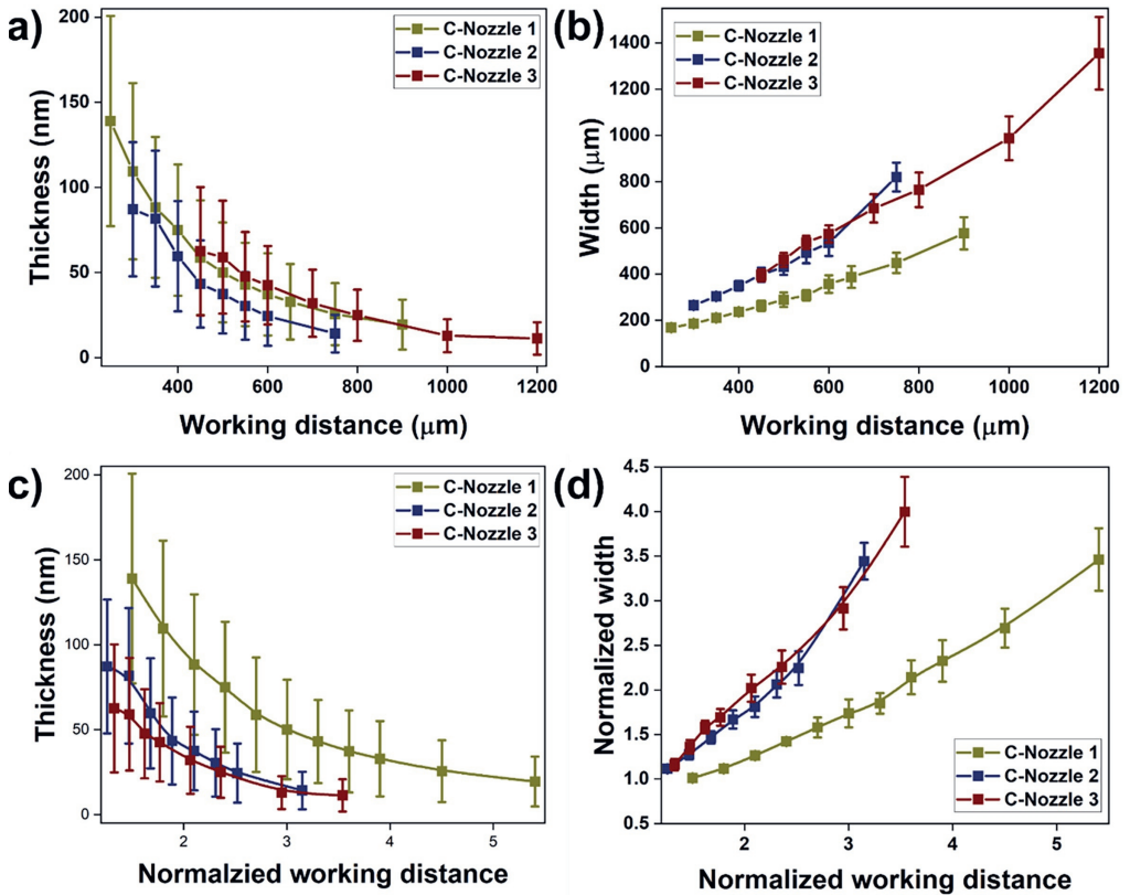
Figure 3.9: Effect of working distance on a) thickness and b) width of the AuNPs line printed with three converging nozzles of C-Nozzle 1-3 with a diameter of 166.5, 238 and 339 μm. c) Thickness and d) normalised width to normalised working distance with corresponding nozzle diameter. The stage speed is set to 0.44 mm/s.
