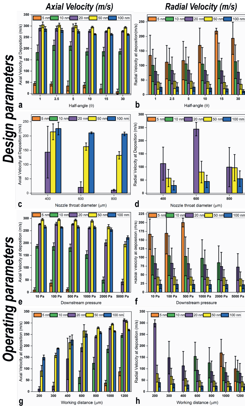
Figure A.15: Axial and radial velocity for copper nanoparticles when impacting on the impaction plate with sizes indicated in the figure for CN, a) and b) for the angle of converging nozzle, c) and d) for throat diameter, e) and f) for downstream pressure and g) and h) WD.
