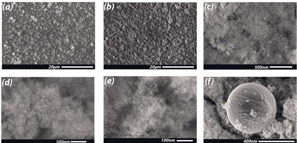
Figure B.2: SEM images of the CuNPs deposited on a silicon substrate with SAM voltage/current setting of V=1.2 kV, I=8 mA a) Centric region and b) boundary of the line, c) presence of microparticles in the film of CuNPs, d) and e) Morphology of film at high-resolution image f) a typical microparticle
