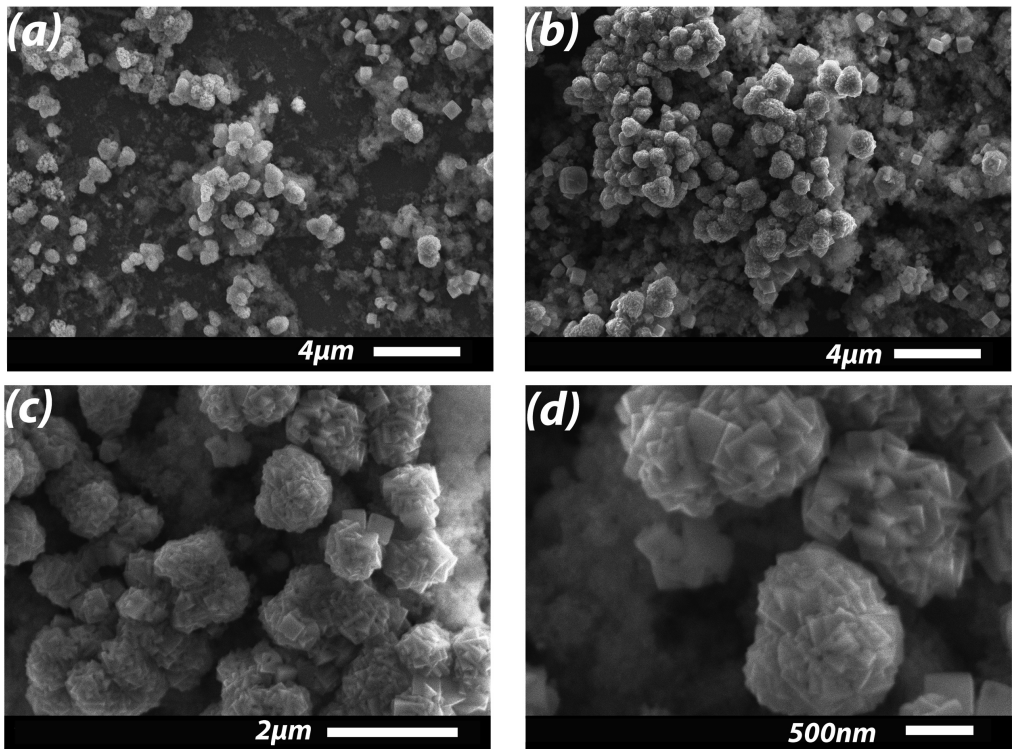
Figure B.4: SEM images of CuNPs deposited on a silicon substrate after thermal treatment in a vacuum oven for 2 hours at 200^{\circ}\text{C} and SAM voltage/current setting of V=1.2\text{ kV} , I=8\text{ mA} . a) evolution of morphology from cubic aggregates to bulk aggregates moving from center to the boundary b),c),d) high magnification of bulk aggregates
