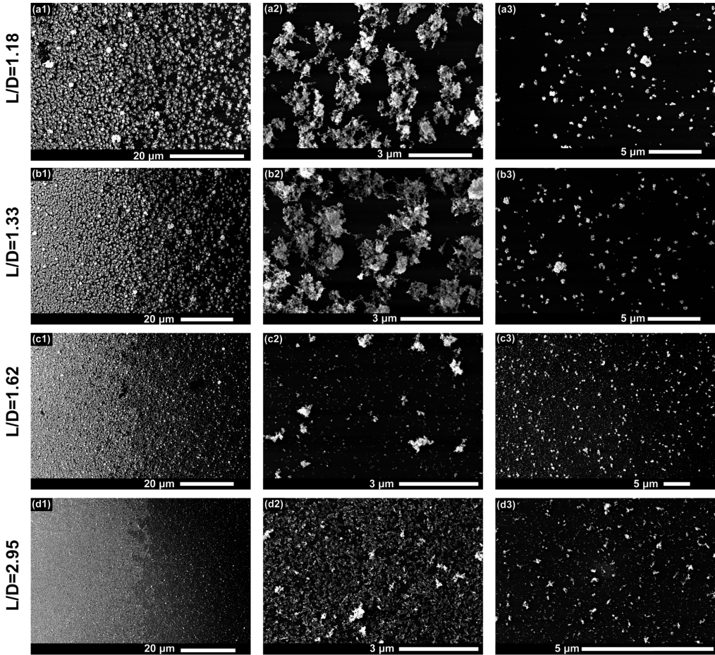
Figure A.20: (a1-d1) SEM images of the border between boundary and splash zones for lines printed with 339\ \mu\text{m} nozzle and WDs as indicated in the figure and (a2-d2) focusing in splash zones closer to the boundary, and (a3-d3) further away from the line in the splash zone.
