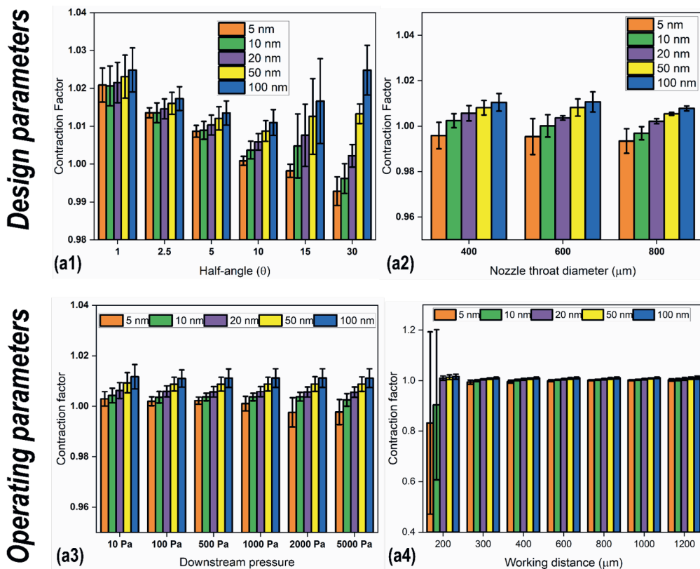
Figure A.12: Contraction factor for copper nanoparticles with sizes indicated in the figure for CN considering design parameters of a) angle of converging nozzle, b) throat diameter, and operating parameters of c) downstream pressure and d) WD.
