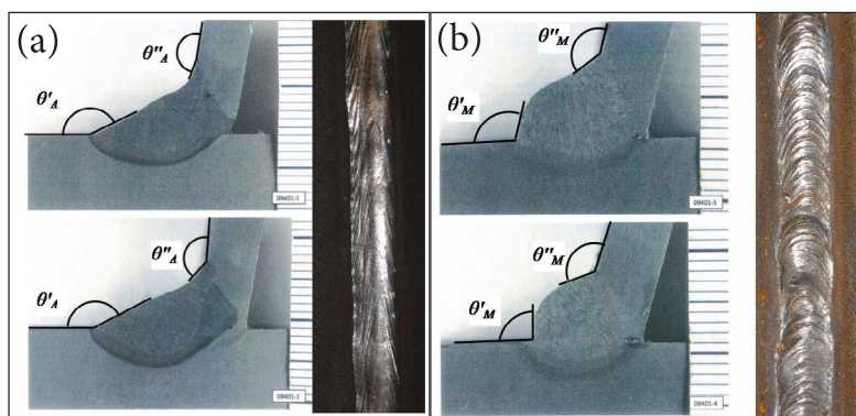
Fig. 4. Representative cross-sections of the stiffener-to-deck plate connections: (a) W1, and (b) W2.
