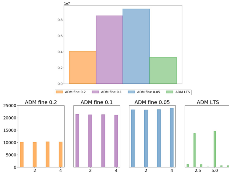
Fig. 23. Test case 4 - Total amount of active cells multiplied by number of Newton iterations (top) and computational complexity history at each local times step within a global step (bottom) for the ADM approach.
