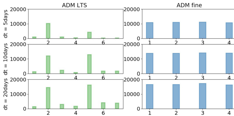
Fig. 7. Test case 1 [99 × 99] - Computational complexity history at each local times step within a global step. The computation complexity is the number of active cells multiplied by the number of Newton iterations.
