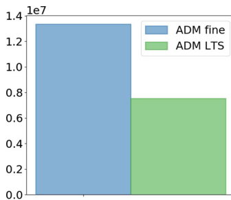
Fig. 8. Test case 1 [198 × 198] - Total amount of active cells multiplied by number of Newton iterations for the ADM with fine time steps and the ADM LTS method.
