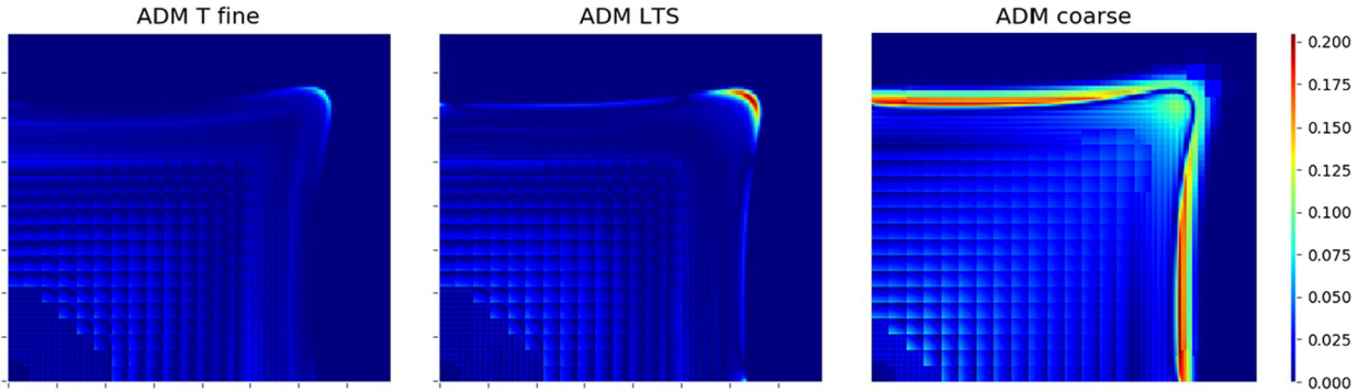
Fig. 10. Test case 1 [198 × 198] - Saturation errors at time t = 540 [days] for the ADM method with fine grid in time (left), ADM-LTS method (center) and the ADM method with coarse grid in time (right).
