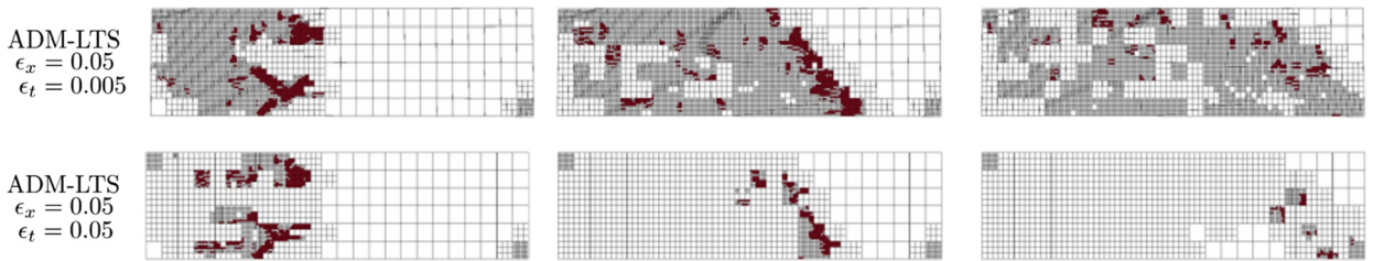
Fig. 26. Test case 5 - Active cells for the refinement level l_{ref} = 2 , at 150 (left), 250 (center) and 350 (right) days for the two threshold values.
