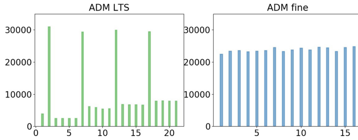
Fig. 9. Test case 1 [198 × 198] - Computational complexity history at each local times step within a global step. The computation complexity is the number of active cells multiplied by the number of Newton iterations.
