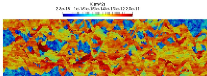
Fig. 24. Test case 5 - Natural logarithm of the permeability.
