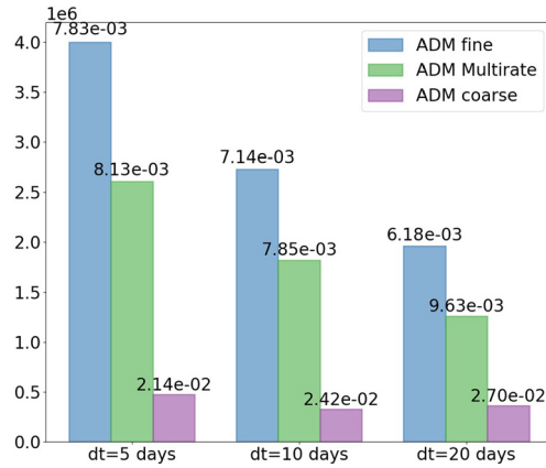
Fig. 6. Test case 1 [99 × 99] - Total amount of active cells multiplied by number of Newton iterations for the three different time step sizes. On the top of each bar the mean in time of the averaged absolute difference respect to the reference solution for the saturation is displayed E_s = \text{mean}|S(t_f) - S_{ref}(t_f)| where t_f is the final time 600 days.
