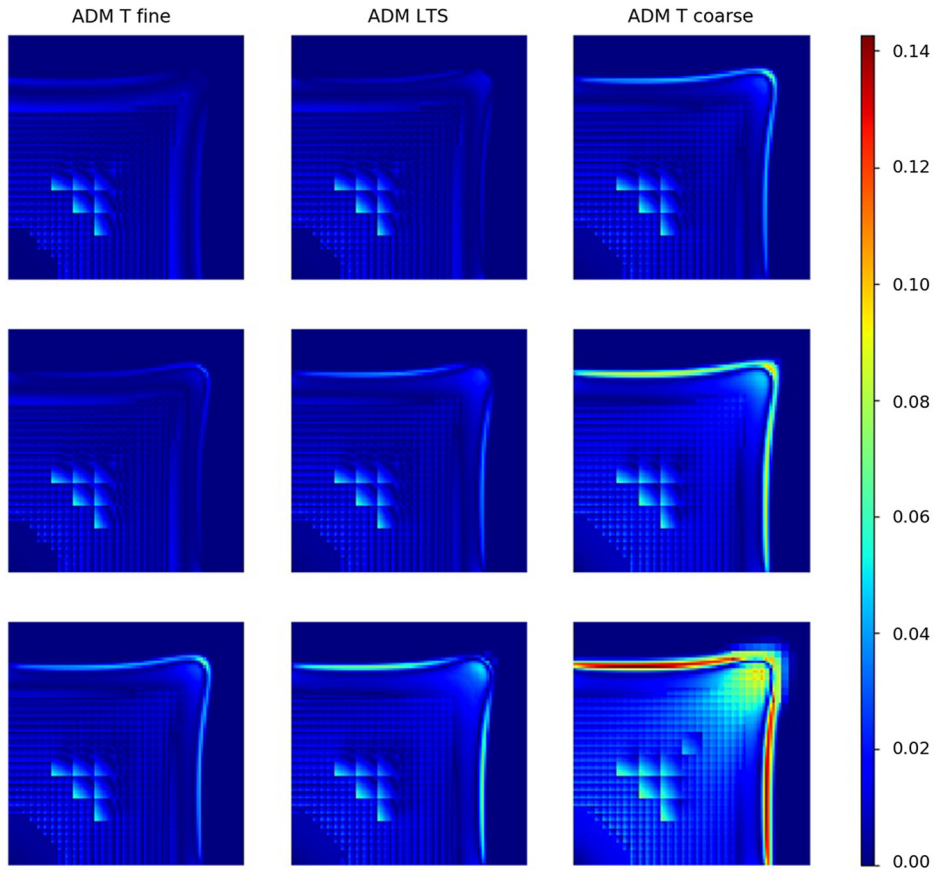
Fig. 5. Test case 1 [99 × 99] - Saturation errors for the ADM method with fine time steps (first column), ADM-LTS method (second column) and ADM coarse time steps method (third column) for the three different global time step sizes.
