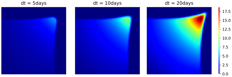
Fig. 3. Test case 1 [99 × 99] - CFL values for different global time steps at time t = 500 days.
