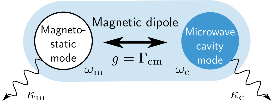
Fig. 5. The parameters in the interaction Hamiltonian (85) between a single cavity and magnon mode [17]. Here, the cavity has the frequency \omega_c and the dissipation rate \kappa_c ; the magnon mode, respectively, \omega_m and \kappa_m . The coupling rate is g \equiv \Gamma_{cm} .
