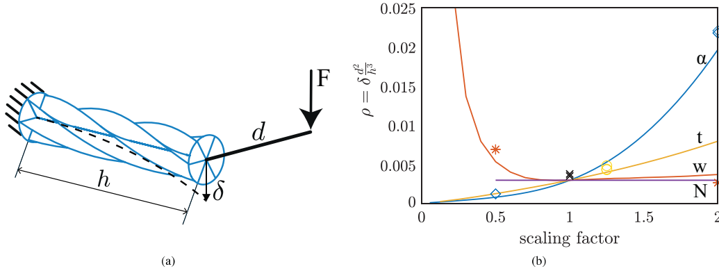
Fig. 6. The non-dimensionalised form of the lateral deflection \delta is plotted for the variations of the design parameters t , w , \alpha and N . The scaling factor parameter on the horizontal axis is defined as a multiplication with respect to the design parameter of interest in the standard design , namely t_0 , w_0 , \alpha_0 and N = 6 . The data represented by the solid lines is obtained by a finite element analysis of the helicoidal joints in a cantilever type loading condition. The scattered data points are obtained from experiments with equivalent loading conditions ( \circ = t , * = w , \diamond = \alpha , \times = \text{standard design} , N is not varied in experiments).
