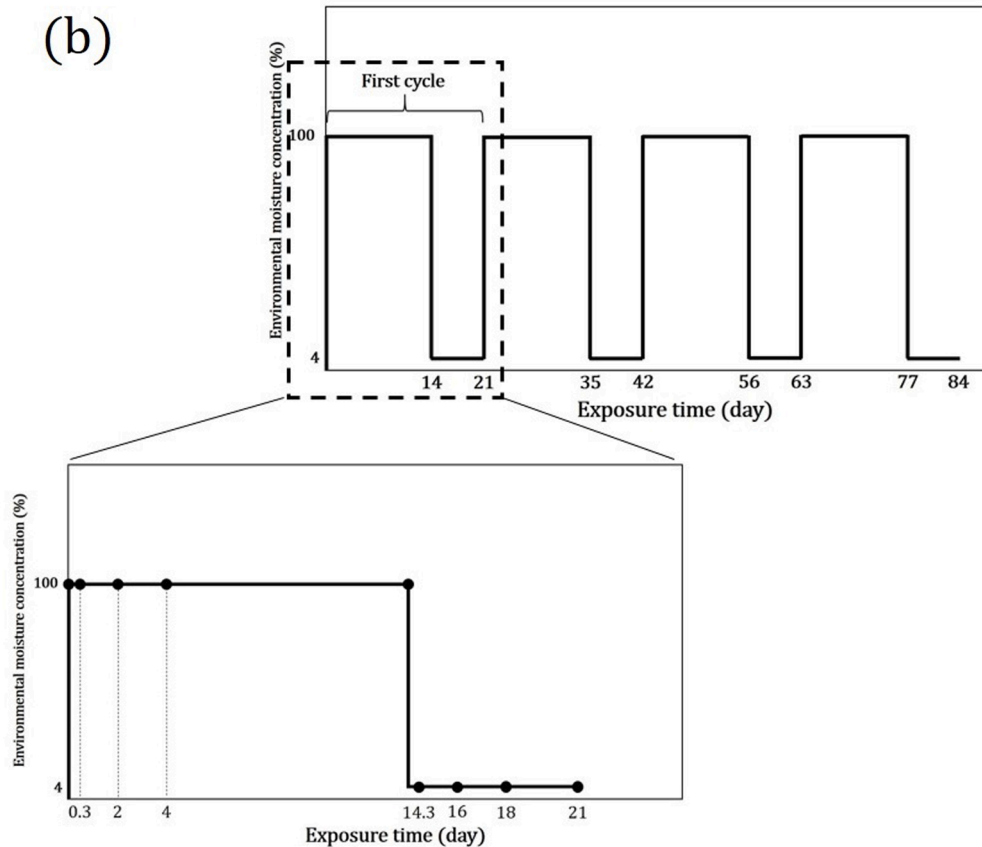
Fig. 2. Schematic representation of the aging conditions (a), aging cycles and exposure times considered for the ODCB specimens (b).
