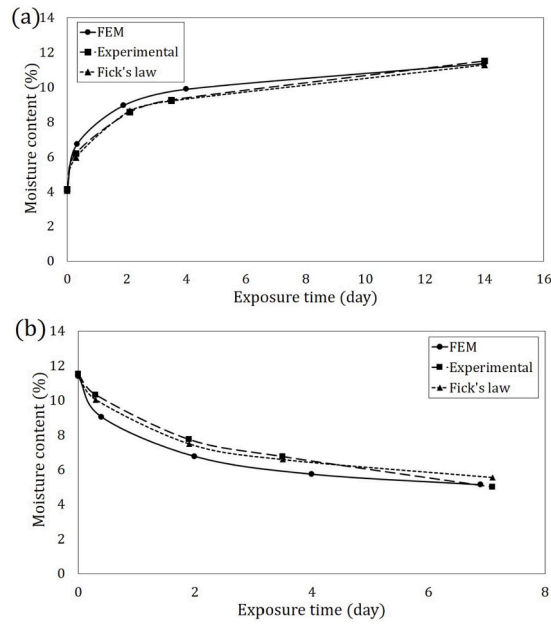
Fig. 20. Moisture contents obtained from different approaches in the second absorption (a) and desorption (b) processes.
