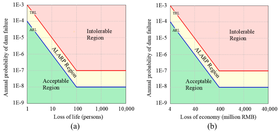
Fig. 5. Social risk criteria for cascade reservoir dams: (a) Loss of life; (b) Loss of economy.
