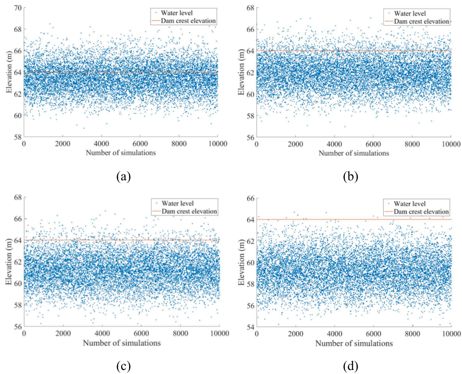
Fig. 13. Water level distribution of DTX Reservoir under different scenarios. (a) Successive dam failures of “Dahua-BLT-Letan-QG;” (b) Successive dam failures of “BLT-Letan-QG”; (c) Successive dam failures of “Letan-QG;” (d) Dam failure of QG reservoir.
