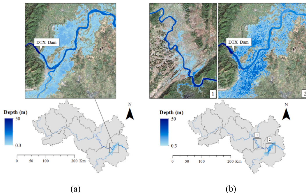
Fig. 14. Inundation area under different dam failure scenarios. (a) Dam failure of DTX reservoir; (b) Successive dam failures of "Dahua-BLT-Letan-QG-DTX".
