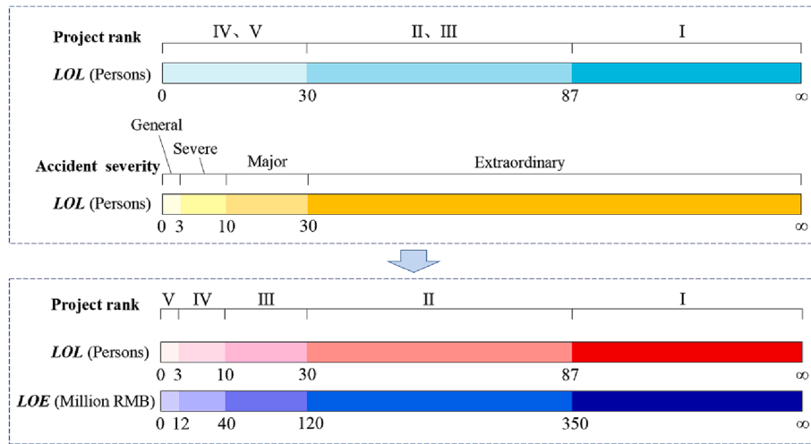
Fig. 7. Thresholds of dam failure losses corresponding to different project ranks.
