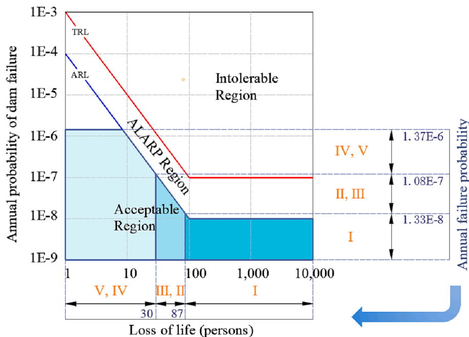
Fig. 6. Critical values of LOL corresponding to annual failure probabilities.
