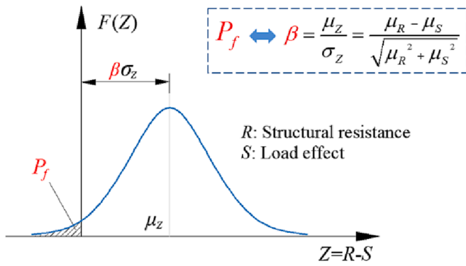
Fig. 3. Relationship between reliability index and failure probability.
