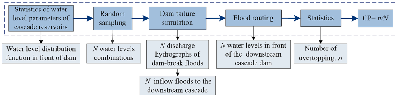
Fig. 10. Calculation of the CP of successive dam failure.
