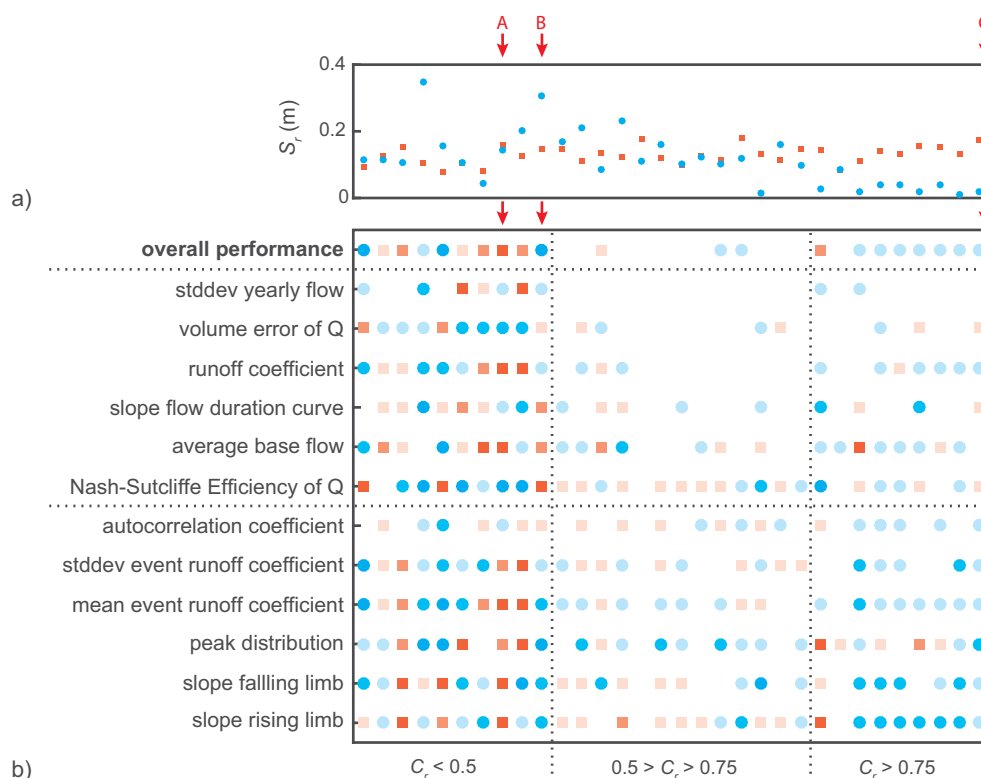
Figure 10. (a) Soil-derived (red squares) and climate-derived (blue circles) S_r , catchments are ordered by increasing runoff coefficient. (b) Overview of signature scores: blue circles and red squares indicate that a specific signature can be better reproduced with S_{r,clm} , respectively, S_{r,soil} for a specific catchment. Where no dots are shown, the performance difference for the specific signature between the two methods is smaller than 0.03. The shading of the symbols from dark to light indicates the degree of performance difference by using S_{r,clm} and S_{r,soil} . The performance differences are categorized by >0.5 (darkest), 0.2-0.5 (middle), 0.03-0.2 (lightest), <0.03 (no symbol). Signatures on top focus more on long-term water balance, while signatures at the bottom focus more on peak shape and height. The arrows indicate the catchments used in Figure 8.
