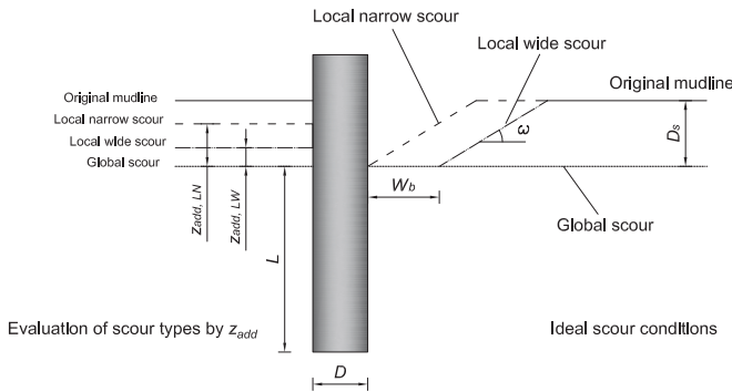
Fig. 14. Illustration of the additional soil depth ( z_{add} ).
