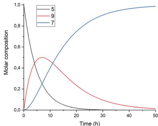
Fig. 3 Consumption of diamic acid 5 , formation and disappearance of reaction intermediate 9 and formation of PDI 7 according to eqn (5)–(7).
