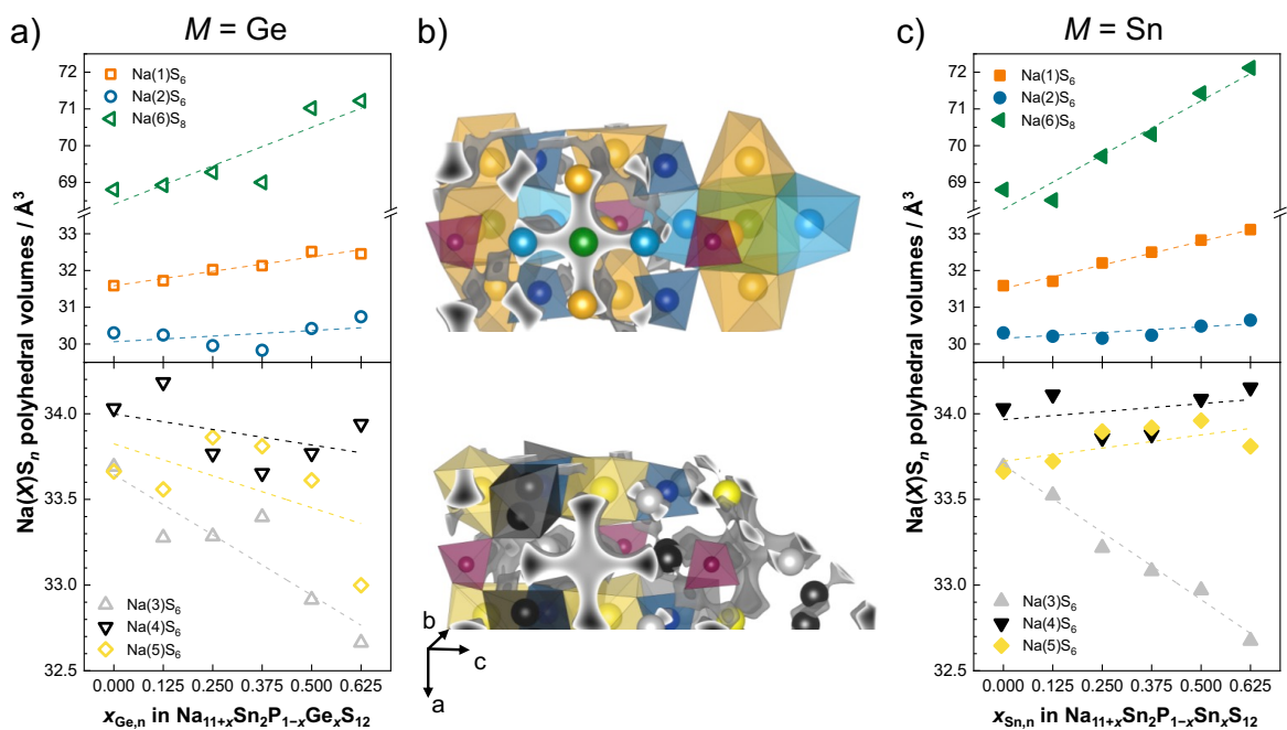
Figure 4: Volumes of the \text{Na}(X)\text{S}_n polyhedra building up the \text{Na}^+ diffusion pathways against the nominal x Ge and x Sn contents in \text{Na}_{11+x}\text{Sn}_2\text{P}_{1-x}\text{M}_x\text{S}_{12} . The \text{Na}(X)\text{S}_n polyhedra in b ) with their connectivity highlighted by the surfaces of equivalent bond valence site energies representing the energetically favored \text{Na}^+ diffusion pathways. Linear fits act as guide to the eye.
