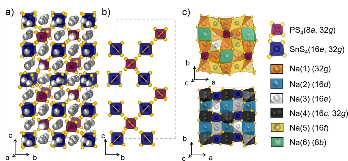
Figure 1: a) Crystal structure of Na 11 Sn 2 PS 12 , showing the Na + channels within the polyanionic backbone of SnS 4 4- and PS 4 3- tetrahedra. b) By depicting only half of those tetrahedra (Sn in front of P; Sn in x = 0.75 , P in x = 0.5 ) in the unit cell in the bc plane and highlighting the tetrahedral edges oriented towards the a -direction, the rotational ordering in b and c plane is presented. SnS 4 4- tetrahedra are rotated with respect to each other \sim 90^\circ along all three spatial dimensions leading to their faces oriented towards the PS 4 3- tetrahedra, which itself are rotated \sim 90^\circ with respect to each other in the c direction. c) The resulting Na-S polyhedra in this polyanionic backbone are shown in the two respective slabs of PS 4 3- ( z = 0.125 ) and SnS 4 4- ( z = 0 ) along the c -direction.
