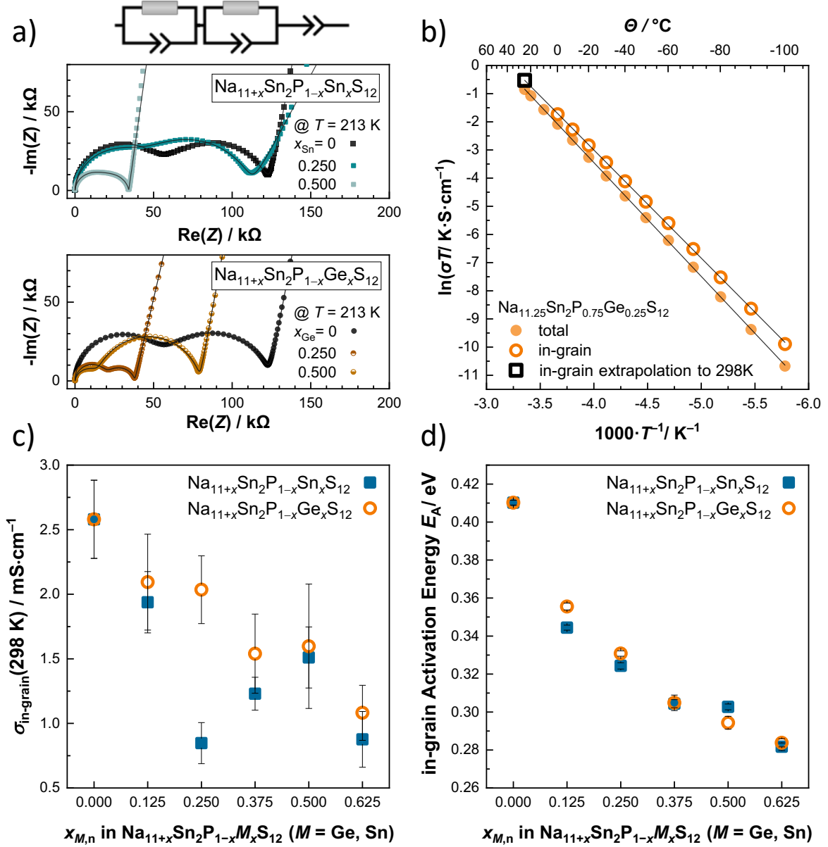
Figure 5. Nyquist representation of selected complex impedance spectra measured at 213 K ( -60^\circ\text{C} ) of \text{Na}_{11+x}\text{Sn}_2\text{P}_{1-x}\text{M}_x\text{S}_{12} ( M = \text{Ge}, \text{Sn} ) with x_M = 0, 0.25, 0.5 , fit (depicted as solid lines) with the displayed equivalent circuit representing contributions from in-grain and grain boundaries, respectively. b) Exemplary linearized Arrhenius representation of total and in-grain conductivities in \text{Na}_{11.25}\text{Sn}_2\text{P}_{0.75}\text{Ge}_{0.25}\text{S}_{12} for determination of respective activation energies E_A and extrapolation of in-grain conductivity to 298 K. The in-grain conductivity \sigma_{\text{in-grain}}(298 \text{ K}) in (c) as well as the in-grain activation energy E_A in (d) for \text{Na}_{11+x}\text{Sn}_2\text{P}_{1-x}\text{M}_x\text{S}_{12} ( M = \text{Ge}, \text{Sn} ) is shown as a function of x_M .
