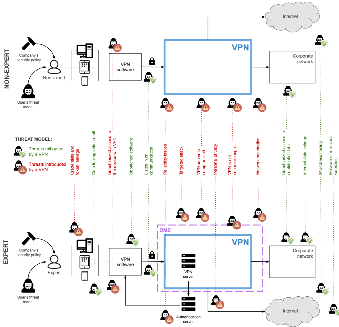
Figure 3: Mental models of experts/non-experts for VPNs along the dimensions of usage , threat modelling , and implementation . *In this figure we used icons by Chanut Industries , Font Awesome , Pixel Bazaar , Umar , DesignModo , RemixIcon , Altop Media , Nick Roach , Webdesigner Depot .
