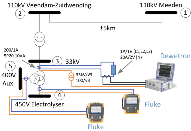
Fig. 4 Measurement setup at Veendam-Zuidwending
