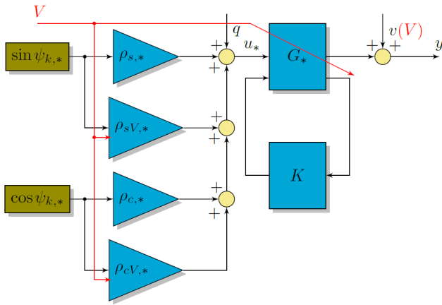
Figure 12. IFT implementation: wind turbine load control. Asterisk stands for IPC or individual flap control (IFC).
