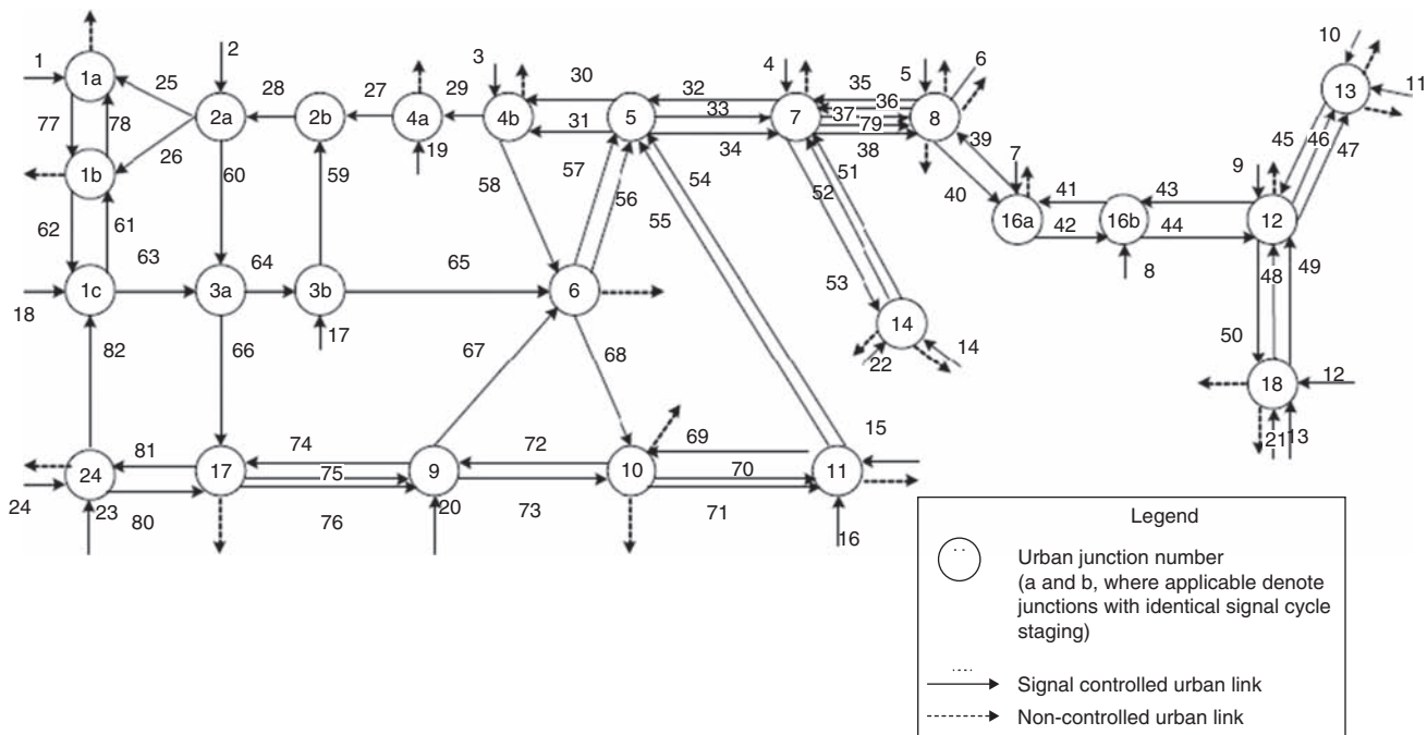
Figure 2. Schematic Map of Chania Traffic Network Showing Junction and Link Numbers
