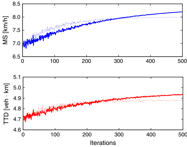
Figure 5. (Color online) Convergence of MS and TTD During P-CAO Iterations in Scenario 3: P-CAO L = 1 (Dotted) and P-CAO L = 2 (Solid) ( \delta_1 = 1 , \delta_2 = 1e-6 )
