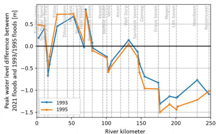
Figure 9: Water level differences between the measured peak water levels during the 2021 floods and the floods of 1993 and 1995. Many stations are missing because they did not exist in the 1990s, or have been demolished or relocated today.
