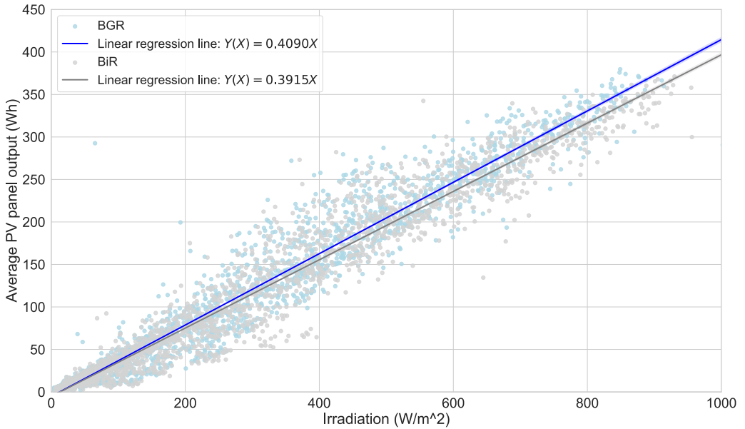
Figure 6.4 Linear regression results including a 95% confidence interval for the average PV panel output versus irradiation in Wm -2 for both the BiR) and BiR based on all hourly daytime data, outliers removed.
