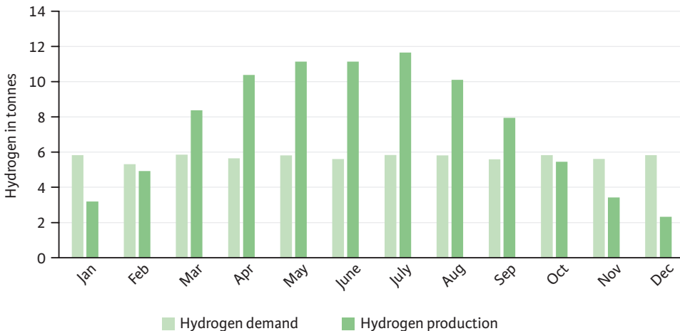
Fig. 2.10 Hydrogen demand and supply over a year for a Power-to-H 3 system with a supply of 540 cars, monthly average over five years.
