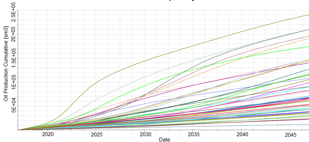
Fig. 25. Cumulative oil production over time in the production scenario F (200 m well spacing) for 50 different facies realizations
