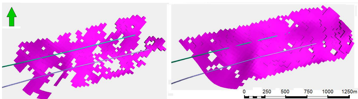
Fig. 38. Connected pore volume within the drainage area (cells in purple) for realizations 1000 (left) and 93000 (right)
