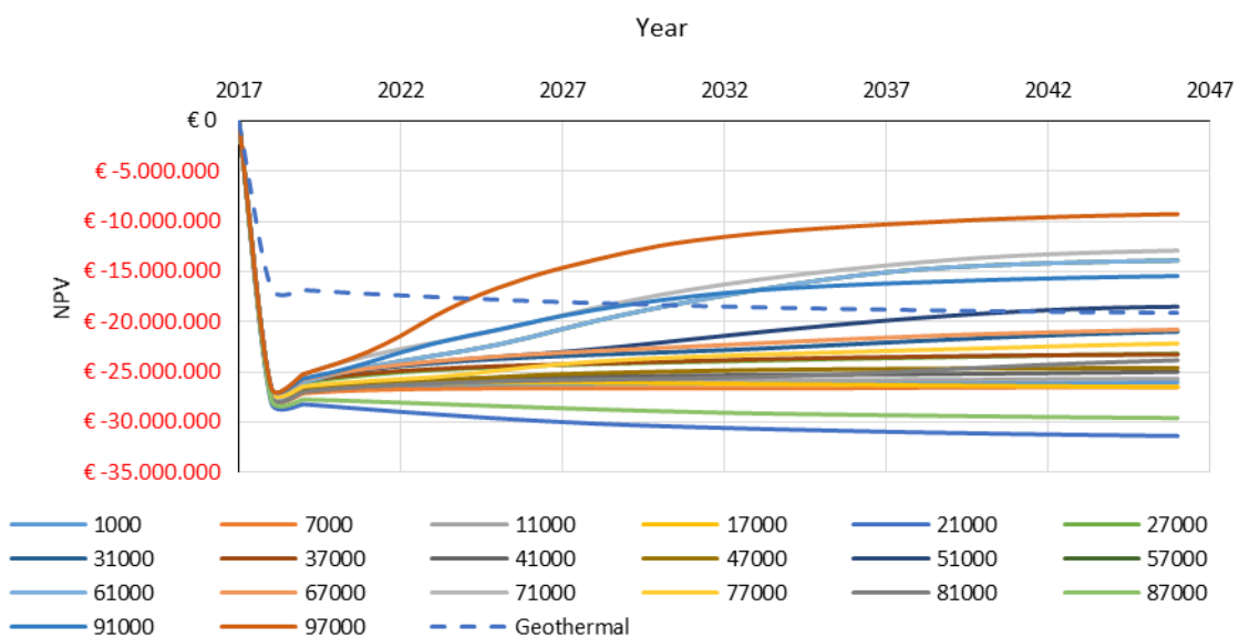
Fig. 27. NPV over time for different realizations in the production scenario F (Heterogeneous Reservoir Model) compared to the NPV of a single-doublet geothermal project
