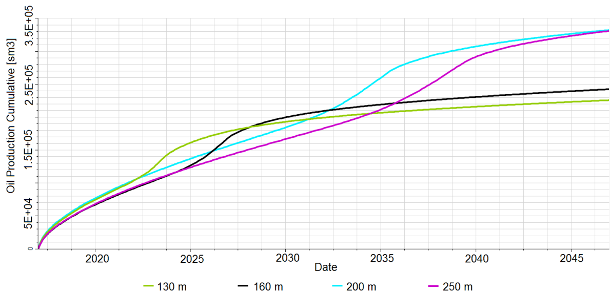
Fig. 18. Cumulative oil production over time for different well spacing in production scenario F
