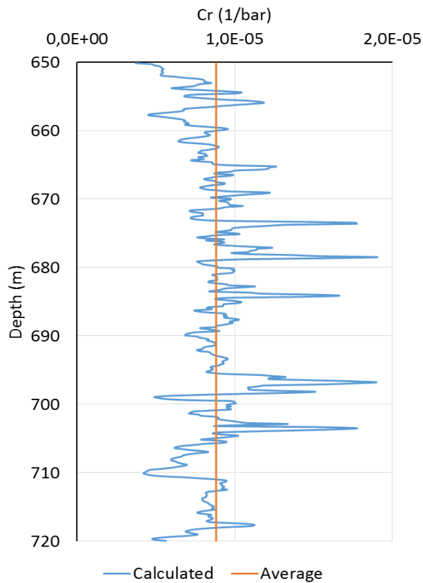
F.6. Calculated rock compressibility in well MKP-10
