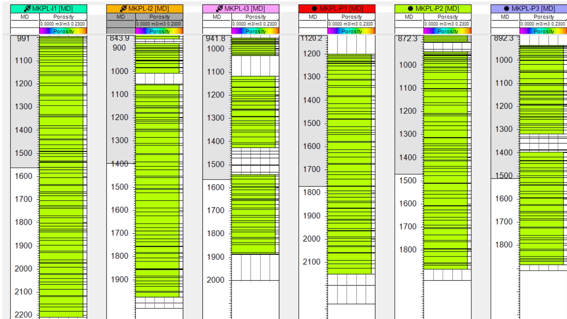
H.4. Reservoir penetration on wells for the 3 doublets scenario on the Homogeneous Simple Reservoir Model. Well productivity illustrated on H.1. appears not to be related with the well penetration within the reservoir
