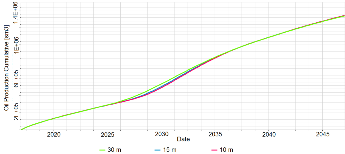
F.1. Cumulative Oil Production for different grid sizes on the Homogeneous Box Model (Scenario C). Differences between 10 m and 15 m grid are very subtle, meaning the results on the 15 m grid are numerically-accurate for a practical case
