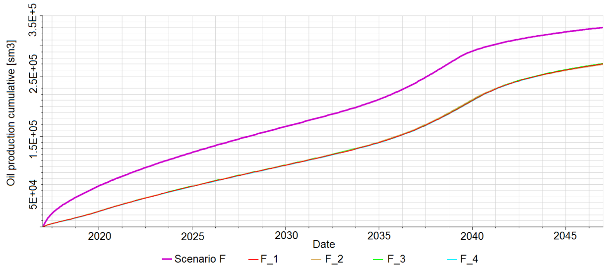
F.3. Cumulative Oil Production for different rock compressibility on the Homogeneous Simple Reservoir Model. Compressibility parameters summarized in F4
