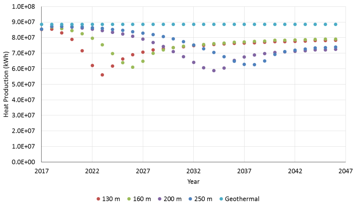
Fig. 19. Heat production profile (yearly) for different well spacing in the production scenario F compared with a stand-alone geothermal doublet with constant production rate of 150 sm 3 /day
