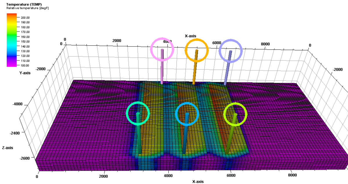
A.2. Reservoir Temperature for scenario D after 30 years. This scenario considers the performance of a single doublet in presence of more wells, even though the presented results are for wells in the middle (blue-injector and orange-producer). Dimensions in feet
