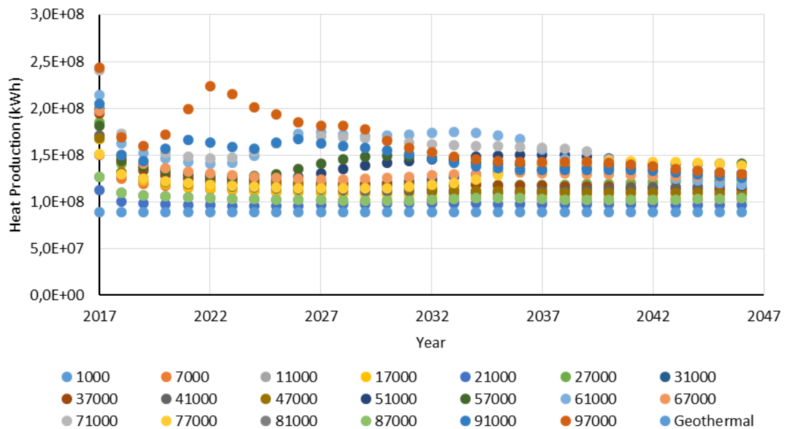
Fig. 28. Total energy production profile (yearly) for different realizations in production scenario F (Heterogeneous Reservoir model) compared with a stand-alone geothermal doublet with a constant rate of 150 sm 3 /day. The number of the realization indicates the seed used in the facies modelling for that specific case
