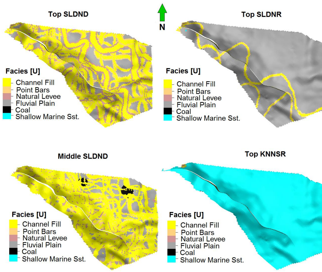
Fig. 9. Facies modelling for 4 different layers within the reservoir (Base case realization)
