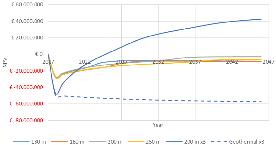
Fig. 21. NPV over time for different well spacing in the production scenario F compared with the up-scaled project, consisting of 3 producers and 3 injectors
