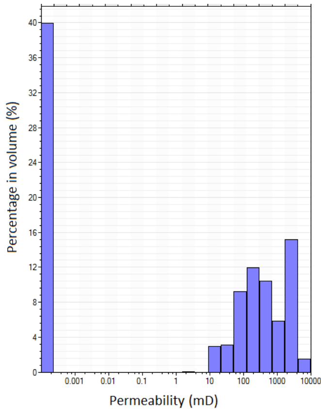
Fig. 13. Histogram (in volume) of the 3D populated permeability for the Base Case realization (Only SLDND). It can be seen that the N/G of only the SLDND is 60% (volume percentage of all the cells with permeability different than 0)
