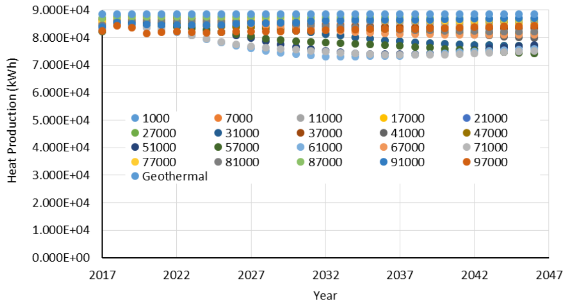
Fig. 26. Geothermal heat production profile (yearly) for different realizations in production scenario F (Heterogeneous Reservoir model). Results are compared with a stand-alone geothermal doublet with a constant production rate of 150 sm 3 /day. The number of the realization indicates the seed used in the facies modelling for that specific case
