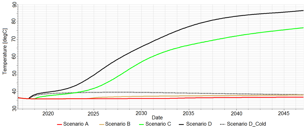
E.3. Fluid production temperature (production well). Approximately 10 years from the start of production the produced fluids (mainly water) could be used to generate heat for scenario D
