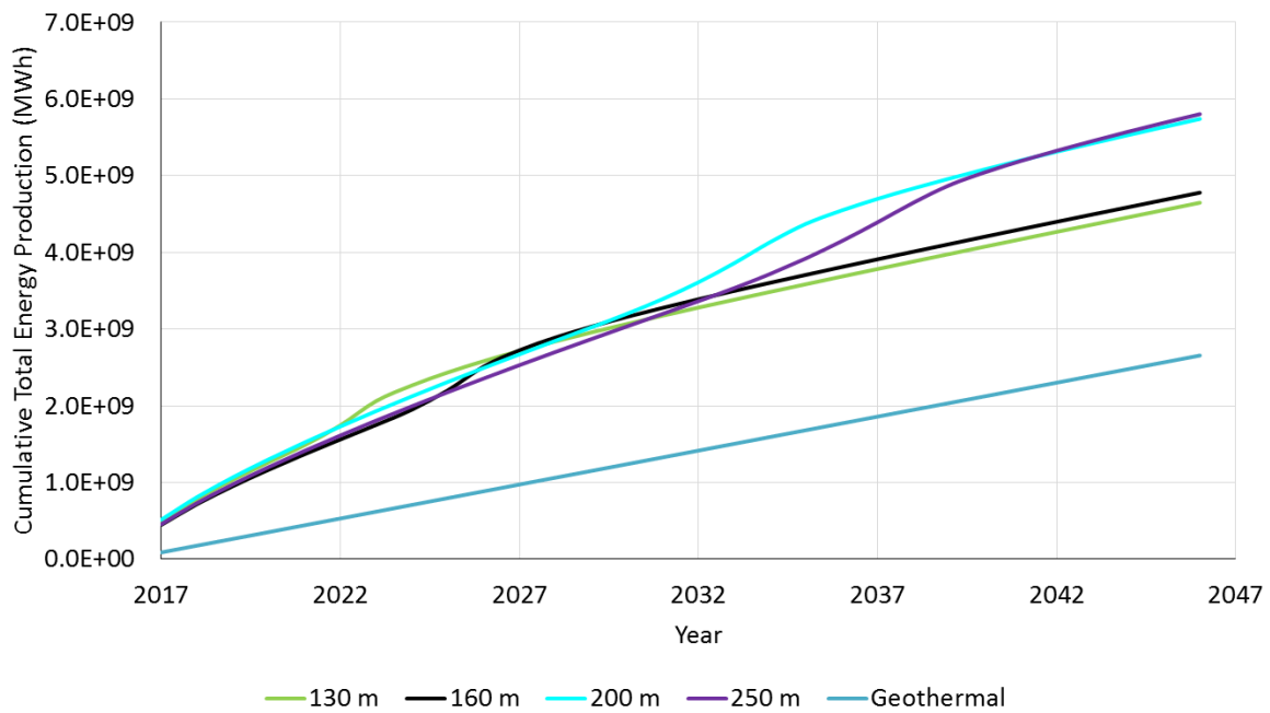
Fig. 23. Cumulative total energy production profile for different well spacing in the production scenario F compared with a stand-alone geothermal doublet with constant rate of 150 sm 3 /day. Delta in energy production is purely due to energy content of the produced oil
