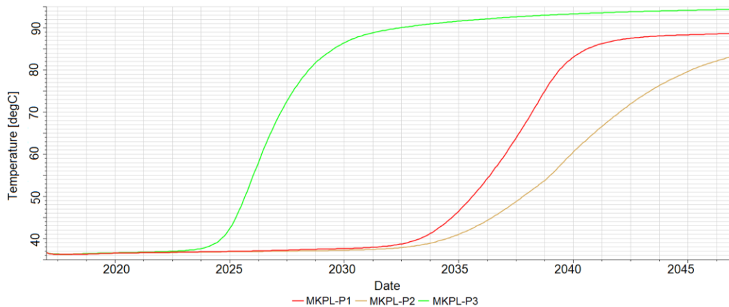
H.3. Fluid production temperature (production well) for different wells in the 3 doublets scenario for the Homogeneous Simple Reservoir Model
