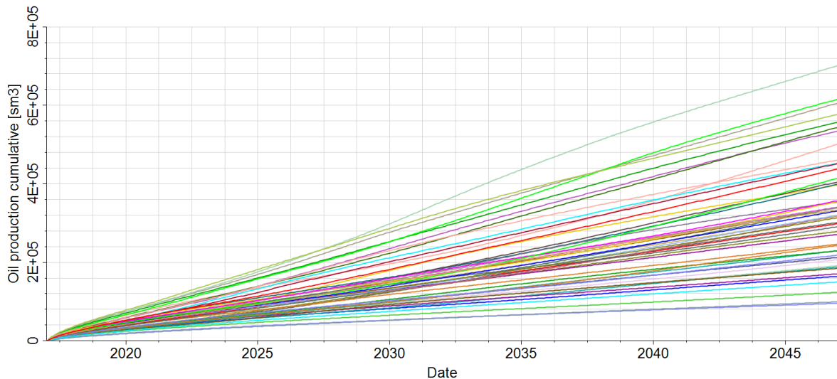
Fig. 30. Field cumulative oil production over time in the production scenario G (200 m well spacing – 3 doublets) for 50 different facies realizations
