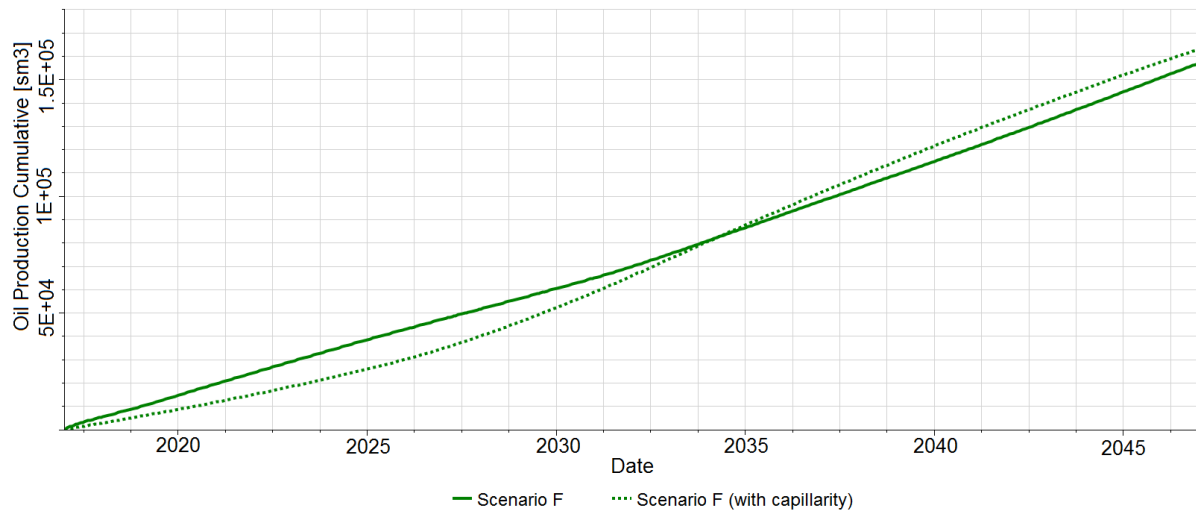
Fig. 24. Cumulative oil production over time in the production scenario F (200 m well spacing) with and without capillarity
