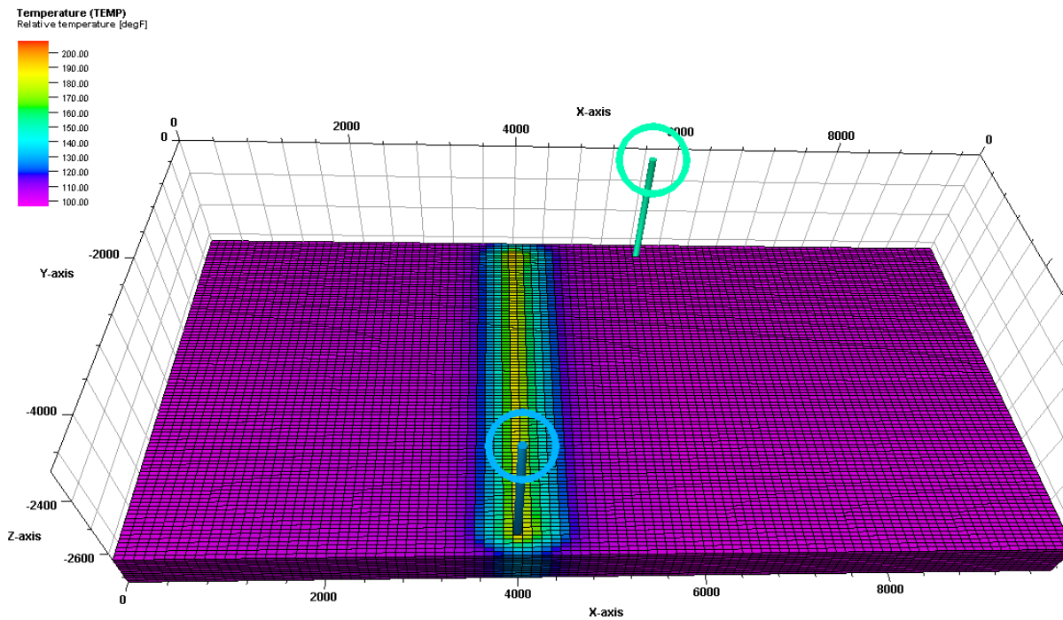
A.1. Reservoir Temperature for scenario B after 30 years. Thermal breakthrough does not occur in the production well (green), for this reason the well spacing was reduced for scenario C and subsequent scenarios. Dimensions in feet
