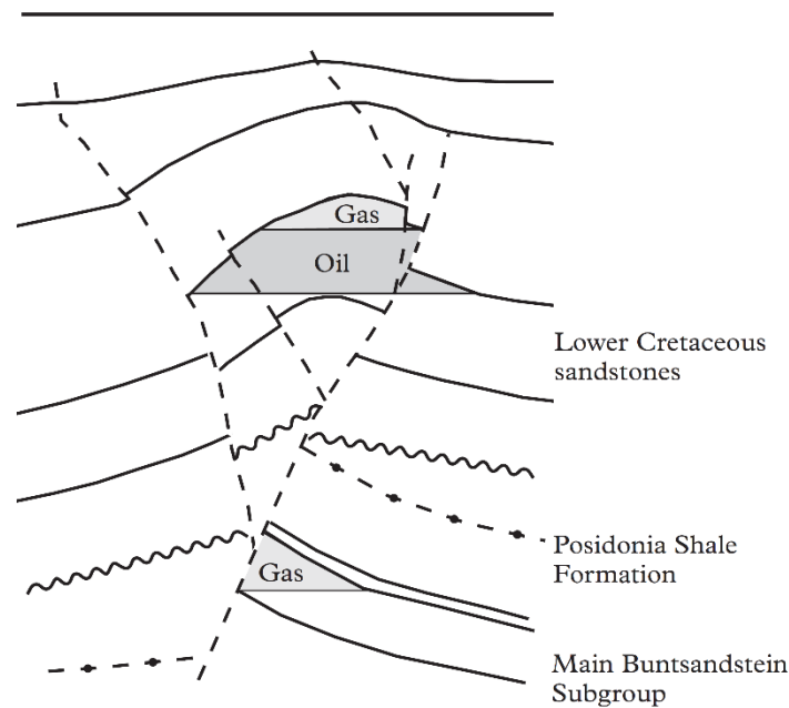
Fig. 4. Characteristic trap situation in the WNB. After van Balen et al. (2000)
