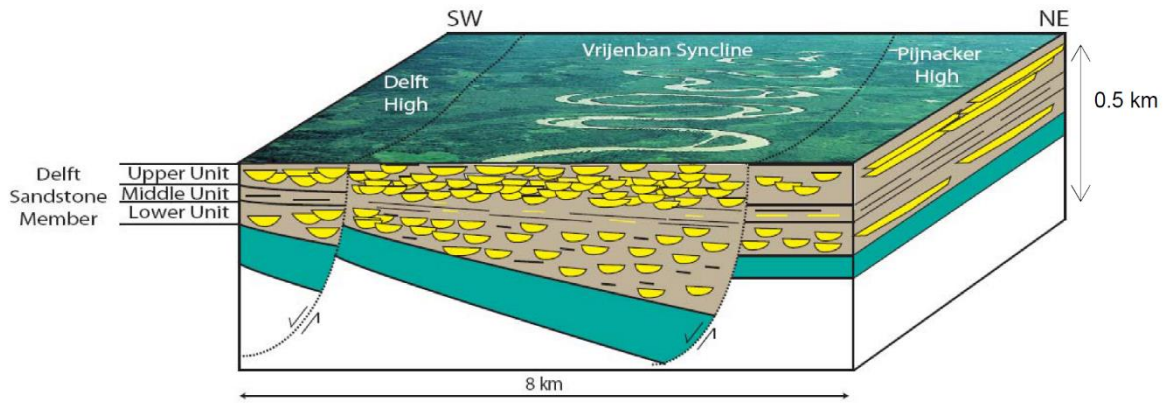
Fig. 3. Depositional model for the DSSM in the study area. After Gilding (2010)
