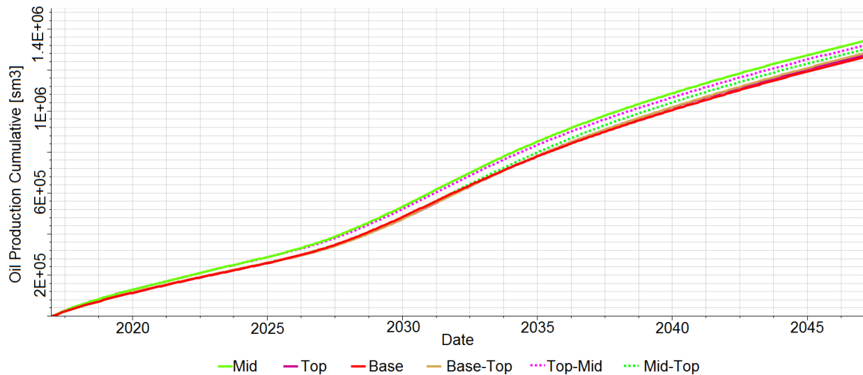
F.2. Cumulative Oil Production for different well placement within the reservoir on the Homogeneous Box Model. Mid: Injector & producer in the mid-reservoir. Top: Both wells at top cell of the reservoir. Base: Both wells at bottom cell of the reservoir. Base-Top, Top-Mid, Mid-Top: First word refers to injection well and second word to producer
