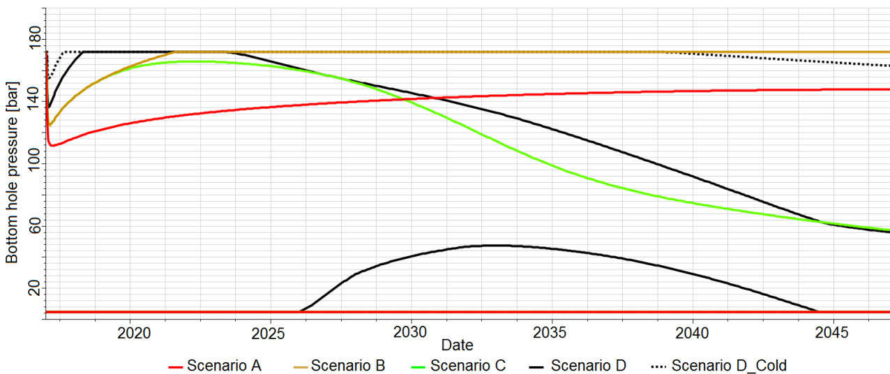
E.5. Well bottom hole pressures. High values correspond to injector wells whereas low values belong to production wells. Missing lines coincide with production pressure boundary condition (5.2 bar)
