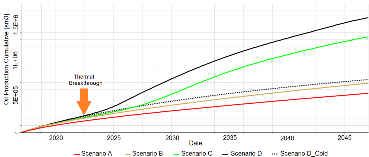
Fig. 15. Cumulative oil production from different scenarios in the homogeneous box model. (see Table 3 for more information on the scenarios)
