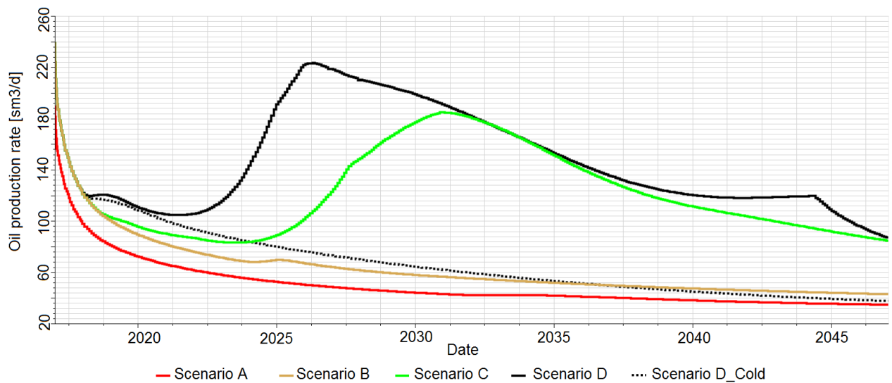
E.4 Oil production rates. High rates occur after water breakthrough
