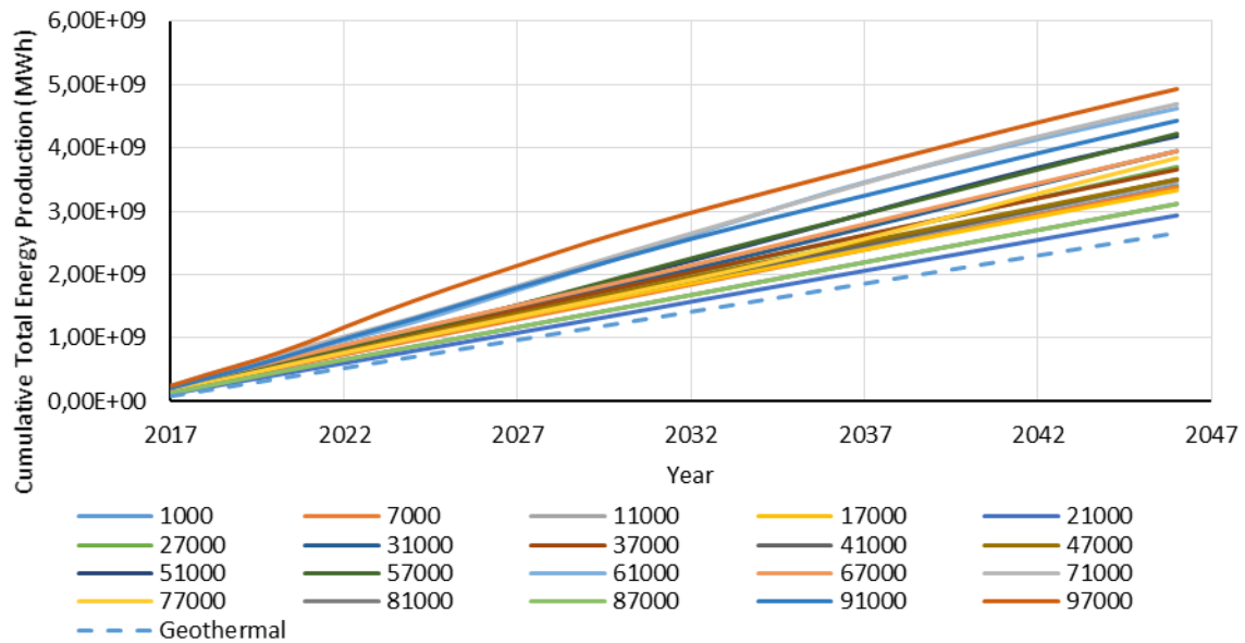
Fig. 29. Cumulative total energy production profile for different realizations in production scenario F (Heterogeneous Reservoir model) compared with a stand-alone geothermal doublet with a constant rate of 150 sm 3 /day. The number of the realization indicates the seed used in the facies modelling for that specific case
