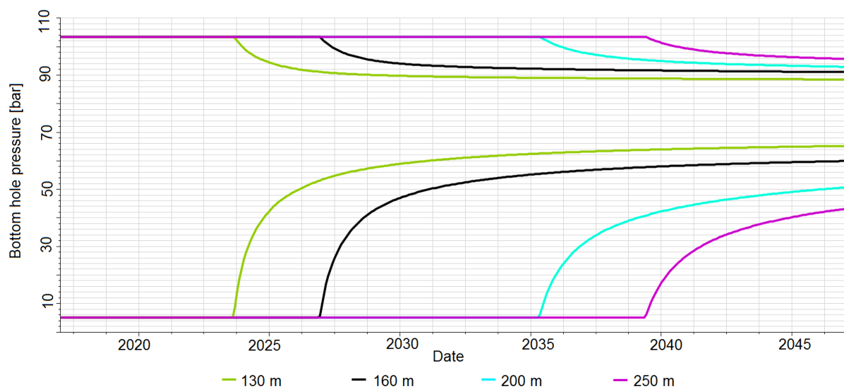
G.5. Well bottom hole pressures for different well spacing. High values correspond to injector wells whereas low values belong to production wells.
