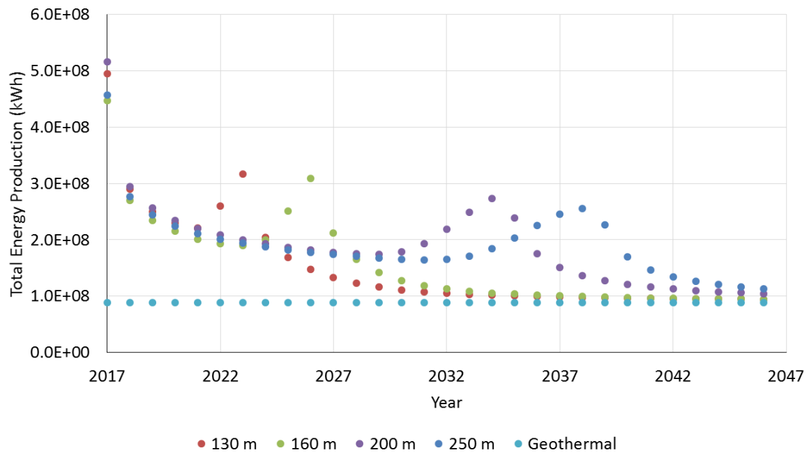
Fig. 22. Total energy production profile (yearly) for different well spacing in the production scenario F compared with a stand-alone geothermal doublet with constant rate of 150 sm 3 /day
