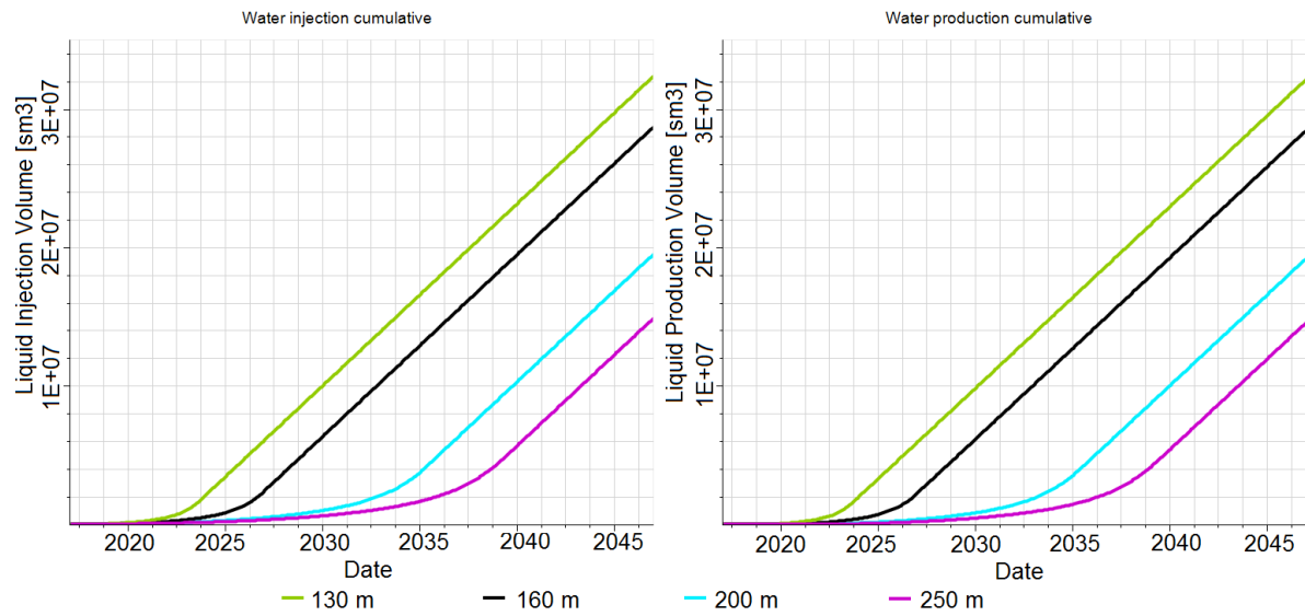
G.1. Cumulative water injection and production for different well spacing
