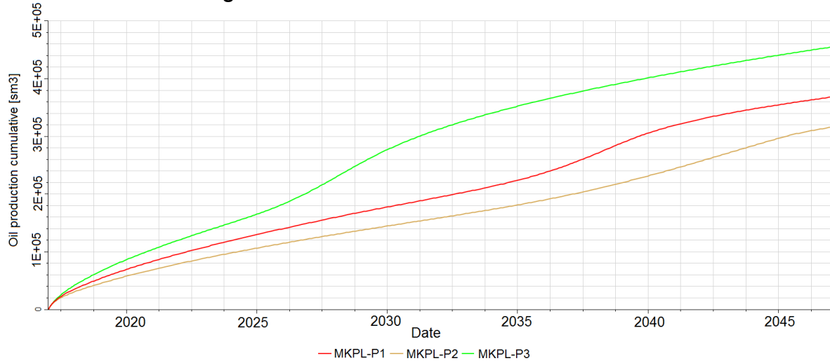
H.1. Cumulative oil production for different wells in the 3 doublets scenario for the Homogeneous Simple Reservoir Model
