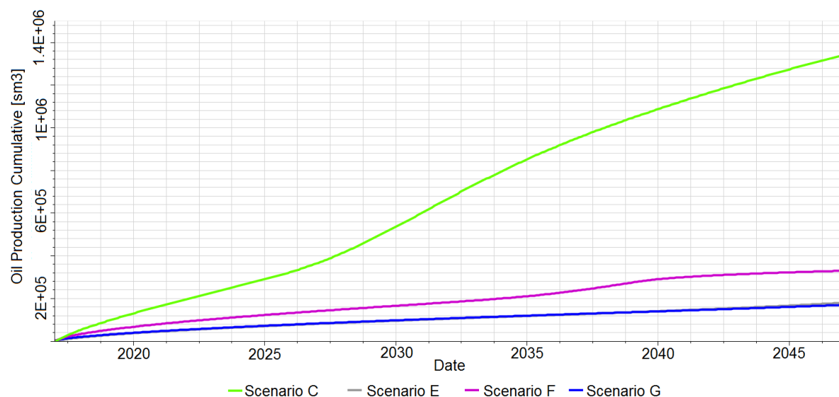
Fig. 17. Cumulative oil production from different scenarios in the homogeneous simple reservoir model, Second step . Scenario E almost coincides with scenario G
