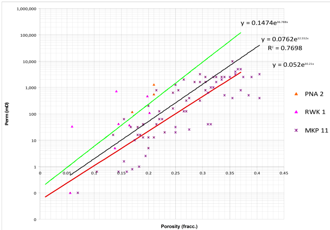
Fig. 12. Porosity- permeability relations for the Delft Sandstone in different areas. After Smits (2008). PNA: Pijnacker, RWK: Rijswijk, MKP: Moerkapelle
