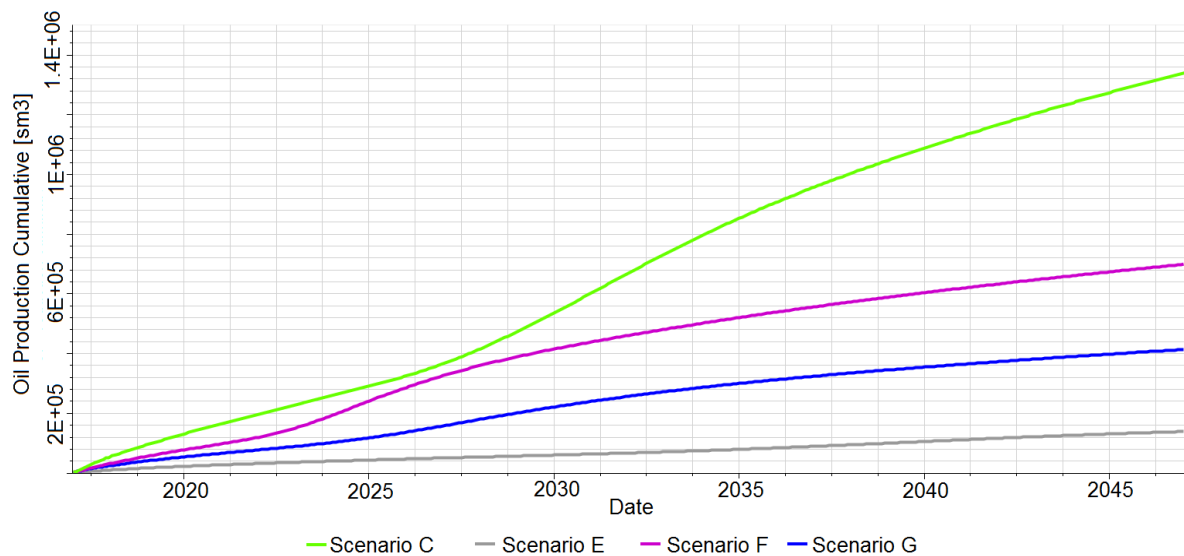
Fig. 16. Cumulative oil production from different scenarios in the homogeneous simple reservoir model, First step .
