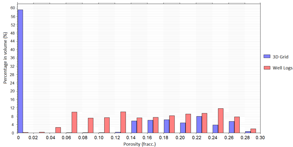
Fig. 11. Histogram (in volume) of the 3D populated porosity vs. Well logs porosity for the Base Case realization (KNNSR, SLDNR and SLDND). It can be seen that the N/G of the whole model is 40% (percentage in volume of all the cells with porosity different than 0 in the 3D grid)
