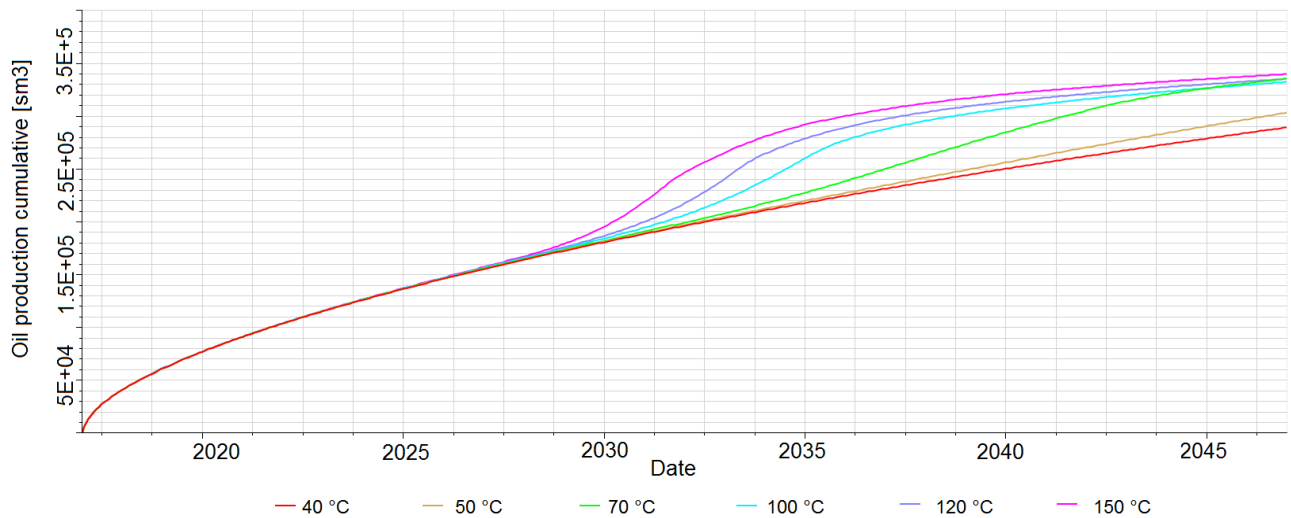
F.7. Cumulative Oil Production for different injection temperatures on the Homogeneous Simple Reservoir Model (scenario F)
