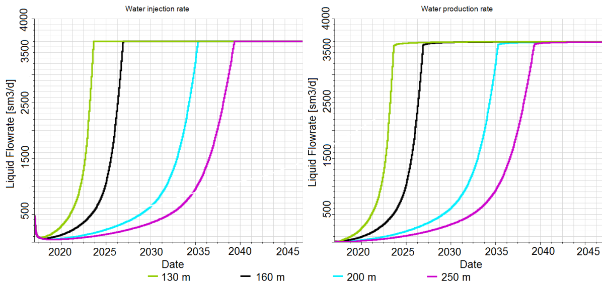
G.2. Water injection and production rates for different well spacing
