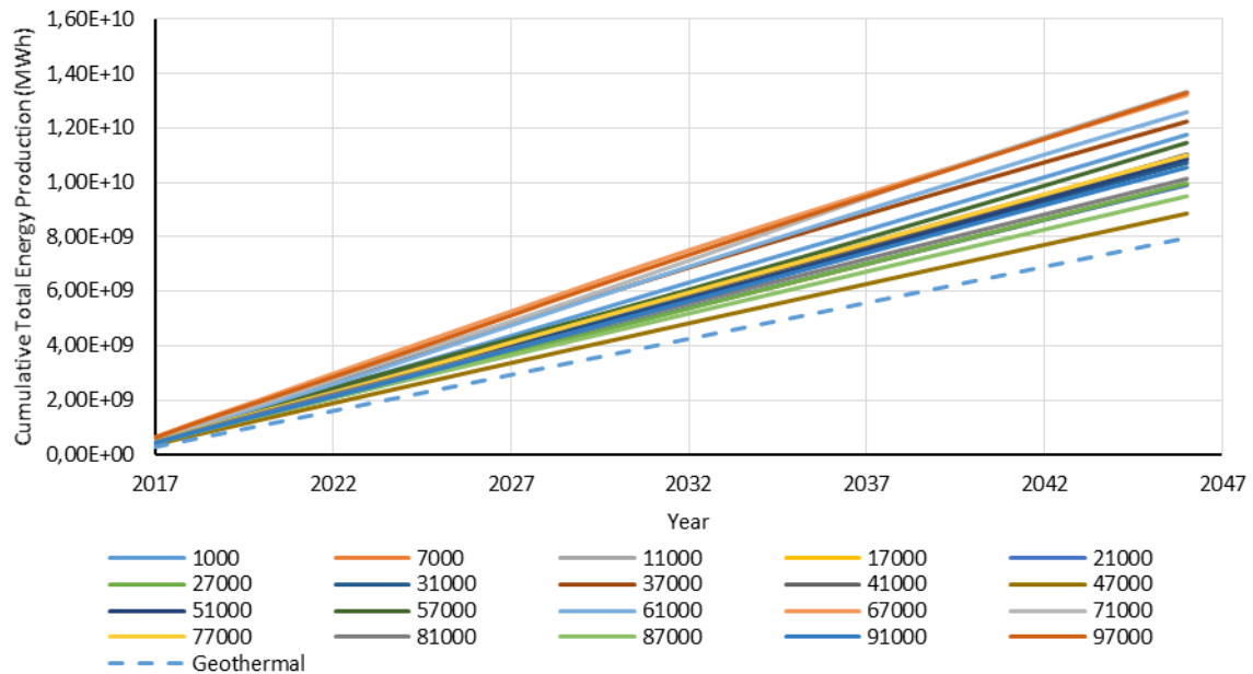
Fig. 34. Cumulative total energy production profile for different realizations in production scenario G compared with a stand-alone geothermal 3-doublets project with a constant rate of 150 sm 3 /day per doublet. The number of the realization indicates the seed used in the facies modelling for that specific case
