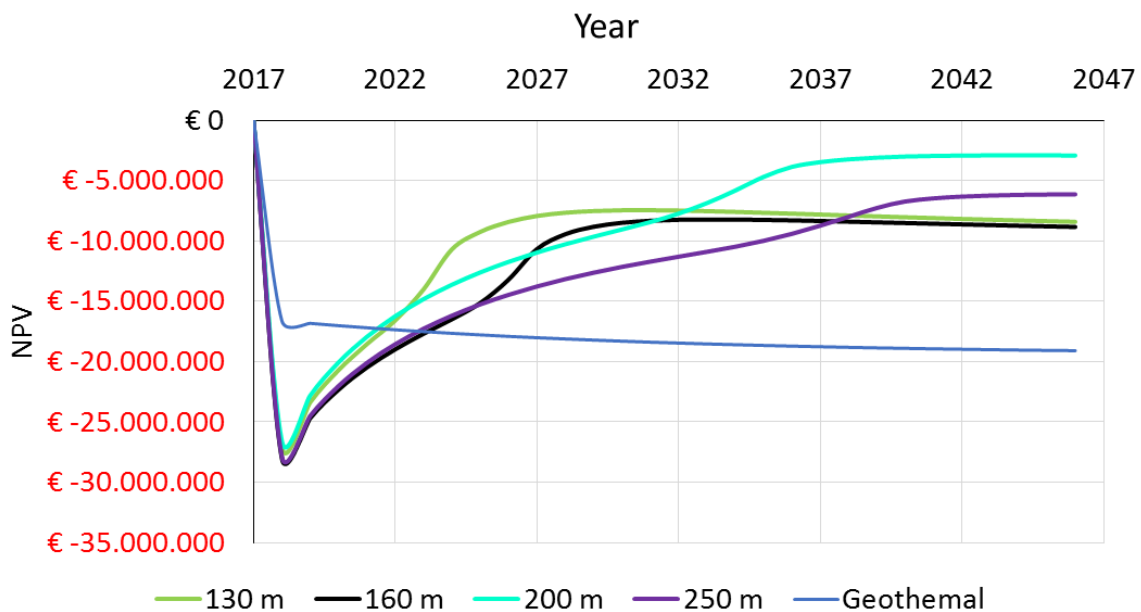
Fig. 20. NPV over time for different well spacing in the production scenario F compared to the NPV of a single-doublet geothermal project
