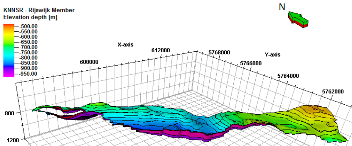
Fig. 7. Homogeneous Simple Reservoir Model for 3 zones. All values in meters
