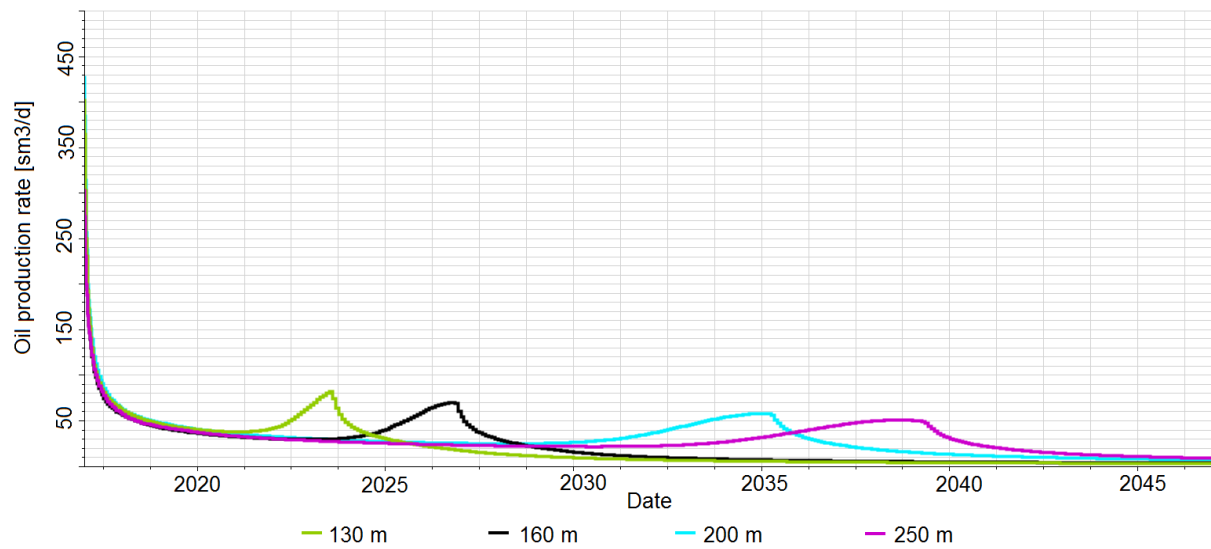
G.4 Oil production rates for different well spacing.
