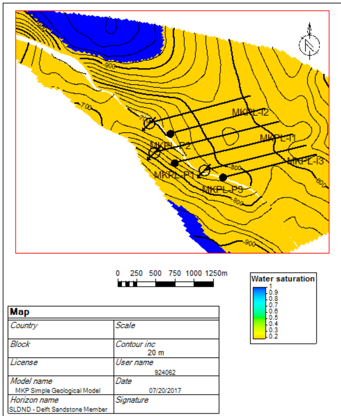
Fig. 14. Scenario G on Contour map for the top of DSSM (SLNDND). Colors in the map represent water saturation (oil saturation is yellow). One pattern with three doublets (scenario G) is illustrated by black continuous lines
