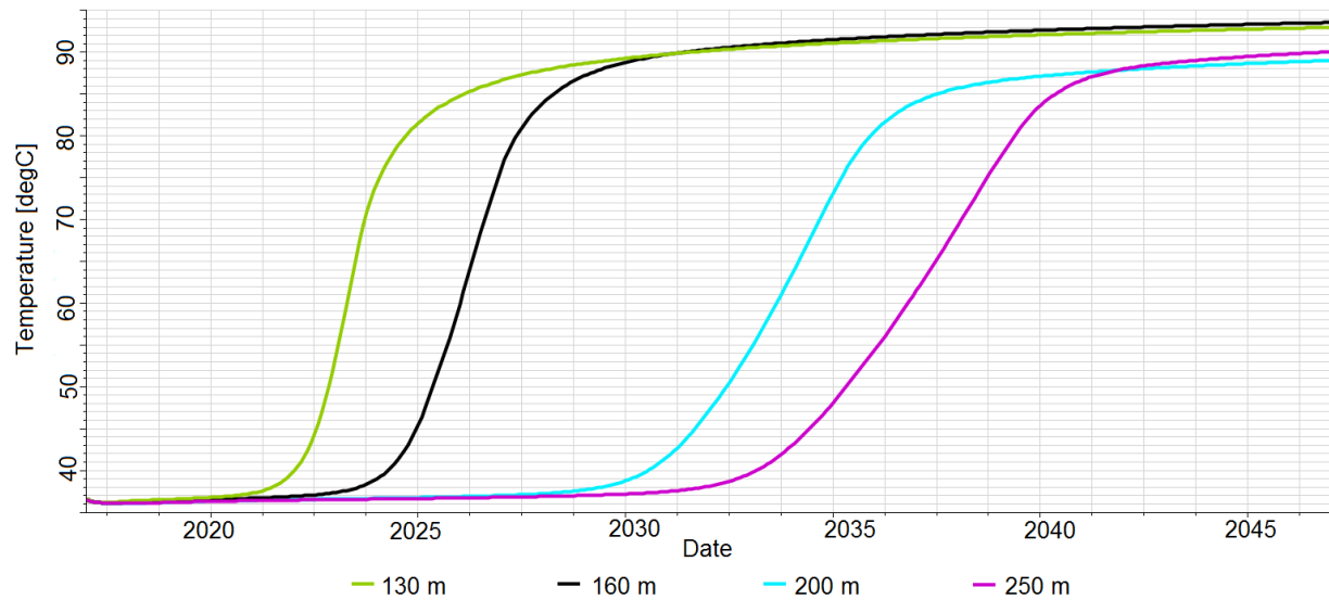
G.3. Fluid production temperature (production well) for different well spacing
