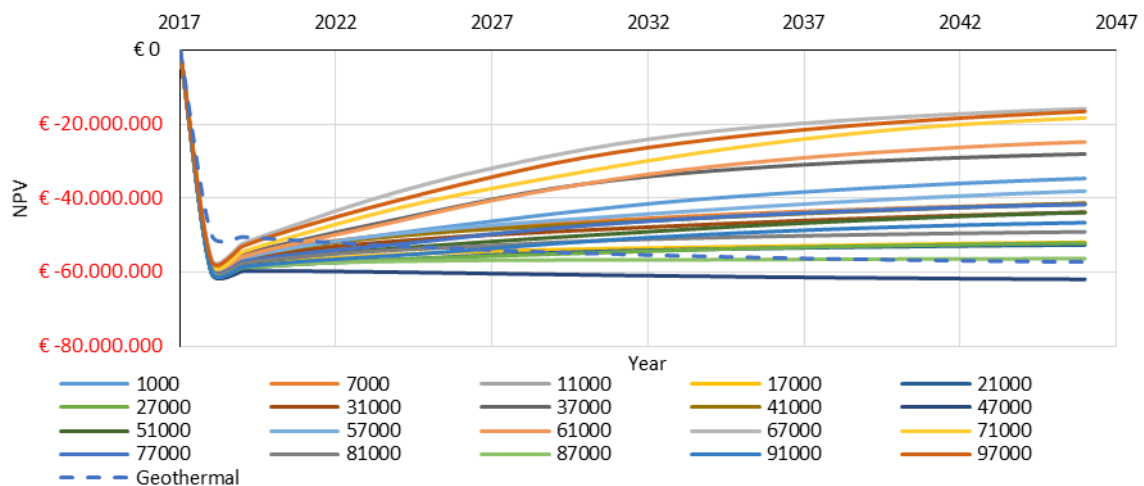
Fig. 32. NPV over time for different realizations in production scenario G (Heterogeneous Reservoir Model) compared to the NPV of a 3-doublets geothermal project
