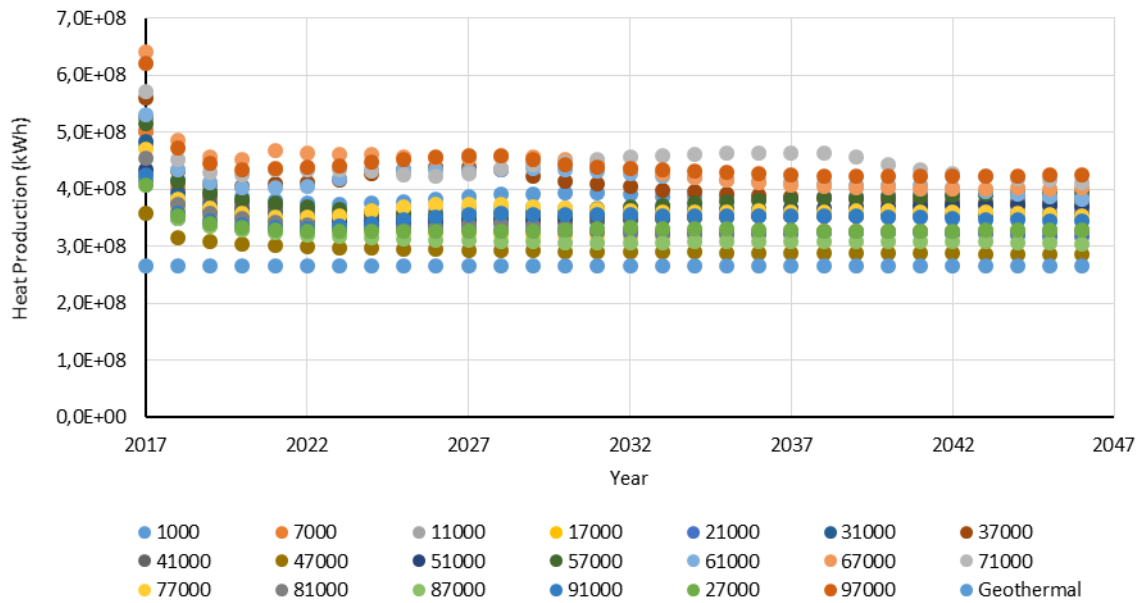
Fig. 33. Total energy production profile (yearly) for different realizations in production scenario G compared with a stand-alone geothermal 3-doublets project with a constant rate of 150 sm 3 /day per doublet. The number of the realization indicates the seed used in the facies modelling for that specific case
