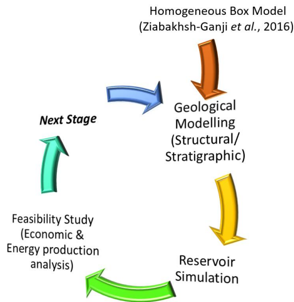
Fig. 5. Flowchart illustrating the methodology used during the project. The starting point is an homogeneous box model constructed by Ziabakhsh-Ganji et al. (2016)
