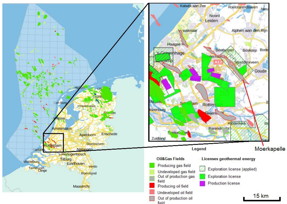
Fig. 1. (Left) Map of the Netherlands oil and gas fields. (Right) Location of the Moerkapelle field within the WNB (Modified after TNO, 2016)
