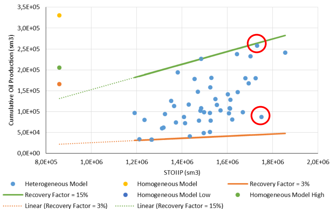
Fig. 36. Dependency of the cumulative oil production on the STOIIP within the drainage area. The drainage area is defined as a 200 m radius from the wells (injector and producer). Red circles highlight the cases selected for analysis in Figs. 36 to 38, represent similar STOIIP with very different recovery factors (high case: realization 93000, low case: realization 1000). Homogeneous Model High ( k=460 mD) and Homogeneous Model Low ( k=312 mD)
