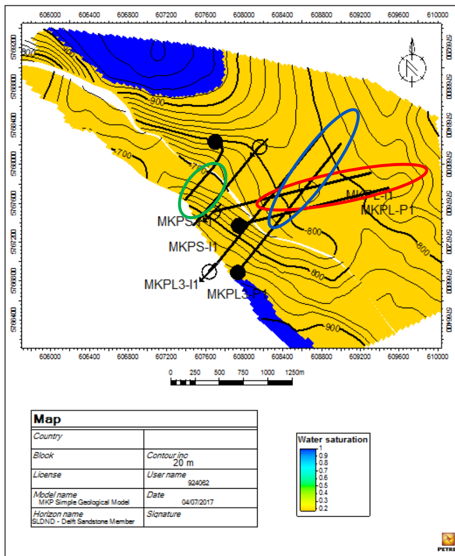
Fig. 8. Scenarios in Stage 2 on a contour map for the top of DSSM (SLNDND). Colors in the map represent water saturation (oil saturation is yellow). Three groups of wells (doublets) with different orientations are illustrated by black continuous lines and their areas of influence are circled in different colors; those correspond to the three production scenarios summarized in Table 5 (Green: Scenario E, Red: Scenario F, Blue: Scenario G)
