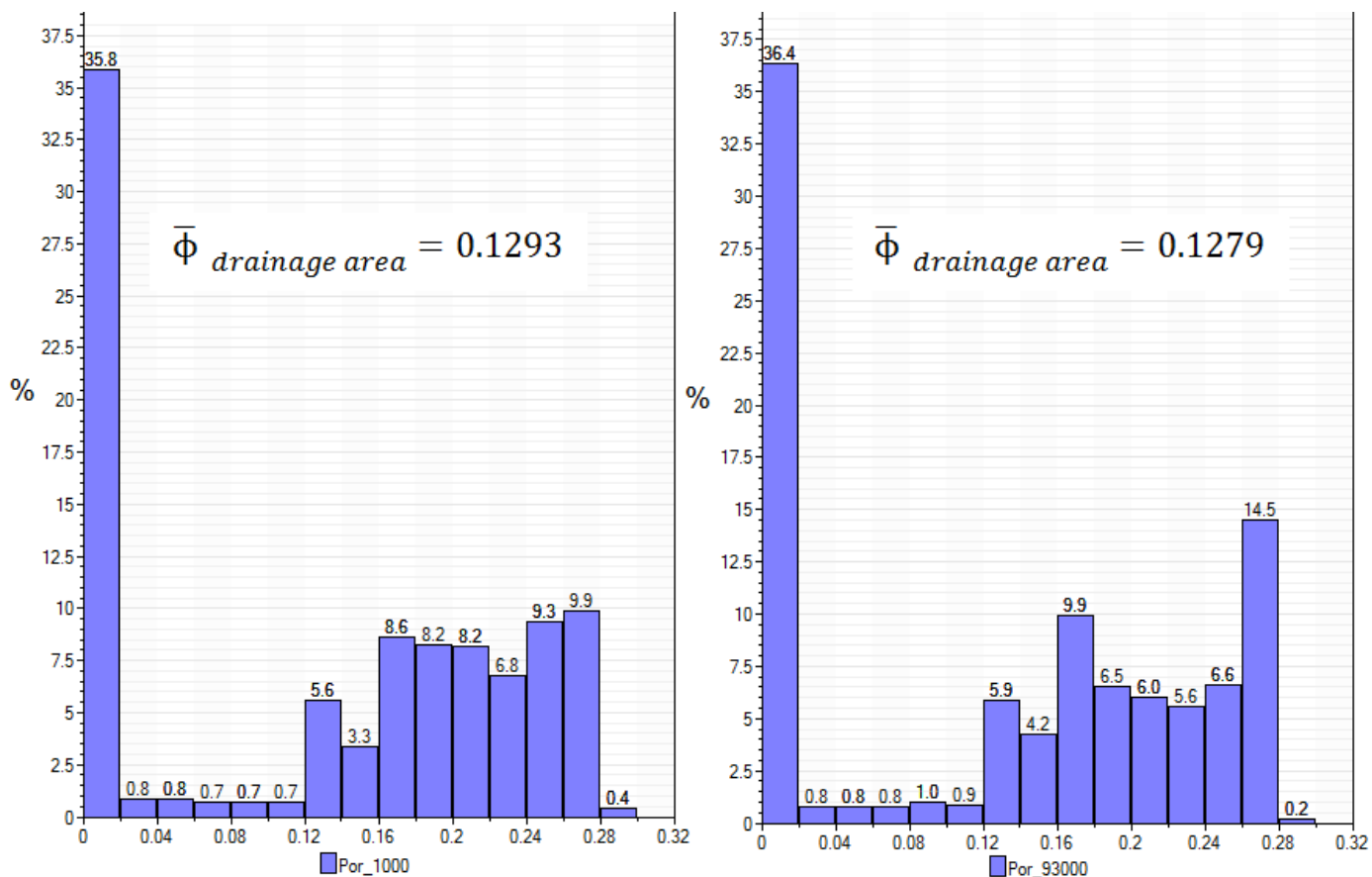
Fig. 37. Histogram (in volume) of the porosity in the drainage area for realizations 1000 (left) and 93000 (right)
