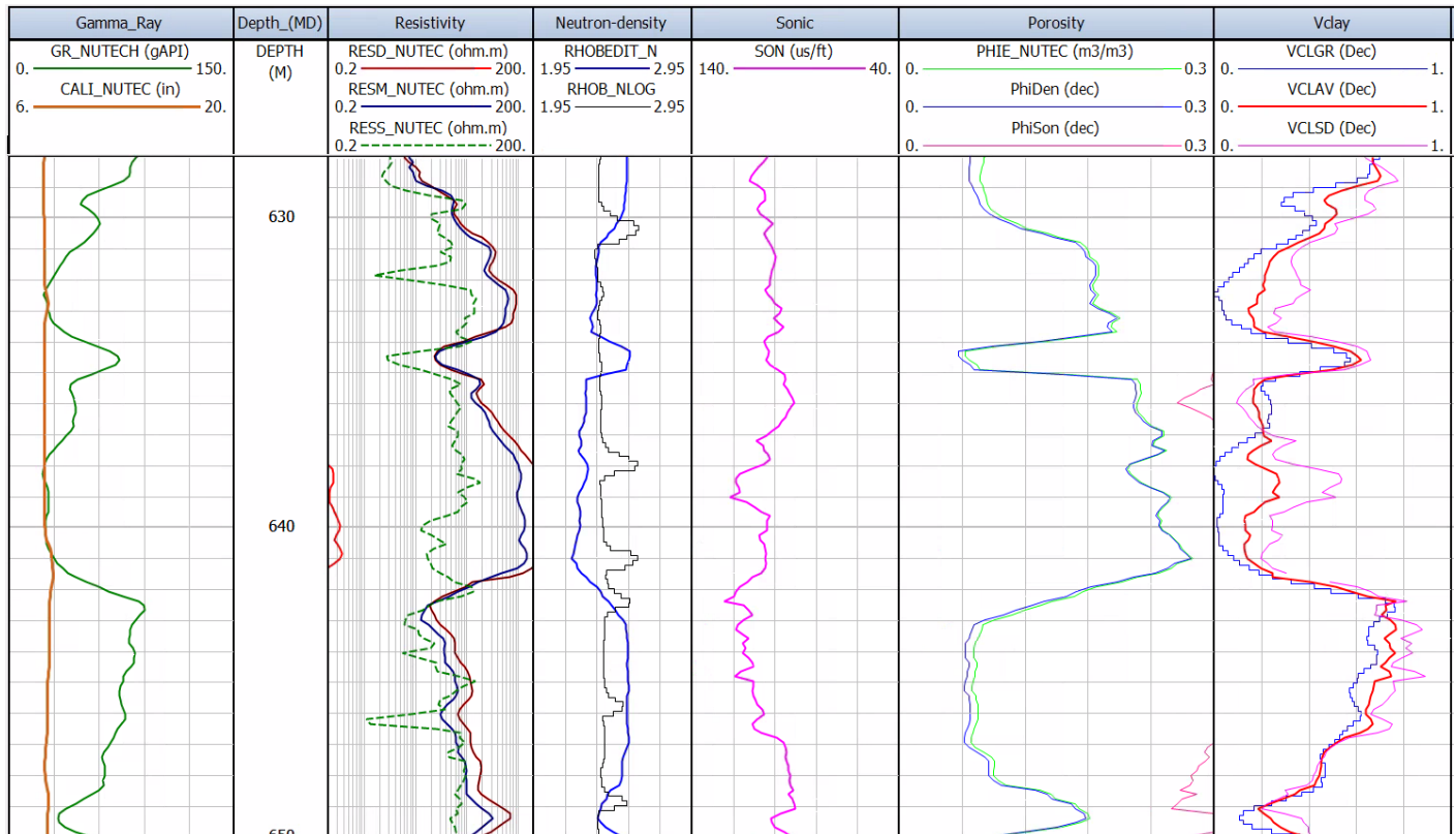
Fig. 10. Example of the results of the calculation of porosity and clay volume in Interactive Petrophysics (IP) software (Well MKP-10)
