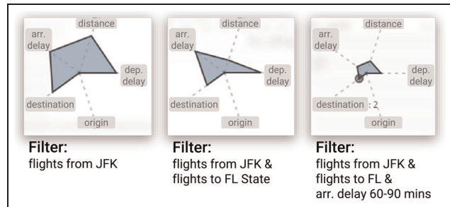
Figure 4. Connector plot. This is a starplot where each “arm” indicates the value range on the corresponding data attribute. The data shown is drawn from a flight delays dataset. With progressive filtering of data, the plot shrinks to reflect the reduction in the number of annotations in the group, as the range associated with attributes decreases.
