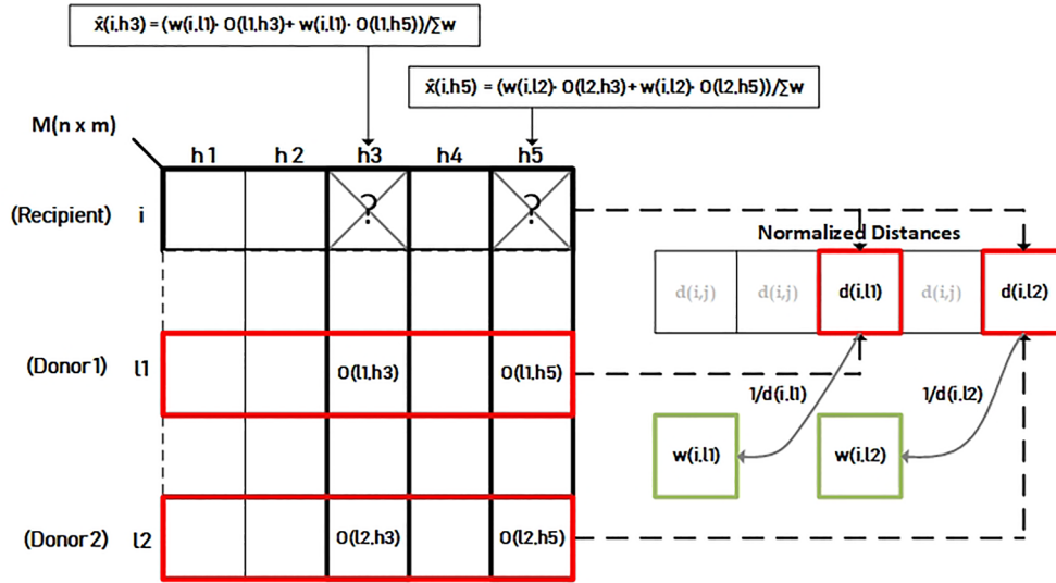
Fig. 5. k-NN imputation technique illustration for k = 2 . h_m = feeders, i, l_k = time.
