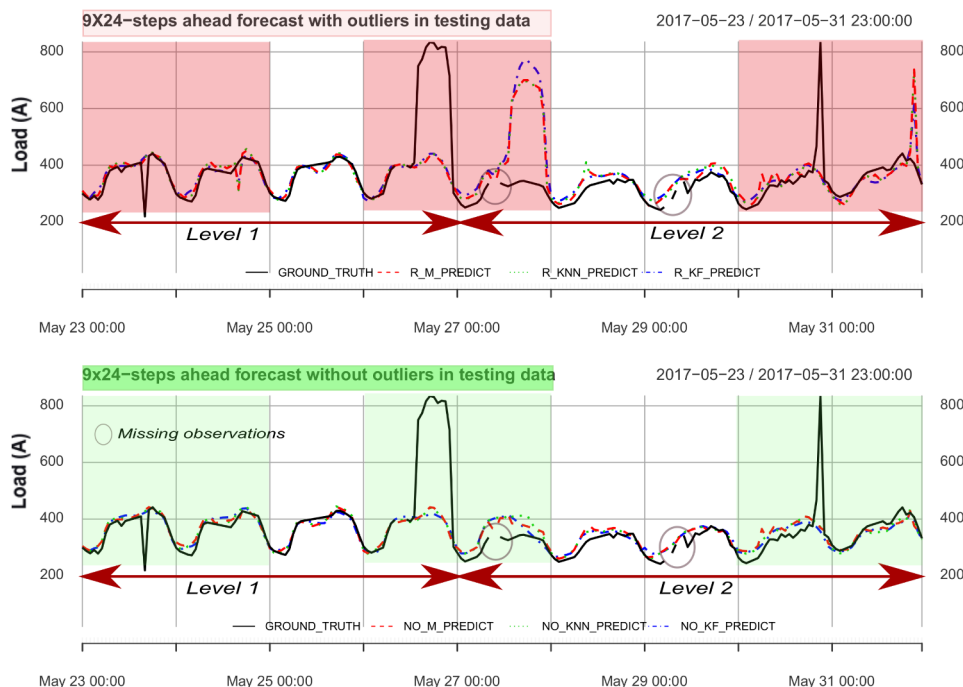
Fig. 9. 9 × 24-steps-ahead forecasts. Testing data contain outliers (top) while outliers are removed and missing value are imputed.
