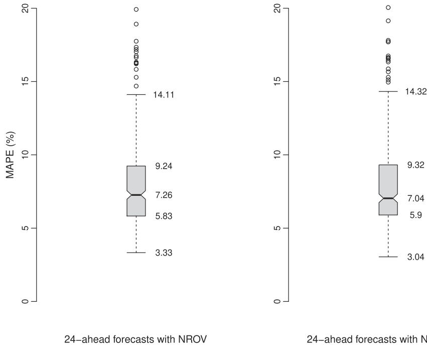
Fig. 7. Statistics for the performance of 24-steps ahead forecast across 342 MV feeders using (1) Nested Rolling-Origin Validation (NROV) on the left and (2) Nested Adjusted-k-fold Validation (NAK-foldV) on the right (NO_KNN dataset).
