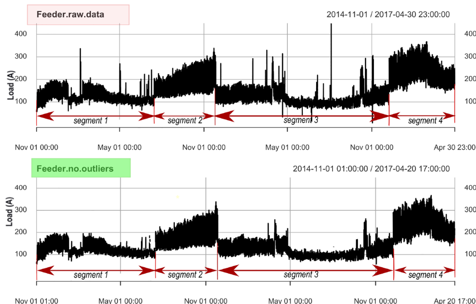
Fig. 2. Outliers detection/removal with BS-Tukey for Feeder 3 data which contain multiple structural breaks – top plot(before detection), bottom plot(after detection).
