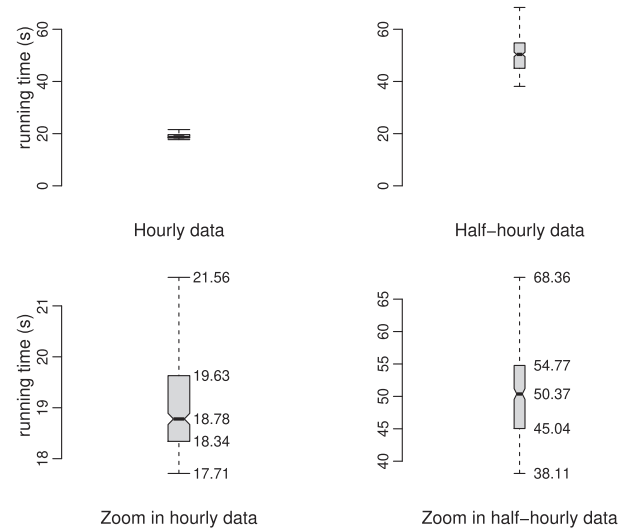
Fig. 3. Running time statistics of the automatic outlier detection across 342 feeders for half-hourly data (43,282 samples each) and hourly data (21,641 samples each).
