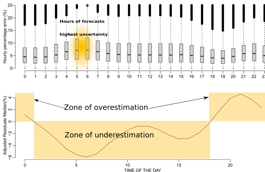
Fig. 10. Hourly analysis of 24-steps-ahead forecasts across 342 MV/LV feeders for the NO_KNN training dataset. Hourly boxplots of the MAPE (top) and median normalised hourly forecast residuals (bottom).
