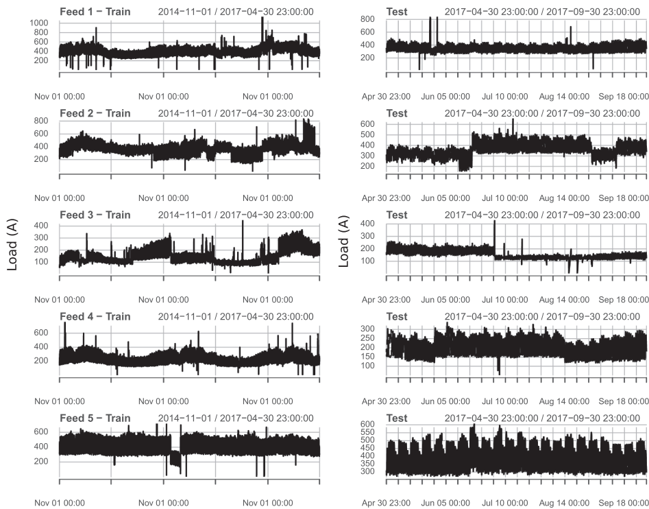
Fig. 8. Time plots for the training and testing raw datasets of “Feed 1” to “Feed 5”.
