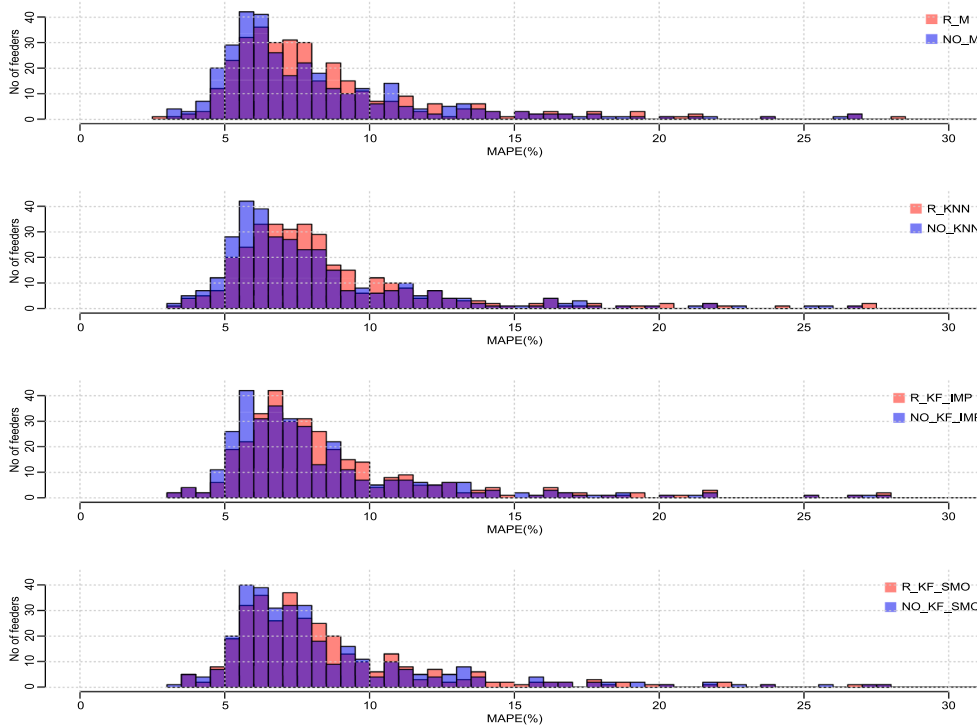
Fig. 11. Histograms of the MAPEs distributions for raw imputed data and fully cleansed data.
