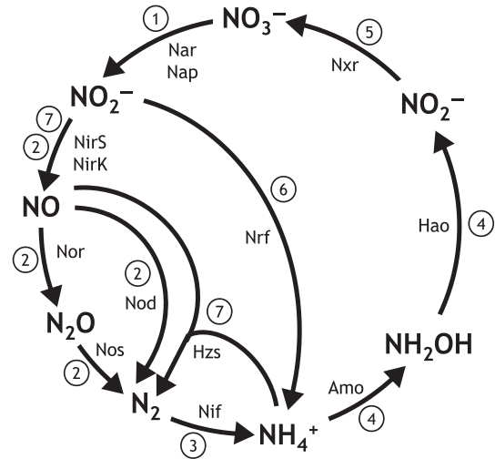
FIGURE 1 Biological N-cycle illustrating major metabolic processes (number coded) with associated known key enzymes. Number-coded metabolic processes: 1, nitrate reduction; 2, denitrification; 3, nitrogen fixation; 4, aerobic ammonia oxidation; 5, aerobic nitrite oxidation; 4+5, comammox; 6, dissimilatory nitrite reduction to ammonium (DNRA); 7, anaerobic ammonia oxidation. Nar/Nap, dissimilatory nitrate reductase; NirK/NirS, dissimilatory NO-forming nitrite reductase; Nor, nitric oxide reductase; Nod, nitric oxide dismutase; Nos, nitrous oxide reductase; Nif, nitrogenase; Amo, ammonia monooxygenase; Hao, hydroxylamine oxidoreductase; Nxr, nitrite:nitrate oxidoreductase; Nrf, dissimilatory ammonia-forming nitrite reductase; Hzs, hydrazine synthase
