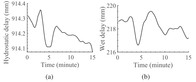
Fig. 4. Tropospheric delay time series for one location. (a) Hydrostatic delay. (b) Wet delay.
