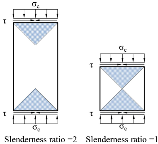
Fig. 10. Confined zones caused by frictional confinement [24].
