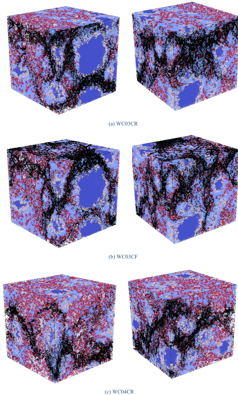
Fig. 8. Simulated crack pattern of cubic specimens at the failure stage (black-crack).
