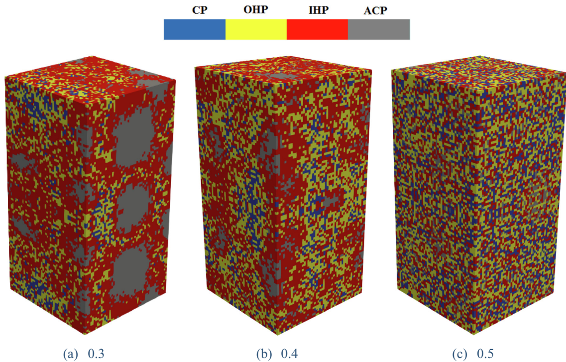
Fig. 2. HCP prismatic specimen ( 100\ \mu\text{m} \times 100\ \mu\text{m} \times 200\ \mu\text{m} ) with different w/c ratios (CP: capillary pore; IHP: inner hydration product; OHP: outer hydration product; ACP: anhydrous cement particle).
