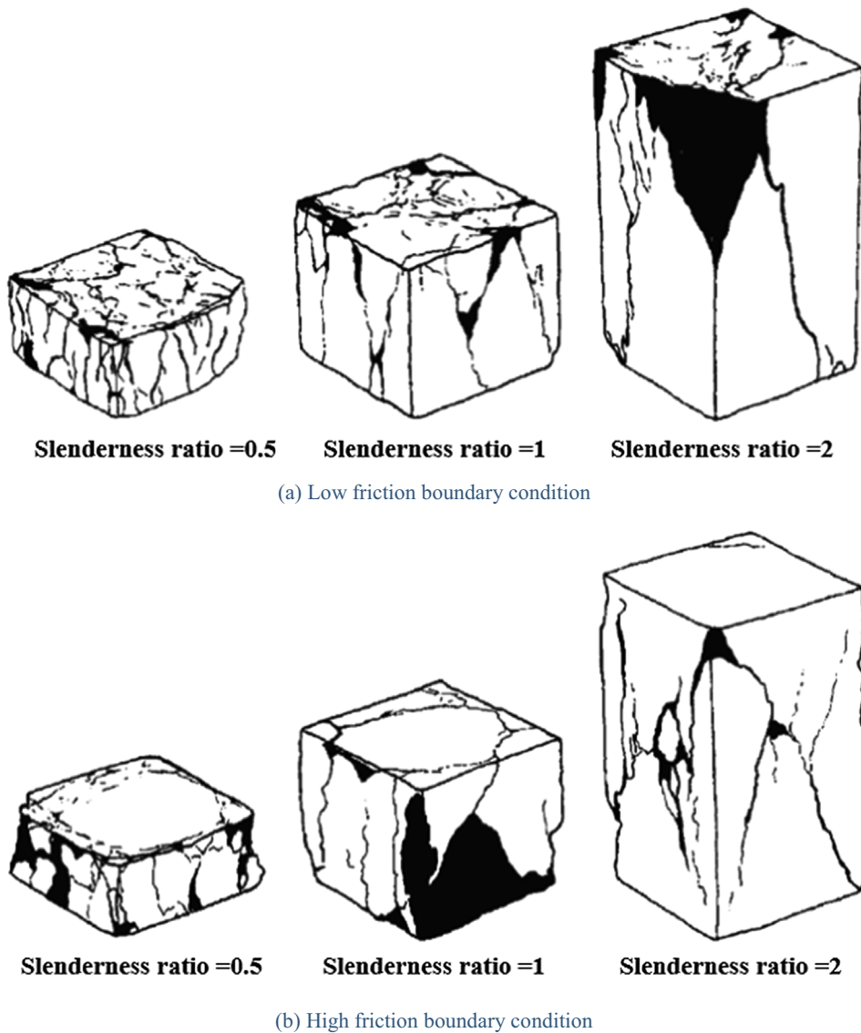
Fig. 11. Crack pattern of concrete specimens at the failure stage under compression [38].
