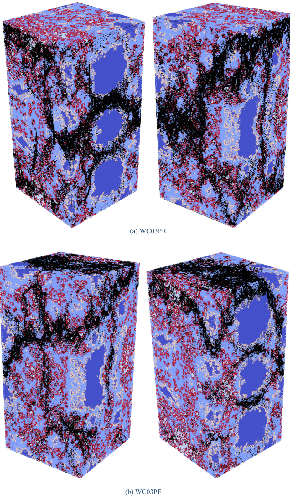
Fig. 9. Simulated crack pattern of prismatic specimens at the failure stage (black-crack).
