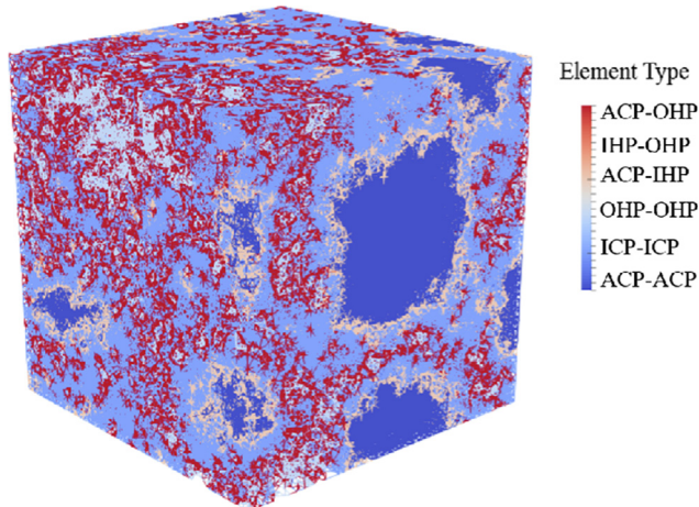
Fig. 4. Element type spatial distribution of cubic specimen with w/c ratio of 0.3.
