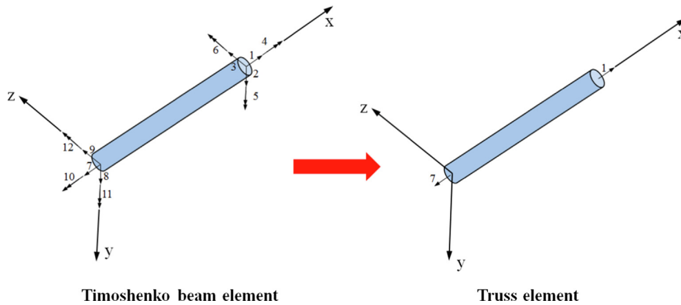
Fig. 5. Schematic view of the element degradation at first step [24].
