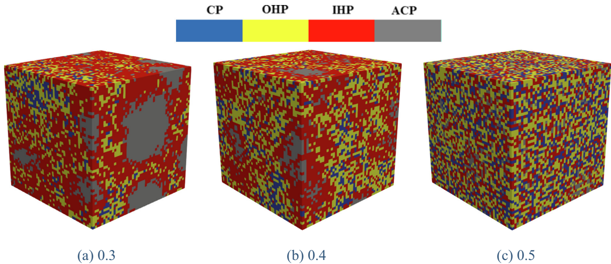
Fig. 1. HCP cubic specimens ( 100\ \mu\text{m} ) with various w/c ratio (CP: capillary pore; IHP: inner hydration product; OHP: outer hydration product; ACP: anhydrous cement particle).
