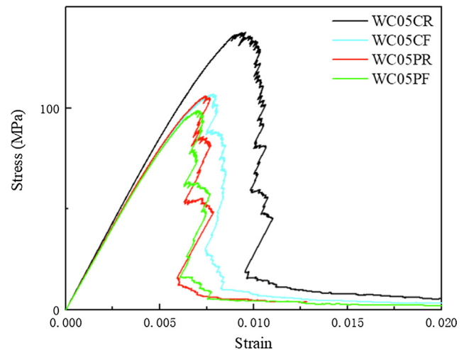
Fig. 7. Comparison of stress–strain response of specimens with w/c ratio of 0.5.
