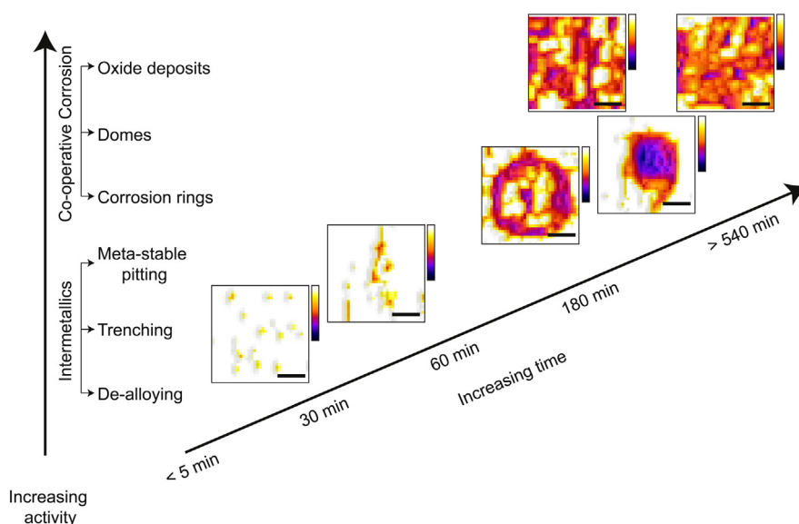
Fig. 6. Summary of the optical observations for the evolution of intermetallic and co-operative corrosion on the surface of AA2024-T3 in 0.05 M NaCl. Scale bars represent 50 \mu\text{m} . (For interpretation of the references to colour in this figure legend, the reader is referred to the Web version of this article.)
