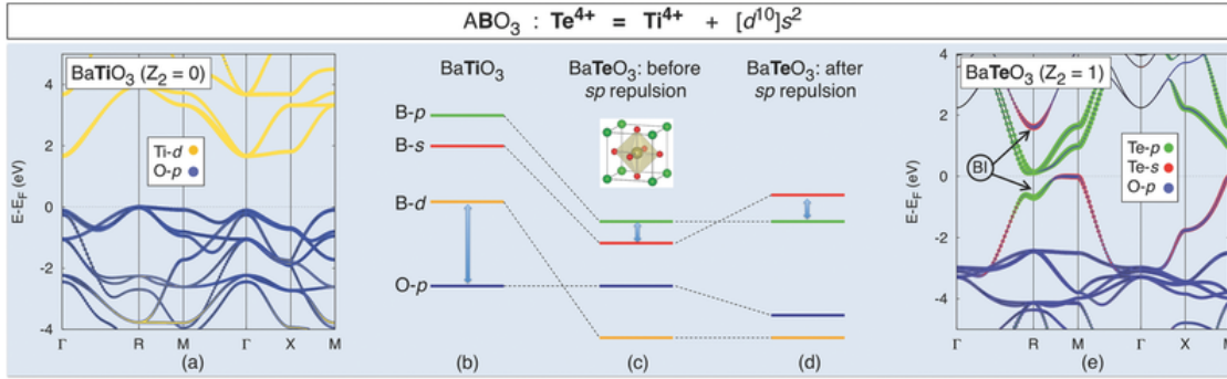
Figure 12. Concept of band inversion according to DFT calculations. (a),(b) The electronic structure of the band insulator ( Z_2=0 ) BaTiO 3 shows a gap between O-2p states and Ti-3d states (blue arrow); (c) replacing Ti with Te, the gap opens within the Te states, between the 5s and the 4p bands; (d),(e) considering the effect of sp repulsion, there is a band inversion (BI) and the formation of a topological insulator ( Z_2=1 ). This electronic structure is however strongly susceptible to atomic distortions that modify the cubic phase and suppress the band inversion. Reprinted from Ref. [81].
