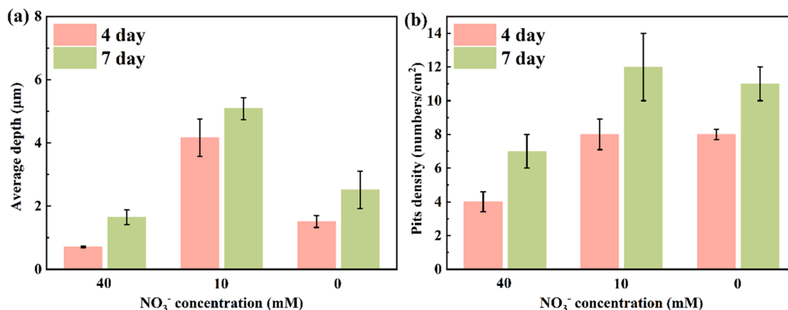
Fig. 3. (a) Average depth and (b) density of the corrosion pits on the stainless steel surfaces after 4 and 7 days of incubation in the media containing 40, 10 or 0 mM NO 3 - .
