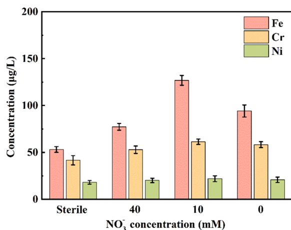
Fig. 4. ICP-MS results for the dissolved Fe, Cr and Ni in the sterile and WT inoculated media containing 40, 10 or 0 mM NO 3 - .
