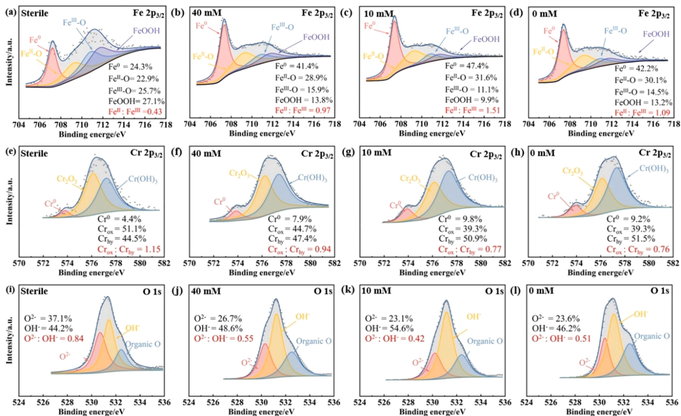
Fig. 5. High-resolution XPS spectra of Fe 2p 3/2 (a–d), Cr2p 3/2 (e–h) and O1s (i–l) for the samples surfaces after immersion in the sterile control and the WT inoculated media with 40, 10 or 0 mM NO 3 - after 7 days of immersion.
