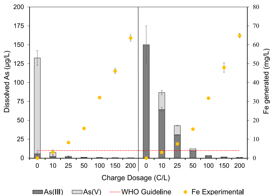
Fig. 5. Batch mode bio-FeEC (left) and conventional FeEC (right) treatment of 150 µg/L As(III) as a function of CD applied at 5 C/L/min CDR. The bio-FeEC experiments were conducted with the effluent of the biological anthracite layer; the conventional FeEC experiments are shown again in Figure S2 (right).
