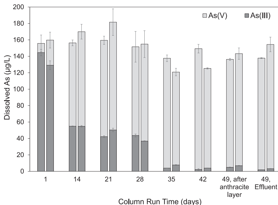
Fig. 3. As(III) and As(V) concentrations in the effluent of the duplicate biological filter columns during 49 days ripening with 150 ± 30 µg/L As(III) spiked tap water.
