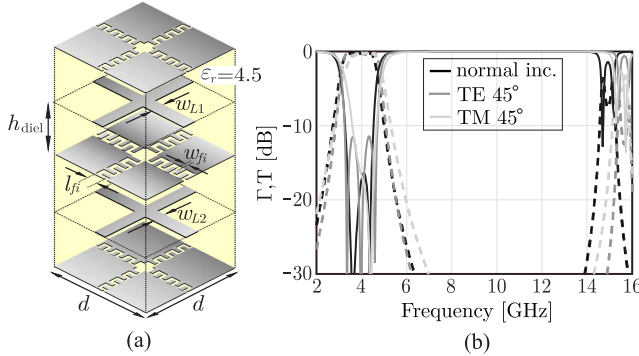
Fig. 2. (a) FSS unit cell realizing the equivalent circuit of Fig. 1(b) and (b) reflection (solid line) and transmission (dashed line) coefficients of the FSS for broadside, 45^\circ TE and TM oblique incidence.
