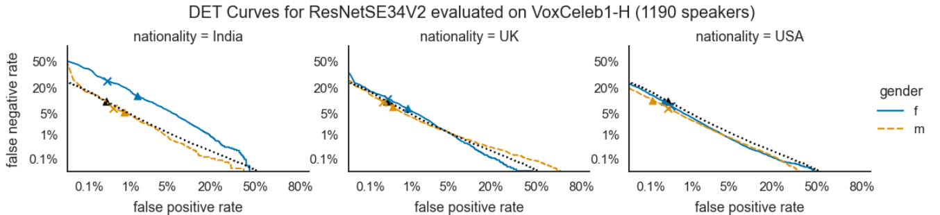
Figure 11: DET curves and thresholds for male and female speakers of Indian, UK and USA nationalities for ResNetSE34V2 evaluated on the VoxCeleb1-H test set.
