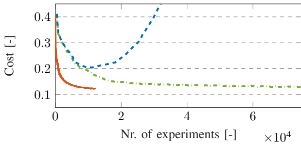
Fig. 4: The cost as a function of the number of experiments for a noisy non-symmetric 21 \times 21 system. Stochastic conjugate gradient descent ILC based on (23) (—) requires far fewer experiments than the implementation using (29) (---). Implementing the deterministic conjugate gradient (--) method in case of noisy system evaluations and gradient estimates leads to divergent behavior.
