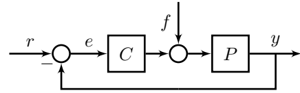
Fig. 1: Closed-loop system with reference r , error e and feedforward input f , for which J = P(I + CP)^{-1} is the process sensitivity of the closed-loop system.
