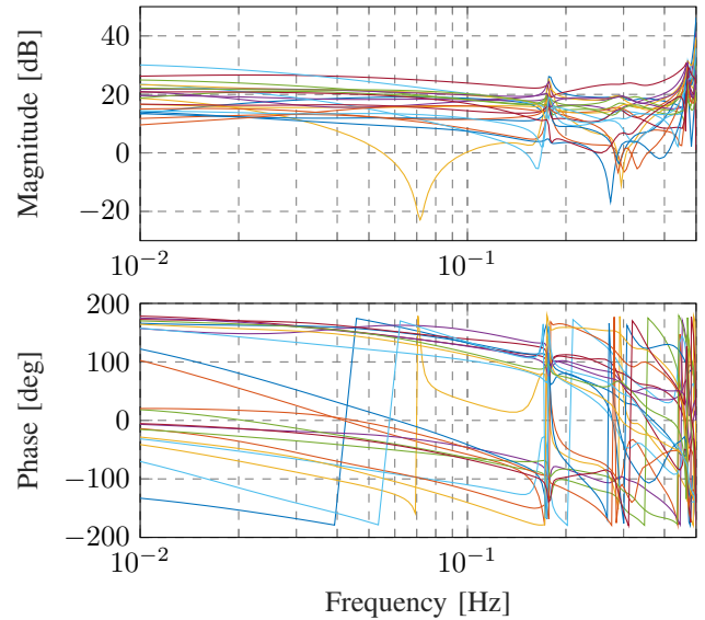
Fig. 2: Bode magnitude and phase plots of the last column of 21 subsystems of the random non-symmetric 21 \times 21 MIMO system used in the example.
