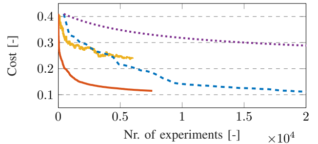
Fig. 3: The cost as a function of the number of experiments for a non-symmetric 21 \times 21 system. Four approaches are shown: the proposed stochastic conjugate gradient ILC method ( \rightarrow ), deterministic conjugate gradient ILC ( \dashrightarrow ), stochastic gradient descent ILC ( \dashrightarrow ) and deterministic gradient descent ILC ( \cdots ). Stochastic conjugate gradient descent ILC requires far fewer experiments than other approaches to reach the same cost.
