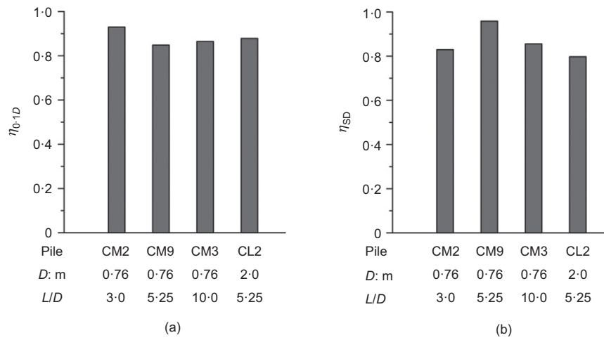
Fig. 12. Calculated accuracy metrics for the (a) full load–displacement curve and (b) small-displacement range
